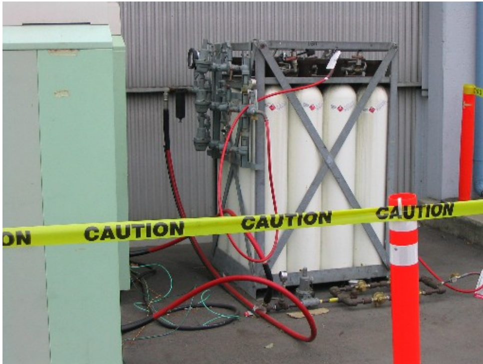
Figure 4 - Natural Gas Fuel Pod
