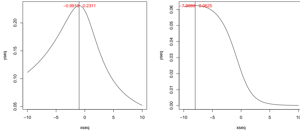
FIGURE 4. \delta for logistic at y = 1 (left) and y = 8 (right).
