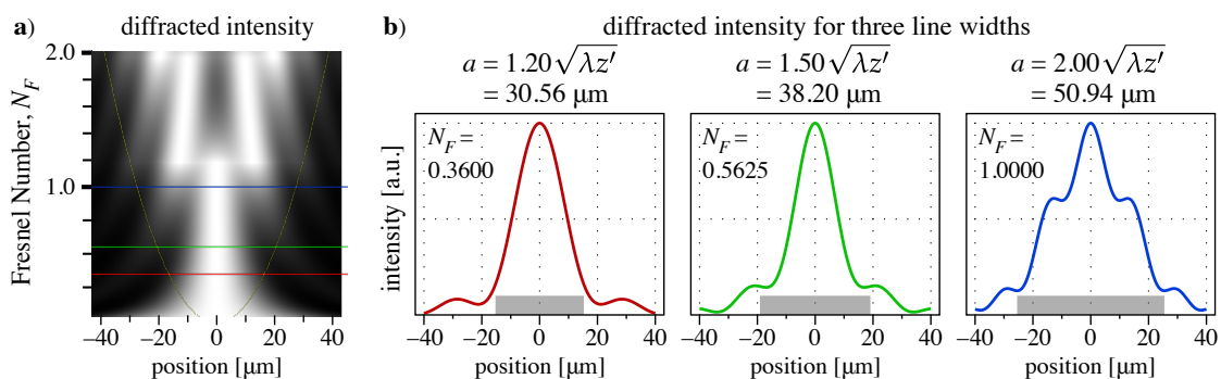
Figure 2. Diffracted intensity patterns from a range of isolated Hartmann-grid line widths calculated with respect to the Fresnel number, N_F = a^2/4\lambda z' , with fixed wavelength, \lambda = 2 nm, detector distance, z = 0.3 m, and incident beam radius, R = 4 m. Note that \sqrt{\lambda z'} = 25.469 \mu\text{m} . (a) Each row is calculated independently and normalized to its maximum value. Yellow curves show the line width, references to the horizontal axis. Red, green, and blue lines show the positions of three specific diffracted intensity calculations (b) extracted from the plot. Gray rectangles represent the line width in each case.
