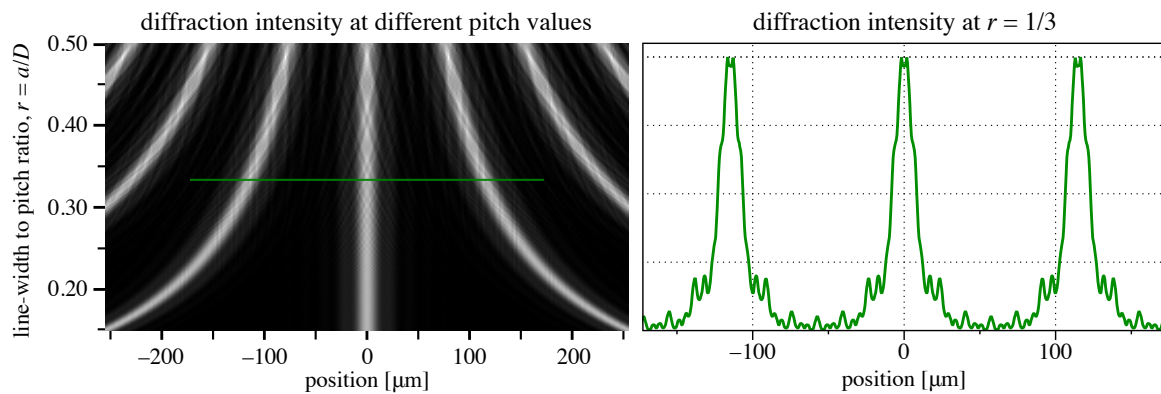
Figure 3. Coherent wave-propagation calculations of Hartmann grid diffraction intensity patterns as a function of the pitch, D . A constant line width, a = 38.203 \mu\text{m} , is maintained (Equation (8)). The plot on the right shows three periods of the pattern, calculated at r = 1/3 , extracted at the position of the green line.
