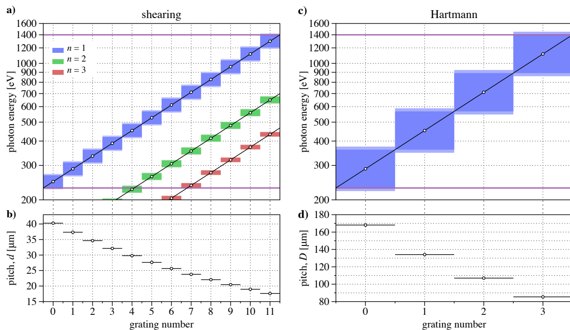
Figure 7. Design of shearing and Hartmann arrays spanning a 230 eV to 1400 eV energy range. (a) Counting 0 to 11, twelve gratings span the range with \beta = 0.1624 , using the first Talbot plane ( n = 1 ). Blue-colored regions show the individual gratings' operating energy range. The equivalent energy range is shown for the second and third Talbot planes in green and red. (b) Corresponding grating pitch values. (c) With \beta = 0.4351 , four Hartmann grids (Numbered 0 to 3) span the range. (d) Corresponding Hartmann grid pitch values.
