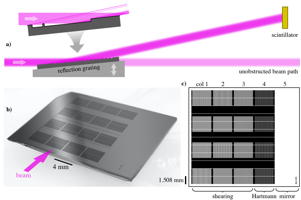
Figure 6. Illustration of the wavefront sensor grating array, its pattern, and use. (a) The narrow beam has a 2^\circ , glancing angle of incidence and a longitudinal footprint longer than the array, so the four patterns in a column are illuminated at once. The inset grating cross-section detail shows how light reflects from the top surface, yet all other light is blocked by the thin walls and etched pattern features. At low angles, the detection-plane scintillator may be upright or inclined. The pattern (c) is etched into a silicon wafer chip (b), which is approximately 28 mm wide. The pattern's five columns contain 12 shearing gratings (Columns 1–3), four Hartmann grids (Column 4), and an open mirror region (column 5).
