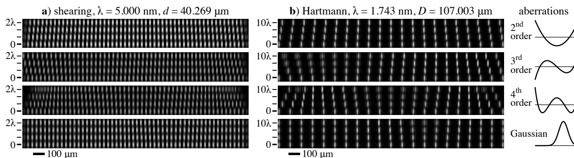
Figure 10. (a) Shearing and (b) Hartmann aberration modeling showing four different aberration types and varying amplitudes. Each row is a detail extracted from an intensity calculation performed for a single grating or grid on a 2 mm wide domain. The scale bars on the left show the uniformly-weighted aberration rms amplitudes for the polynomials and the peak height for the Gaussian cases.
