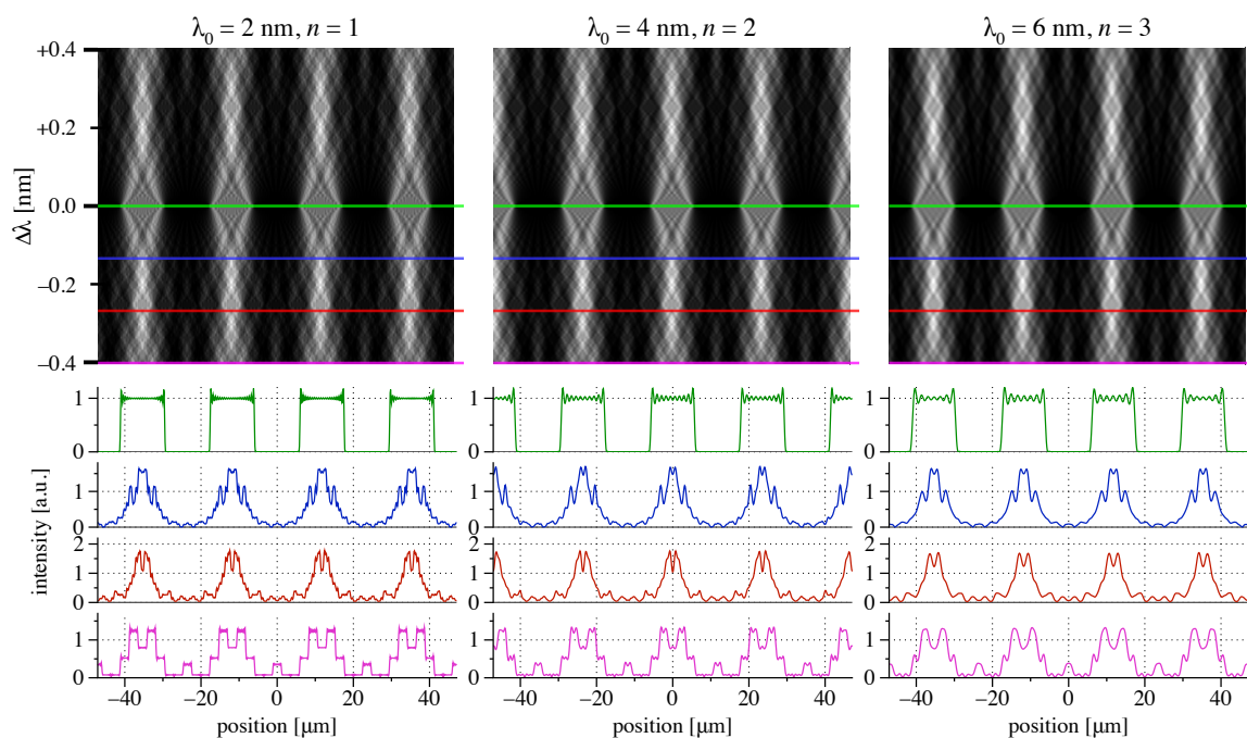
Figure 5. Coherent wave-propagation calculations of the detector-plane, central intensity region in shearing interferometry, for a 2, 4, and 6 nm wavelength, with a fixed geometry matching Figure 4a. Eighty, uniformly-illuminated grating lines are modeled in each case. Conditions match the first three Talbot planes, respectively. Each row is normalized for constant integrated power. Green lines indicate the Talbot condition. Blue, red, and magenta lines show wavelength shifts of -0.133 nm, -0.267 nm, and -0.400 nm, respectively. Corresponding intensity profiles are extracted from the wavelength offsets and plotted below.
