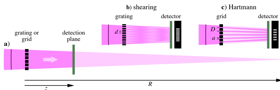
Figure 1. (a) Beam geometry used in the single-grating shearing interferometry and Hartmann wavefront. A converging (shown) or diverging beam, incident from the left, is transmitted by a shearing grating or Hartmann grid and propagates a distance z to the detection plane. The grating-to-focus distance is R (negative in the diverging-beam case). Inset details show (b) shearing geometry with grating pitch d and (c) Hartmann geometry with grid pitch D and opening width a .
