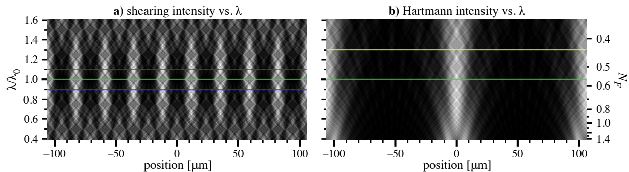
Figure 4. Coherent wave-propagation models of shearing and Hartmann detector-plane intensities for a range of wavelengths about \lambda_0 = 2 nm (green line), in a converging beam. Each row is normalized for constant integrated power. Pitch values are d = 25.469 \mu\text{m} for shearing and D = 114.609 \mu\text{m} for Hartmann with a = 38.203 \mu\text{m} . (a) Red and blue reference lines represent a \pm 10\% wavelength change. (b) Hartmann calculations show separation between neighboring beamlets. The yellow line marks a +30\% wavelength change, where \beta = 0.690 . The corresponding Fresnel number is shown at the right.
