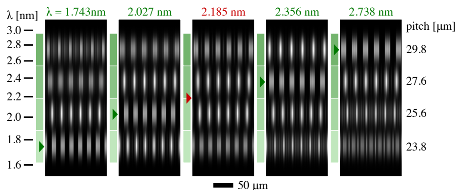
Figure 8. Modeled shearing detector-plane intensity patterns. The four gratings of Column 2 are illuminated with wavelengths shown above each detail. Grating pitch values are shown on the right. Square-wave intensity patterns are reproduced at the four design wavelengths (green markers), while the intermediate wavelength (red marker) shows that gratings from the two middle rows can both be used. The green colored rectangles align to the scale at the left and show the wavelength ranges over which each grating is designed to be used.
