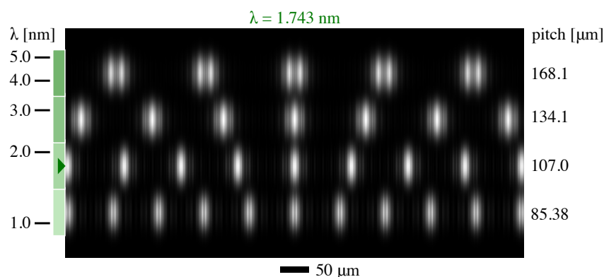
Figure 9. Hartmann detector-plane intensity pattern detail, calculated for the wavelength corresponding to the design of the second-lowest row (green marker). The beamlets in that row have a smooth intensity profile and minimal overlap. Green colored rectangles align to the scale at the left and show wavelength ranges over which each grid is designed to be used. We observe that the two grids designed for larger wavelengths project spots with a more prominent structure, while grids designed for smaller wavelengths show adjacent beamlet interference.
