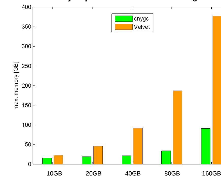
Cnygc (v0.4.1429) and Velvet (v1.0.19) memory requirements cow rumen metagenome
