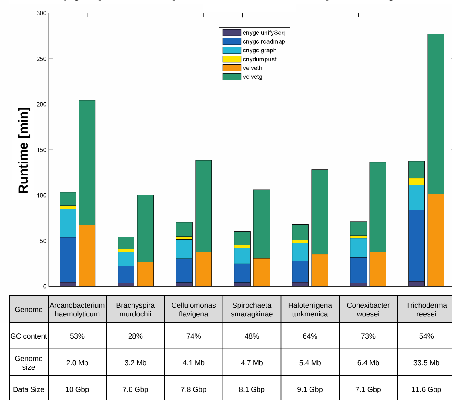
Cnygc (v0.2.1208) and Velvet (v1.0.18) running times
