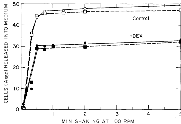
FIGURE 2 Release of HTC cells from glass as a function of time of shaking at 100 rpm. HTC cells were collected in log phase of growth and resuspended in induction medium at 350,000/\text{ml} . 15-ml aliquots of cell suspension ( 5.0 units of A_{650} ) were incubated without shaking at 37^\circ\text{C} in the presence and absence of 10^{-7}\text{ M} Dex. After 6 hr of incubation, vessels were rotated at 100 rpm and 1.5-ml aliquots of cell suspension were removed at various intervals for A_{650} measurements. The total number of cells (total amount of A_{650} ) released at each interval is shown for duplicate experiments.
