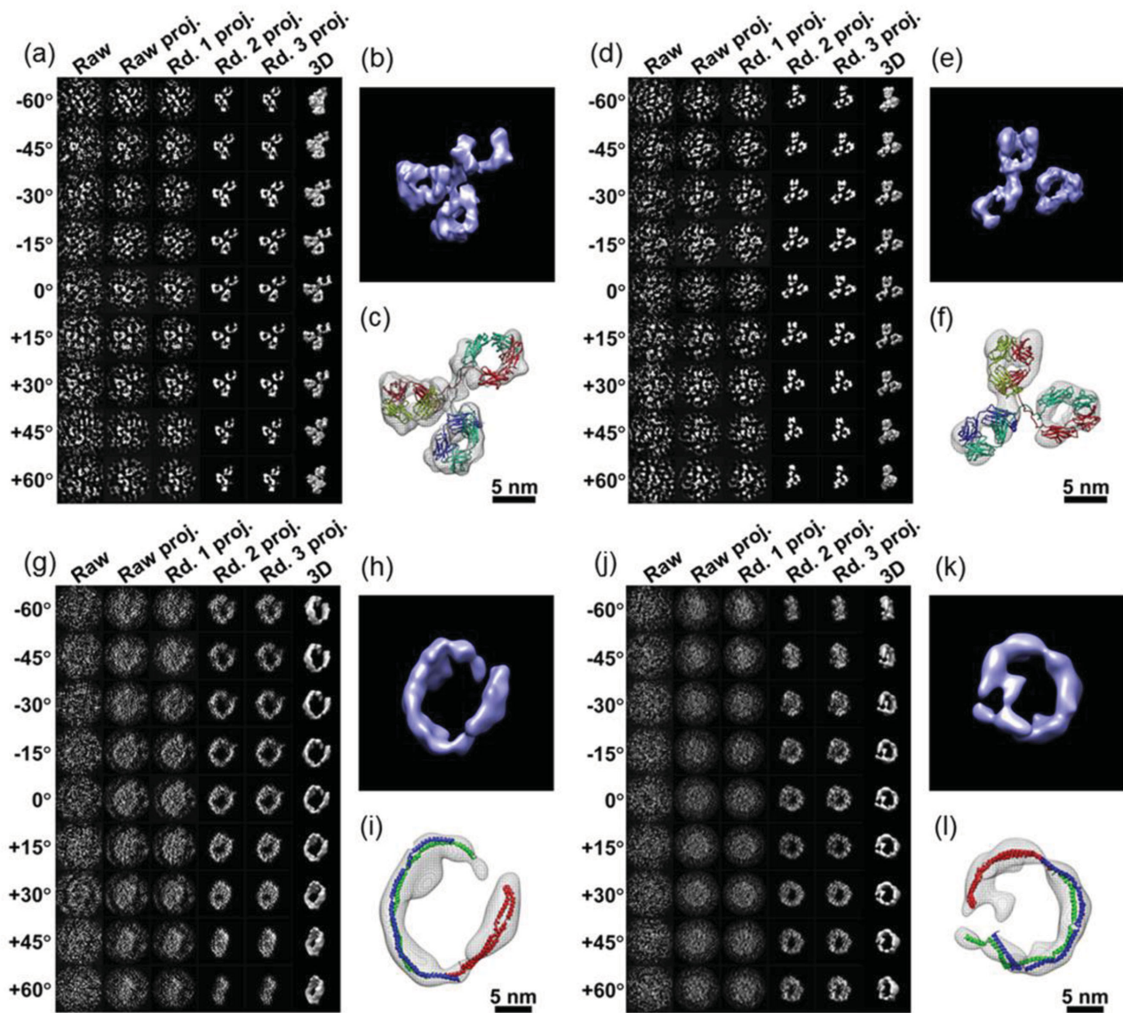
Figure 16. IPET 3D reconstructions of two IgG antibody particles by negative-staining ET and two HDL particles by cryo-EM. a) Nine representative images from a tilt series of a single-instance IgG antibody by negative-staining (NS) ET displayed in the left-most column. The IPET method obtains the 3D model of an individual protein via an iterative refinement processes. b) The iso-surface of the final 3D reconstruction of an individual antibody particle. c) Flexible docking of the structure obtained by X-ray crystallography (PDB entry 1IGT) into each domain of IgG shows a good fit. d–f) Another example of an individual IgG antibody particle. g–i) A 17 nm nascent HDL particle embedded in ice, imaged by cryo-EM tomography and reconstructed by the IPET method. The high-density portion corresponds to the protein component, primarily consisting of apolipoprotein A-I (apoA-I), forms a discoidal shape (a ring shape). j–l) Another example of a 17 nm nascent HDL particle by cryo-EM tomography. The 3D reconstruction showed the similar structural feature to the first HDL particle. Our cryoET reconstructions are consistent with other cryoEM observations. a–l) Reproduced with permission. [38] Copyright 2012, The Authors, Published by PLoS ONE.
