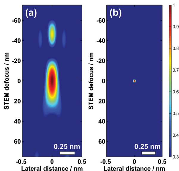
Figure 6. A comparison between the lateral and depth resolution of focused STEM beams for: a) an uncorrected 200 kV FEI Tecnai STEM and b) an aberration-corrected 300 kV FEI Titan. The intensity scale shows low intensity for blue and high intensity for red. The drastically reduced probe dimensions (both lateral and depth) of aberration-corrected STEM have important implications for electron tomography because the entire object may not be in focus.
