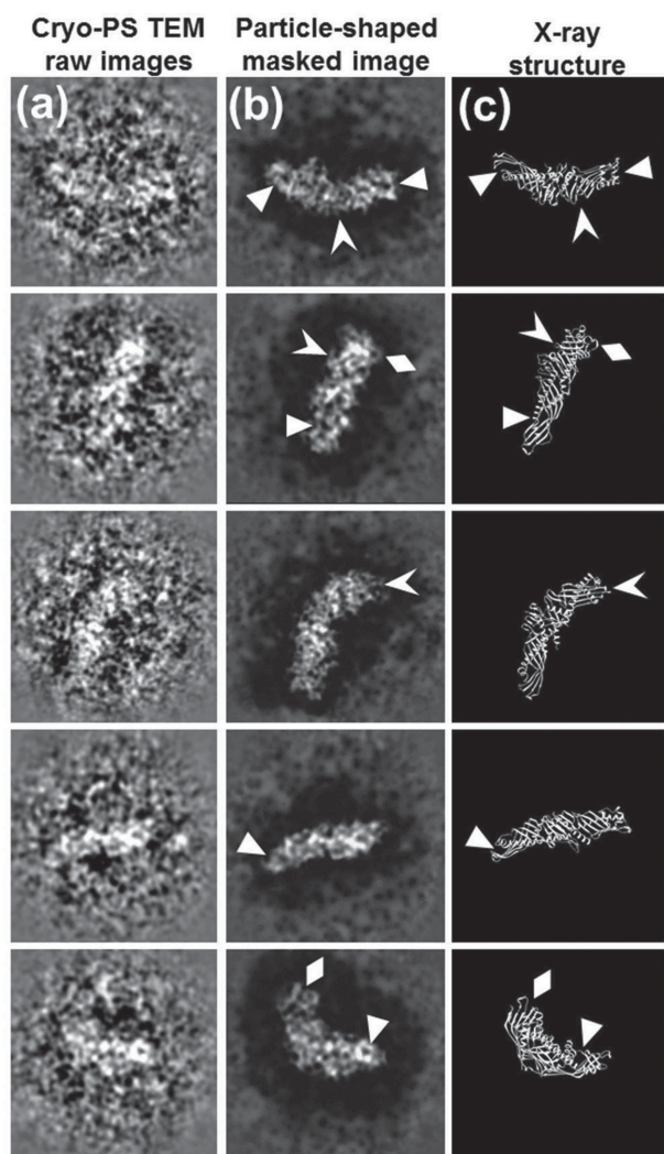
Figure 13. Images of a small and asymmetric protein CETP (53 kDa) imaged using cryo-positive staining (cryo-PS) showing high-resolution details. a) Five representative images of CETP particles prepared by cryo-positive staining (with reversed contrast and a circular-shaped soft mask). b) By applying particle-shaped soft masks on each particle image, the masked images are compared with (c) the structure of CETP (obtained by X-ray crystallography and shown in ribbon structure) at similar viewing angles. Similar structural features are marked by arrows. Reproduced with permission. [162] Copyright 2012, rights managed by Nature Publishing Group.
