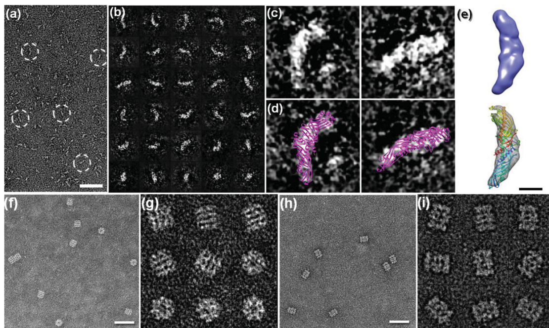
Figure 11. TEM images of proteins with known structure using OpNS. a) Survey view of a small and asymmetric protein, 53 kDa CETP (dashed circles) by OpNS. b) 30 representative images of CETP particles. c) Two representative images of CETP particles with particle orientation identified by their tapered tip end (N-terminal \beta -barrel domain) and globular tip end (C-terminal \beta -barrel domain), d) which is consistent with the CETP structure, obtained from X-ray crystallography (PDB: 2OBD), in size and shape. e) The high-contrast images were used to reconstruct a 3D volume at 1.4 nm resolution. f) Survey view of another protein with known structure, GroEL, and g) 9 representative particle images prepared by OpNS. h) Survey view of a third protein with known structure, proteasome, and i) 9 representative particle images prepared by OpNS. Scale bars: a) 50 nm; e) 3 nm; f) and h) 50 nm. a–e) Reproduced with permission. [162] Copyright 2012, rights managed by Nature Publishing Group; f–i) Reproduced with permission. [181] Copyright 2014, The Authors, published by Journal of Visualized Experiments (JoVE).
