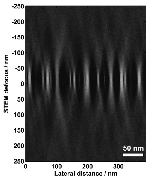
Figure 7. An example of the limited 3D-reconstruction resolution achieved using only defocus in aberration-corrected HAADF-STEM. The image is a cross-section through a set of images at different defocus values of ca. 5 nm diameter gold nanoparticles on a carbon substrate using an aberration-corrected STEM at 300 kV with a 30 mrad semi-convergence angle. The depth of focus is estimated to be ca. 6 nm. The lateral extent of the nanoparticles (horizontal axis) is well defined and the thickness (vertical axis) is highly elongated due to signal from the focused and unfocused parts of electron beam.
