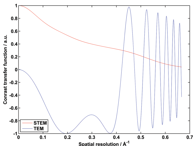
Figure 5. A comparison of the CTF for STEM (red) and TEM (blue). The phase portion of the CTF for TEM is plotted at Scherzer defocus (maximum resolution). STEM shows a monotonically decreasing function for increasing spatial frequency. TEM has low information transfer at low frequencies ( <0.1 \text{ \AA}^{-1} ). However, TEM provides relatively high transfer compared to STEM near the maximum linear resolution at the first zero crossing of the TEM CTF (ca. 0.32 \text{ \AA}^{-1} ). The oscillatory nature of the TEM transfer function above the first zero crossing complicates analysis of TEM images at high resolution especially for crystalline materials. Importantly, TEM provides relatively high SNR for a given dose compared to STEM, which are not considered in this comparison.
