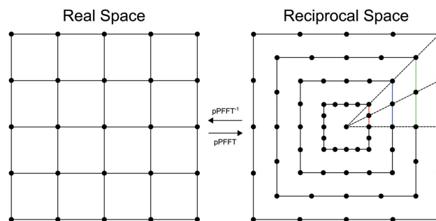
Figure 8. Unlike normal tilting ET, data acquisition for equally sloped tomography (EST) uses specific tilt-angles that directly map into reciprocal space on a grid of concentric squares without interpolation. The pPFFT -1 accurately calculates the density map in real space on a rectangular grid. For clarity, the diagram shows a small set of 4 tilt angles with 22.5° between tilt images. Notice the colored vertical lines in reciprocal space, which mark equal slope increments between projections. Since projections acquired using EST perfectly map to reciprocal space, iterative calculations that transform the data between real and reciprocal space (used to improve the reconstruction resolution) are exact and produce no artifacts.
