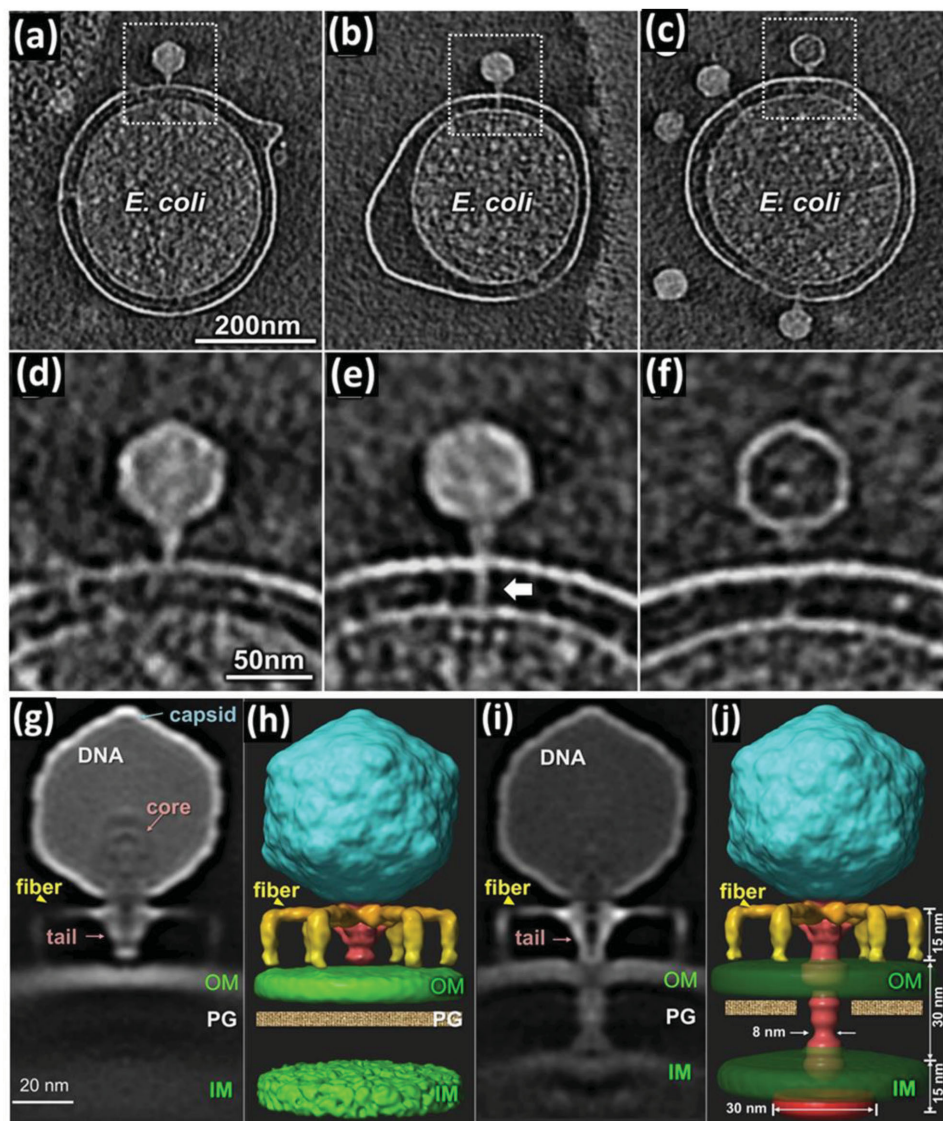
Figure 15. 3D reconstruction of bacteriophage T7 virion infection of Escherichia coli minicells by cryo-electron tomography. a–c) Three selected sections of large-volume 3D reconstructions of T7 infection of E. coli . d–f) Higher-magnification views of the sections of the subvolumes. g,h) A central slice and 3D surface view of a selected sub-volume average from 3352 virions. i,j) A central slice and 3D surface view of another selected sub-volume average from 1886 virions. Reproduced with permission. [241] Copyright 2013, American Association for the Advancement of Science (AAAS).
