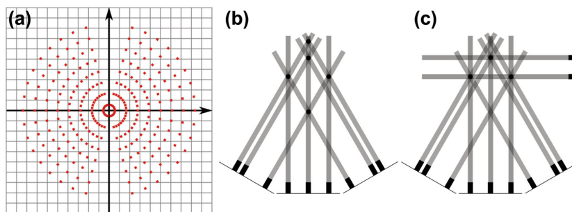
Figure 4. a) The mismatch between information sampled by a 17-image tilt series with equal angular increments (red dots) and a square Cartesian grid. The interpolation method used to combine this data can strongly influence the final reconstruction. Radon back-projection is used to avoid interpolation in space interpolation. b) A simplified example of Radon back-projection for a set of 3 low-tilt projections producing 5 possible object locations (black dots). c) The addition of a high-tilt projection uniquely defines the existence and location of only 3 objects.
