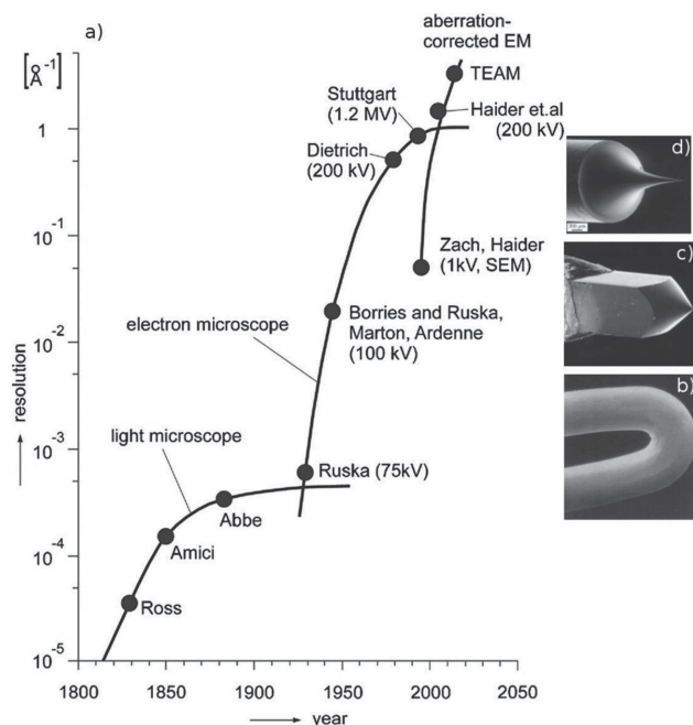
Figure 1. A schematic diagram of the historical resolution of visible light microscopes and transmission electron microscopes. a) The left panel shows a time line for the improvement of the resolution of microscopes versus the year of development. Reproduced with permission. [6] Copyright 2009, Oxford University Press. b–d) Three different types of TEM electron sources: a W filament, a LaB 6 filament, and an FEG. b) Reproduced with permission. [7] Copyright 1991, Springer; c, d) Reproduced with permission. [8] Copyright 2009, Springer.
