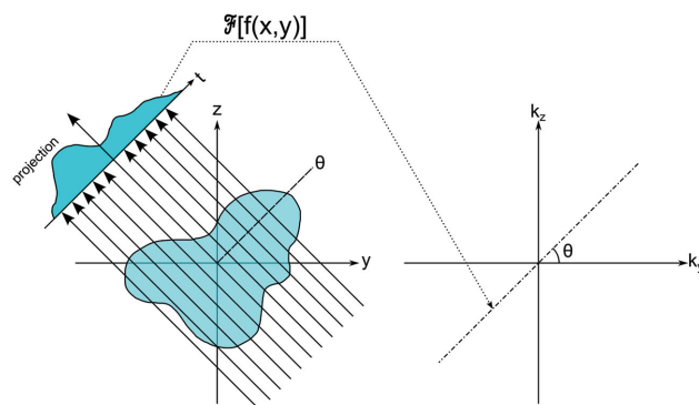
Figure 2. A diagram of the mathematical concept of the projection theorem in 2D (directly extendible to 3D). A projection of a 2D object in real space is reduced to a 1D measurement of the projected density. The Fourier transform of the 1D projection is equivalent to a central section at the original projection direction through the object's full Fourier transform.
