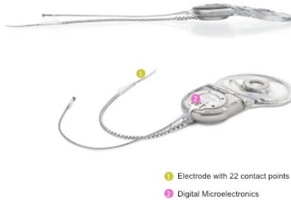
Fig. 39 MED-EL Cochlear Implant Electrode 57
