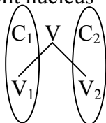
(3.34) Split nucleus
