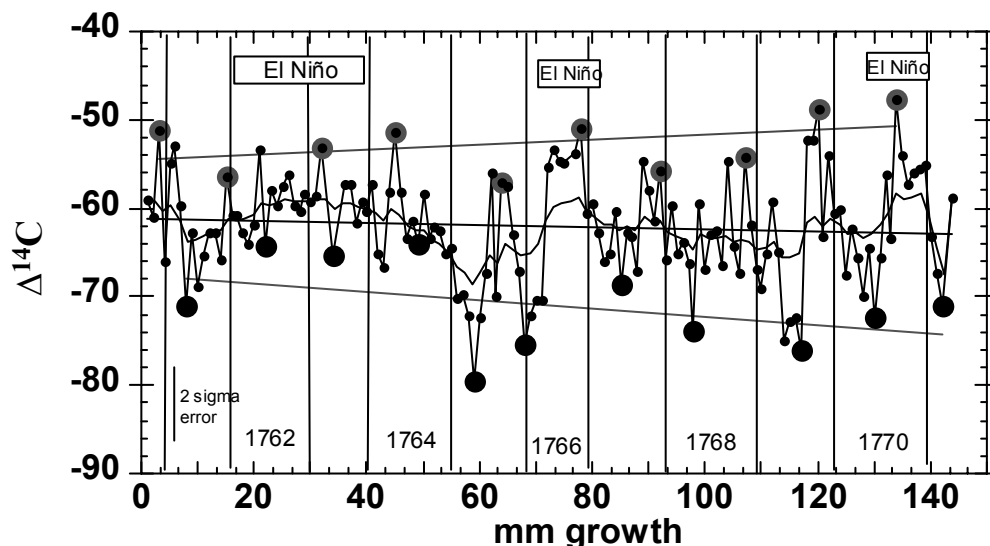
Figure 1 \Delta^{14}\text{C} measurements of monthly coral bands from Urquina Bay, Galapagos, during the period 1760 to 1771. The uncertainty of the age assignments in this age range is \pm 6 yr. Duplicate analyses of separate aliquots from the same coral sample and splits of the same \text{CO}_2 were averaged to a single point. Large grey points represent the highest \Delta^{14}\text{C} values for each year (lowest upwelling) and large black points represent the lowest \Delta^{14}\text{C} values for each year (most intense upwelling). Vertical lines mark the base of the high-density bands, which are generally formed when upwelling is low. Horizontal lines (grey) are the least-squares fits of the high and low ^{14}\text{C} values, and that (black) for all of the monthly results. The smoothed line of the monthly data is obtained using a Stineman function, which suggests that El Niño events occurred during 1762–63 and possibly 1766.
