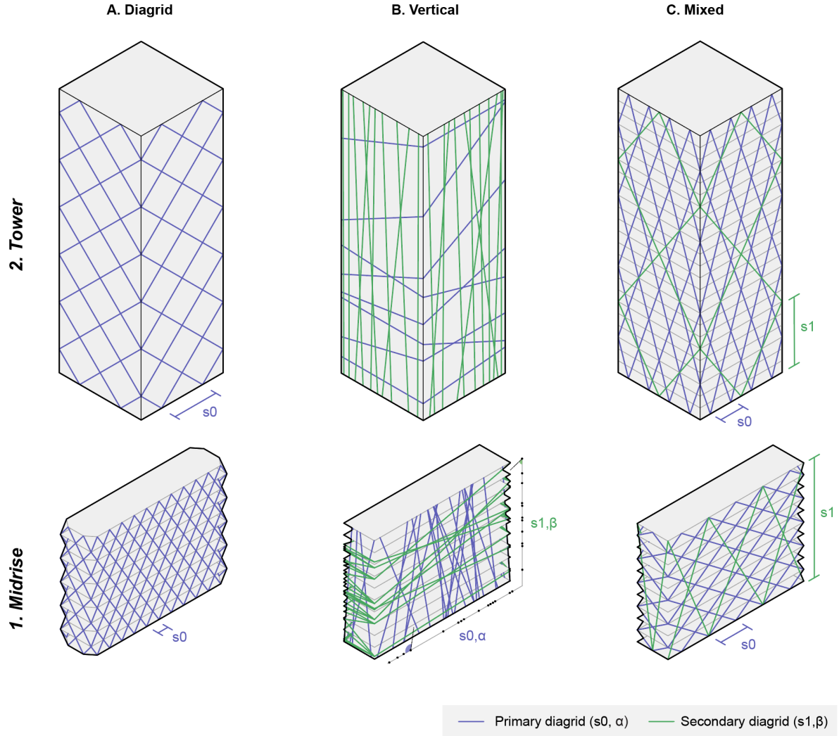
Figure 4: Geometric definition with floors and beams of a single diagrid (A.) with variable spacing ( s_0 ). Vertical scattering (B.) with two overlaid diagrids with variable beam angle ( \alpha, \beta ) and variable spacing ( s_0, s_1 ) and mixed scattering (C.) with two overlaid diagrids with variable spacing ( s_0, s_1 ).
