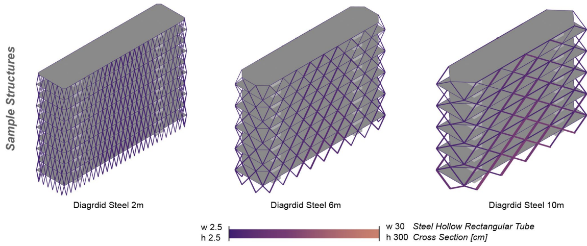
Figure 7: Three sample structures in steel with node spacing ( s ) of 2m, 6m and 10m. Element members are colored according to the largest and smallest member to display the mass distribution.
