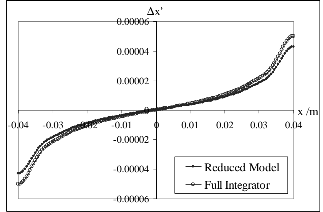
Figure 2: Horizontal momentum kick from one period of the NLC main damping rings wiggler.
