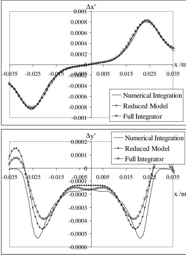
Figure 1: Horizontal and vertical kicks from one period of the SPEAR 2 BL11 wiggler.
