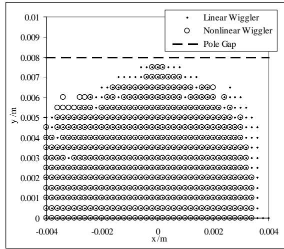
Figure 3: Aperture with the linear and nonlinear wiggler models, and vertical collimation in the wiggler.
