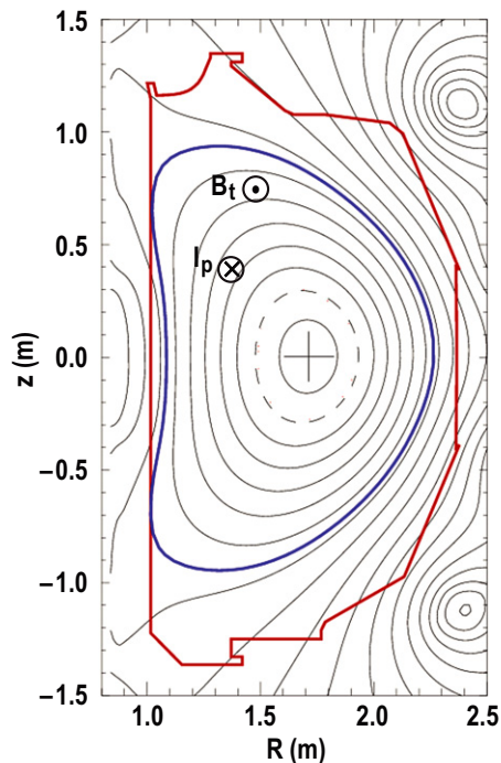
Figure 1. Poloidal cross-section of DIII-D for shot 141182. The thin contours are surfaces of constant magnetic flux; the dashed contour is the q = 1 surface; the inner thick contour (bean shape) is the last closed flux surface; the outer thick contour indicates the wall of the vessel.
