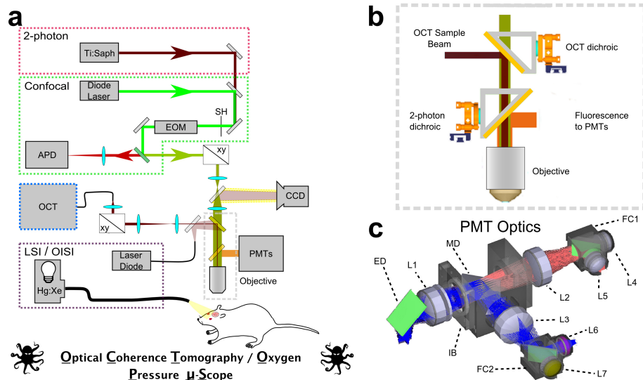
Fig. 1. (a). Schematic featuring primary components of the custom multimodal optical microscope. EOM- electro-optic modulator, SH- shutter, APD- avalanche photodiode, xy-galvanometer scanners, Hg:Xe- arc lamp. (b) Magnified region of schematic illustrating how the TPM/confocal scanning beam path and OCT beam path are coupled together and how emitted fluorescence is separated. OCT and TPM/confocal modules were designed with separate scanning arms and their probing optical beams were coupled into the same microscope objective by a movable dichroic mirror. (c) Detailed model of detector array for TPM fluorescence. Some specifications ED: Epi dichroic after objective (FF735-Di01-25x36, Semrock Inc), IB: Infrared blocker (FF01-750/SP-50, Semrock Inc), MD: main dichroic mirror (t560lpxr-35x52, Chroma Technology Corp), FC1: Filter Cube 1 (dichroic mirror: t640lpxr; channel 1 emission filter: hq680-60m-TPM; channel 2 emission filter: et595/50m-TPM, Chroma Technology Corp), FC2: Filter Cube 2 (dichroic mirror: FF495-Di02-25x36; channel 3 emission filter: FF01-525/50-25; channel 4 emission filter: FF01-460/60-25, Semrock Inc), L1-L3: Lenses 1-3: 50 mm diameter; FL = 81 mm (026-1450, OptoSigma Corporation), L4-L7: Lenses 4-7: 25.4 mm diameter, FL = 19 mm (KBX043, Newport).
