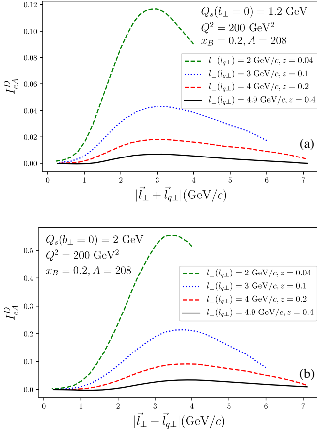
FIG. 11. The nuclear modification factor for the dijet spectrum from double scattering I_{eA}^D(l_{\perp}, l_{q\perp}, \Delta\phi, z) as a function of the azimuthal angle \Delta\phi or the transverse momentum imbalance |\vec{l}_{\perp} + \vec{l}_{q\perp}| in e + \text{Pb} DIS for different dijet kinematics and (a) Q_s(0_{\perp}) = 1.2 GeV and (b) Q_s(0_{\perp}) = 2 GeV.
