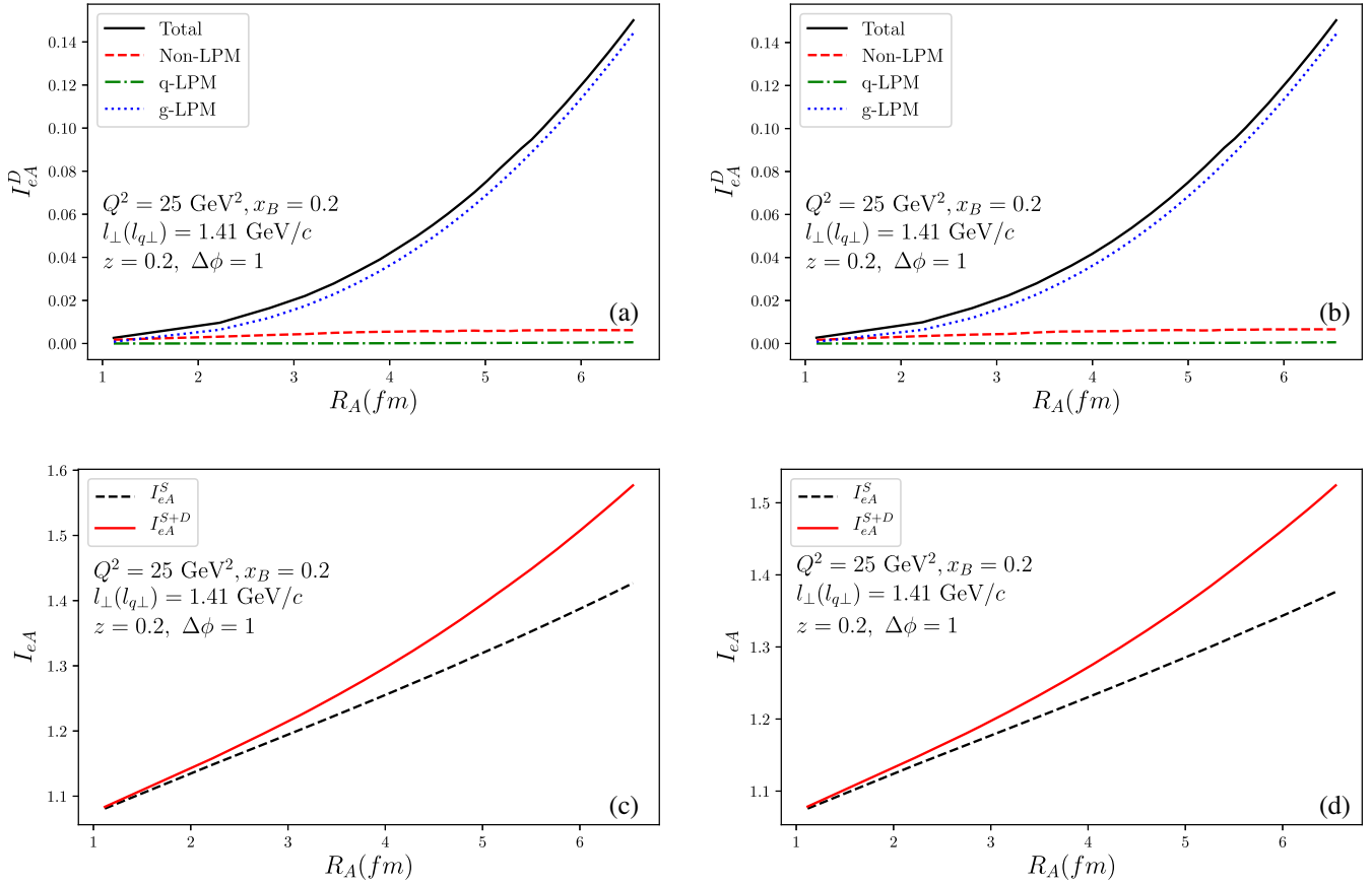
FIG. 25. The nuclear-size R_A dependence of the nuclear modification factor from double scattering I_{eA}^D(l_{\perp}, l_{q\perp}, \Delta\phi, z) (a) with (b) and without (b) constraint x_G > x_A , the nuclear modification factor I_{eA}^{S+D}(l_{\perp}, l_{q\perp}, \Delta\phi, z) with (solid) and without (dashed) double scattering I_{eA}^S(l_{\perp}, l_{q\perp}, \Delta\phi, z) without (c) and with (d) the constraint x_G > x_A in e + \text{Pb} DIS.
