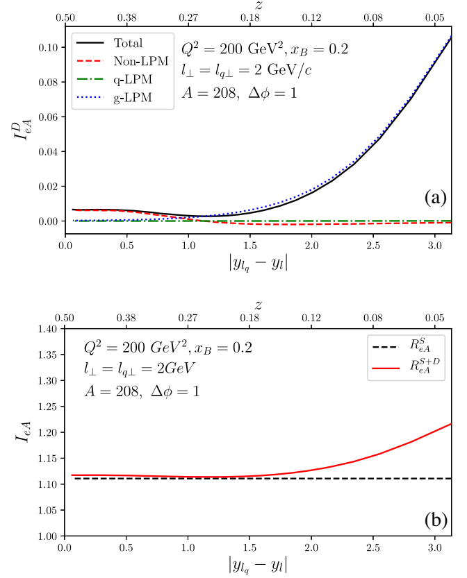
FIG. 12. The rapidity gap |y_{l_q} - y_l| or momentum fraction z dependence of (a) the nuclear modification factor from double scattering I_{eA}^D(l_{\perp}, l_{q\perp}, \Delta\phi, z) (b) the nuclear modification factor with (solid) R_{eA}^{S+D}(l_{\perp}, l_{q\perp}, \Delta\phi, z) and without (dashed) double scattering R_{eA}^S(l_{\perp}, l_{q\perp}, \Delta\phi, z) in e + \text{Pb} DIS.
