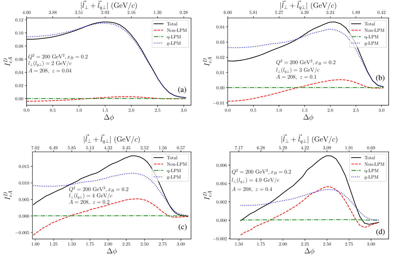
FIG. 9. The nuclear modification factor I_{eA}^D(l_{\perp}, l_{q\perp} = l_{\perp}, \Delta\phi, z) for the dijet cross section from double scattering as a function of the azimuthal angle \Delta\phi or the transverse momentum imbalance |\vec{l}_{\perp} + \vec{l}_{q\perp}| in e + \text{Pb} DIS with x_B = 0.2 and Q^2 = 200 \text{ GeV}^2 for (a) [z, l_{\perp}(\text{GeV}/c)] = [0.04, 2] , (b) [0.1, 3] , (c) [0.2, 4] and (d) [0.4, 4.9] .
