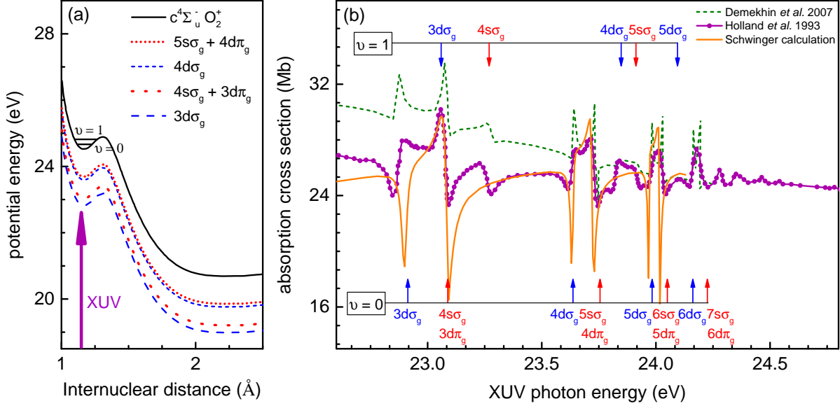
FIG. 1. (Color online) (a) Schematic potential energy diagram of O 2 . Black curve is the excited ionic c-state ( c^4\Sigma_u^- ). Blue dashed and red dotted curves are Rydberg series of neutral superexcited nd and ns states, respectively. Each state supports two vibrational levels. (b) (Purple line) Synchrotron measurement of photoabsorption cross section from [31]. Features associated with various electronic states and their vibrational levels ( \nu=0 at bottom and \nu=1 at top) are labeled. (Green dash line) Theoretical photoabsorption cross section from [32]. (Orange solid curve) Multichannel photoabsorption cross section that we obtained using Schwinger variational calculation.
