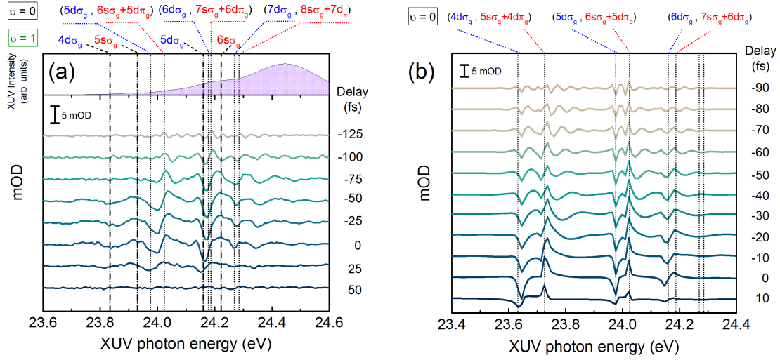
FIG. 3. (Color online) (a) Experimental transient absorption spectra at certain representative time delays. The scale bar represents 5 mOD change. Experimental XUV spectrum is also shown at the top. Negative time delay implies XUV arrives at the target earlier than NIR pulse. All nd\sigma_g ( ns\sigma_g + nd\pi_g ) states show negative (positive) OD at resonance, corresponding to less (more) absorption compared to continua absorption spectrum. (b) The MCTDHF calculations of the transient absorption spectra at few time delays.
