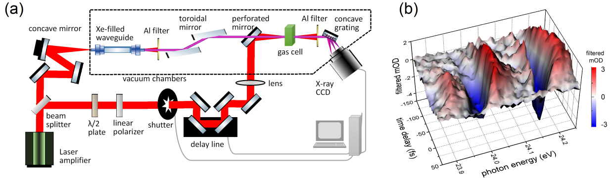
FIG. 2. (Color online) (a) Experimental set up for XUV transient absorption studies in neutral superexcited states of O_2 . (b) Experimentally measured transient absorption spectrogram in O_2 .
