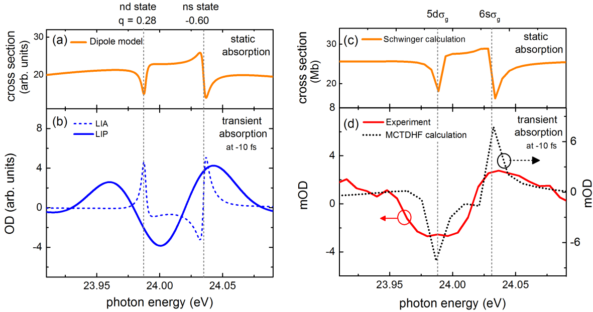
FIG. 7. (Color online) Modeling of transient absorption line shapes resulting from the NIR perturbation. (a) Simulated static absorption profile that mimics the 5d and 6s state line shapes and the corresponding Fano q parameters. (b) Transient absorption spectra obtained when NIR perturbation is modeled as laser induced phase (LIP) and laser induced attenuation (LIA). (c) Calculated static absorption spectrum for 5d and 6s states based on Schwinger variational approach from Fig 1(b) for comparison. (d) Experimentally measured transient absorption spectrum (solid red line), and MCTDHF calculated transient absorption spectrum (dashed black line) from Fig 3(b) for comparison.
