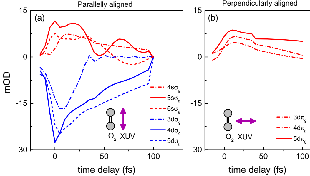
FIG. 8. (Color online) Transient absorption line-outs calculated using MCTDHF method for molecules (a) aligned parallel to XUV field polarization, and (b) perpendicularly to XUV field polarization, plotted at the energies corresponding to several resonances. Note that the NIR field polarization is always parallel to the XUV field polarization.
