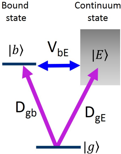
FIG. 6. (Color online) Three level model system showing a ground state |g\rangle , an excited bound state |b\rangle , and a continuum state |E\rangle , along with dipole couplings D_{gb} , D_{gE} , and interaction term V_{bE} .
