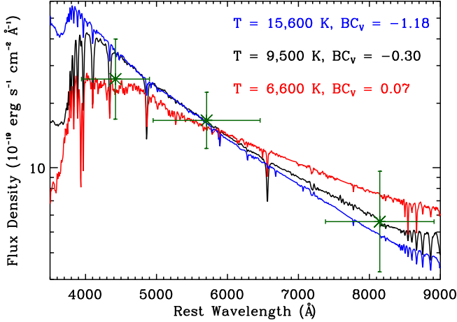
Figure 3. HST archival photometry from the SN 2016gkg progenitor star. The wavelength uncertainty of each point represents the width of the corresponding WPC2 filter. Each point has been corrected for extinction and the recessional velocity of NGC 613 has been removed from the effective wavelength. Overplotted are the best-fit (black) and \Delta\chi^2/\chi_{\min}^2 = 1 (red/blue) stellar spectra obtained from Pickles (1998). We indicate the temperature and bolometric correction of each stellar spectrum in the upper-right of the panel.
