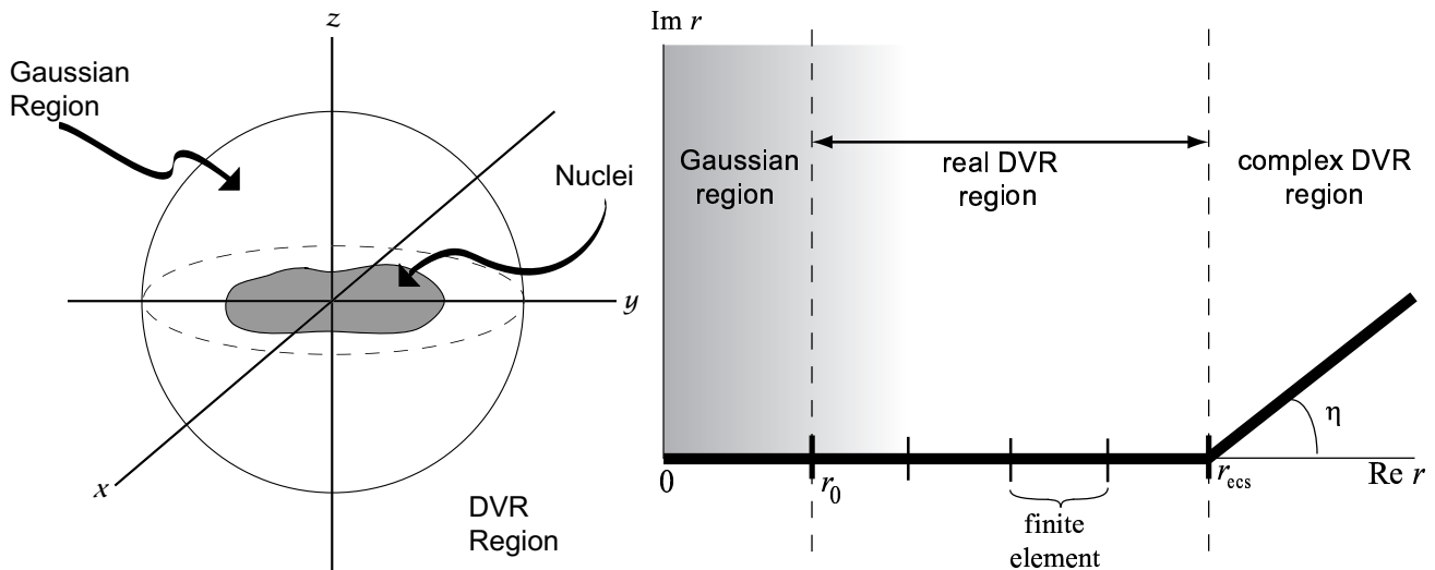
FIG. 1: Description of areas of physical space where different basis representations of electronic coordinates are best suited. In a mixed-basis composed of Gaussians and DVR functions, a radial interface r_0 specifies the linkage between the two constituent bases.
