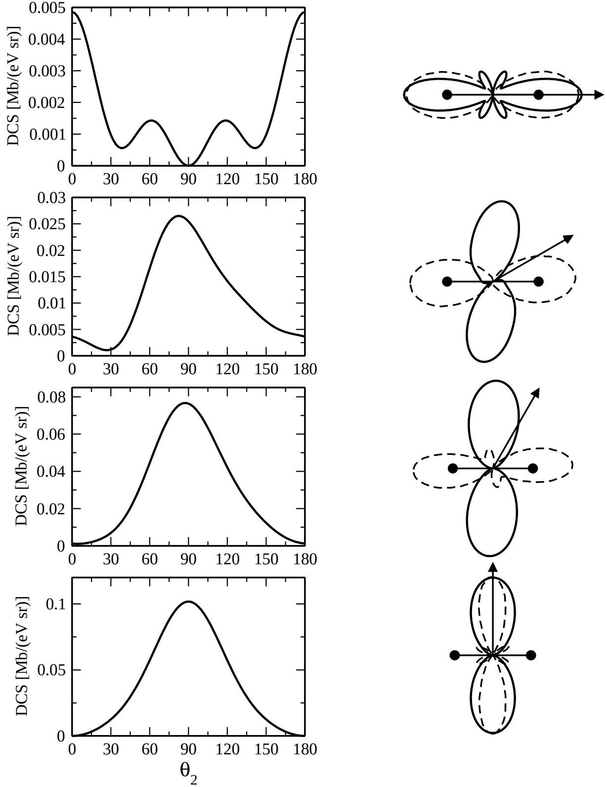
FIG. 5: Differential cross sections and angular distributions for \text{H}_2^+ at polarization angle \theta = 0^\circ, 30^\circ, 60^\circ, and 90^\circ (top to bottom) with respect to the molecular axis (horizontal) and a 10.0 eV ejected electron in the plane of the polarization and molecular axes. Solid curve: current result. Dashed curve: 2C un-normalized angular distributions of Walter and Briggs [30]. Note that for pure \Sigma polarization (top panel), the cross sections are roughly twenty times smaller than for pure \Pi polarization (bottom panel).
