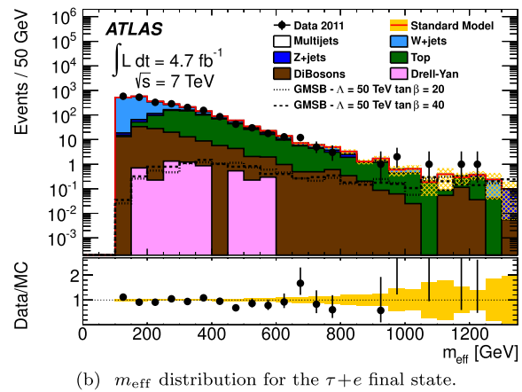
Fig. 4 Distribution of m_{\text{eff}} for the (a) \tau + \mu and (b) \tau + e final states after all analysis requirements. Data are represented by the points , with statistical uncertainty only. The SM prediction includes the data-driven corrections discussed in the text. The band centred around the total SM background indicates the uncertainty due to finite MC sample sizes on the background expectation. Also shown is the expected signal from two typical GMSB samples ( \Lambda = 50 TeV, \tan \beta = 40 , \Lambda = 50 TeV, \tan \beta = 20 ). In the top figure , the event in data surviving all the analysis requirements is shown in the overflow bin
