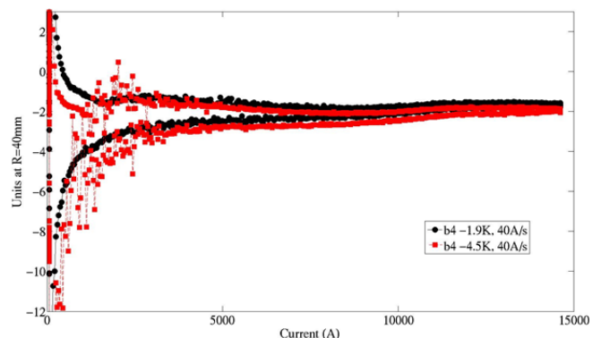
Fig. 16. There is evidence for flux jumps within the magnet cable. Larger amplitude is observed at lower currents and at 4.5 K rather than 1.9 K.
