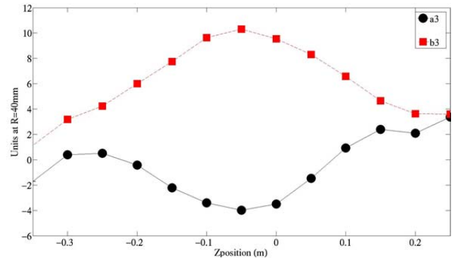
Fig. 5. Harmonics a_3 and b_3 vs probe Z-position, 14.6kA. Note that straight section center, defined by equal values of B_z in the ends, is Z=-0.05 .
