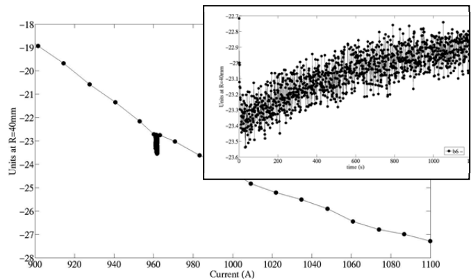
Fig. 15. b_6 in the vicinity of the injection porch (960A) during an accelerator cycle measurement. The inset shows the decay trend of b_6 vs. time at injection.
