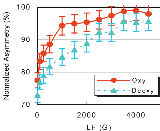
Fig. 2b. Longitudinal-field decoupling pattern representing asymmetry at around 1 \mu\text{s} versus applied longitudinal magnetic field for positive muon in oxyhemoglobin aqueous solution and deoxyhemoglobin solution at room temperature.
