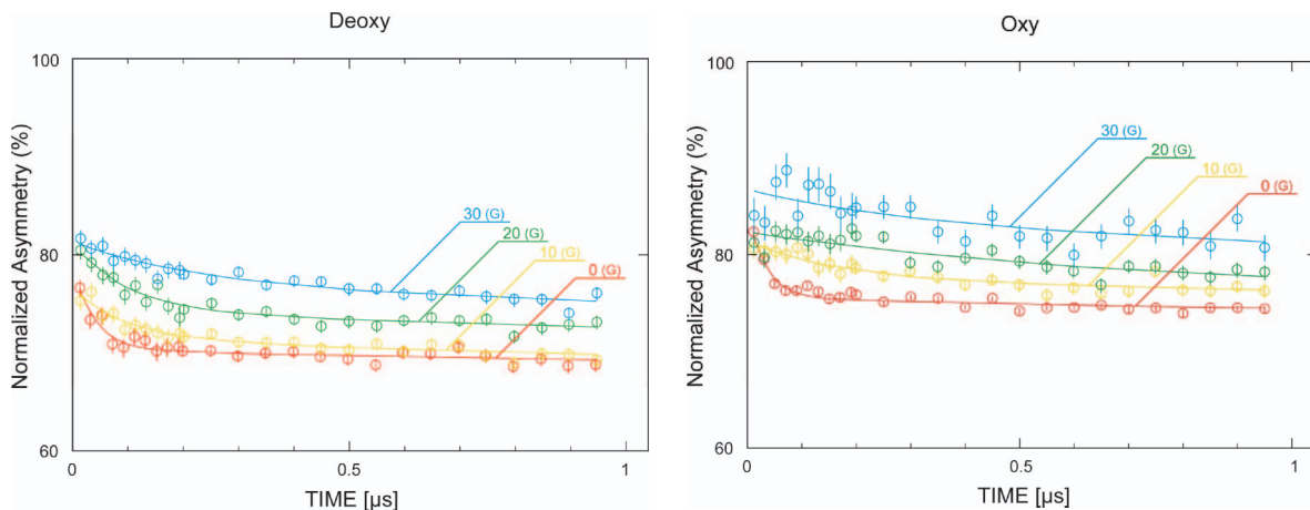
Fig. 2a. Muon spin relaxation time spectrum for positive muon in deoxyhemoglobin and oxyhemoglobin in aqueous solution at room temperature under upto 30 G longitudinal field. It is clearly seen that the earlier-time relaxation is maintained in deoxy-Hb and it is suppressed in oxy-Hb.
