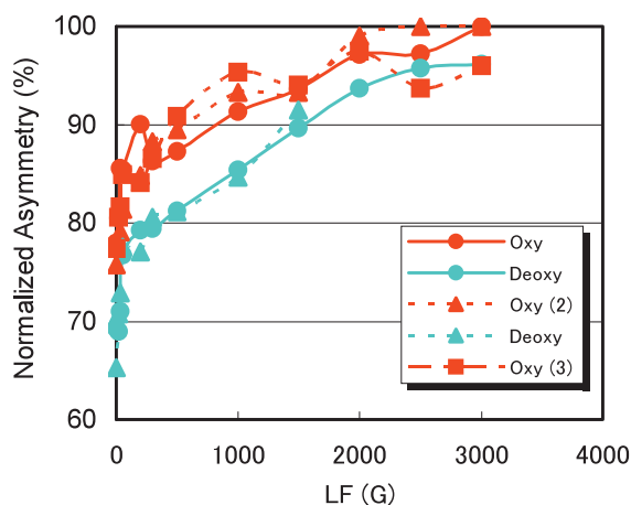
Fig. 3. Longitudinal decoupling pattern representing asymmetry at around 1 \mu\text{s} versus applied longitudinal magnetic field for positive muon in oxyhemoglobin containing human blood and deoxyhemoglobin containing human blood at room temperature taken from our previous work. 5)
