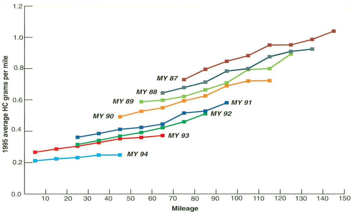
Average HC emissions by vehicle model year (MY) increase linearly with increasing mileage. Average emissions measured in 1995 are higher for earlier model years. More study is needed to determine if the difference in emissions by model year is due to improved technology or simply vehicle aging.
