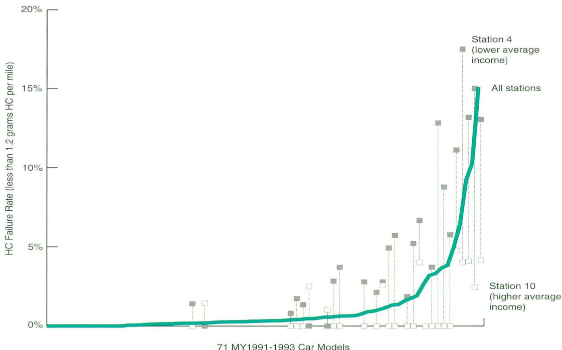
About half of 1991 to 1993 model year (MY) passenger car models have essentially no HC emissions failures within the first 2 to 5 years of driving. However, the models that do fail emissions tests most often have higher failure rates in lower income areas. This suggests that vehicle maintenance can affect in-use car emissions, at least for some car models.
