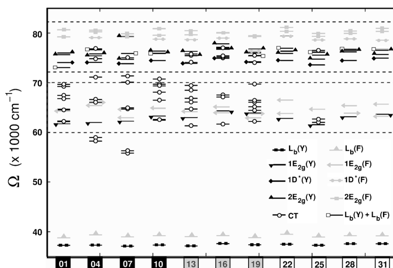
Figure 4. Transition frequencies from the ground state for the singly excited manifold ( L_b(Y) , L_b(F) ) and the bright excited states in the Vis ( 24000 – 32000 \text{cm}^{-1} ) and UV ( 35000 – 43000 \text{cm}^{-1} ) probing windows for selected snapshots. States with TDM magnitude below the threshold of 0.03 a.u., as well as local states in the range 40000 – 60000 \text{cm}^{-1} (e.g. L_a , B_a , B_b ), are not shown, as they do not appear in the presented nonlinear spectra. Snapshot labeling according to Figure 2.
