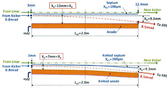
Figure 4: Possible ESS geometries.
