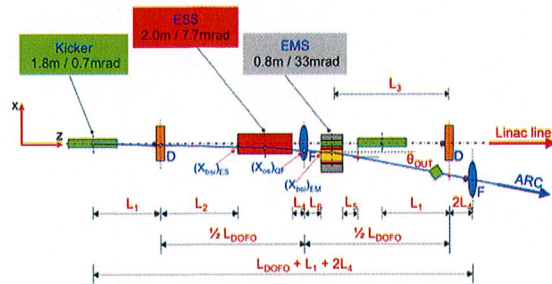
Figure 2: Schematic of a take-off section heading into a two-achromats branch line.
