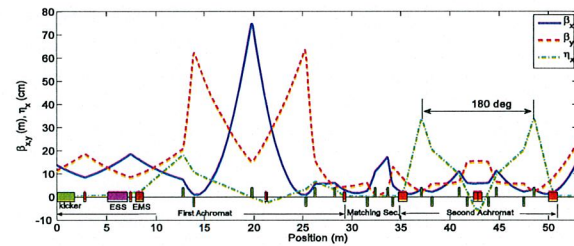
Figure 7: Twiss functions of one typical branch beam line.
