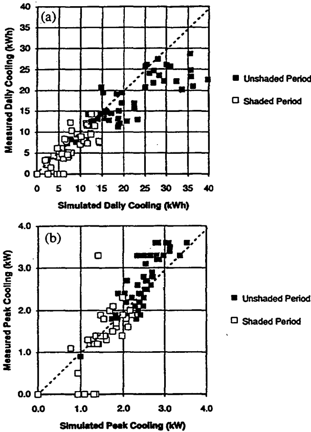
Fig. 7. Measured vs. simulated (a) daily cooling energy; (b) peak power usage at Site T1 during 1992. Simulations use weather data measured at the site. One week of data (June 27 to July 4) and some outliers were removed. When measured and simulated data are equal, they fall along the diagonal line. The plots indicate that the model overpredicts daily energy cooling use and underpredicts cooling load at peak conditions.
