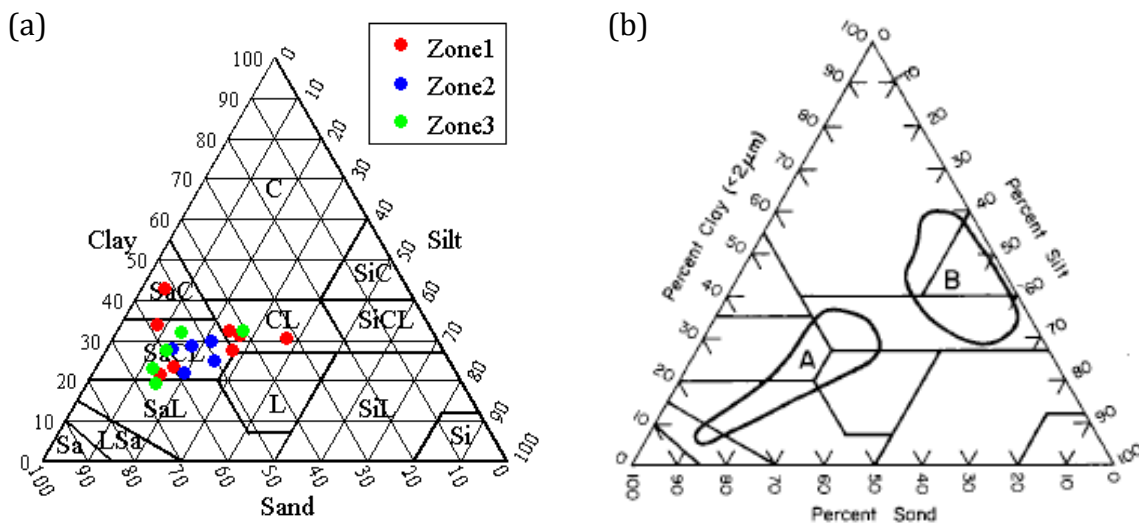
Figure 2. (a) Texture of deeper soil from the Ngee Sep. 2011 campaign on the USDA texture triangle. The symbols for the texture classes are Sa: Sand/Sandy, C: Clay, Si: Silt and L: Loam. (b) From Gersper et al. [1980] “Particle size distribution and texture of mineral horizons in soils from A) Aerice Pergelic Cryaquepts on sloping areas marginal to Footprint Creek (10 samples), and B) Histic Pergelic Cryaquepts and Pergelic Cryohemists in a moist meadow (86 samples)”.
