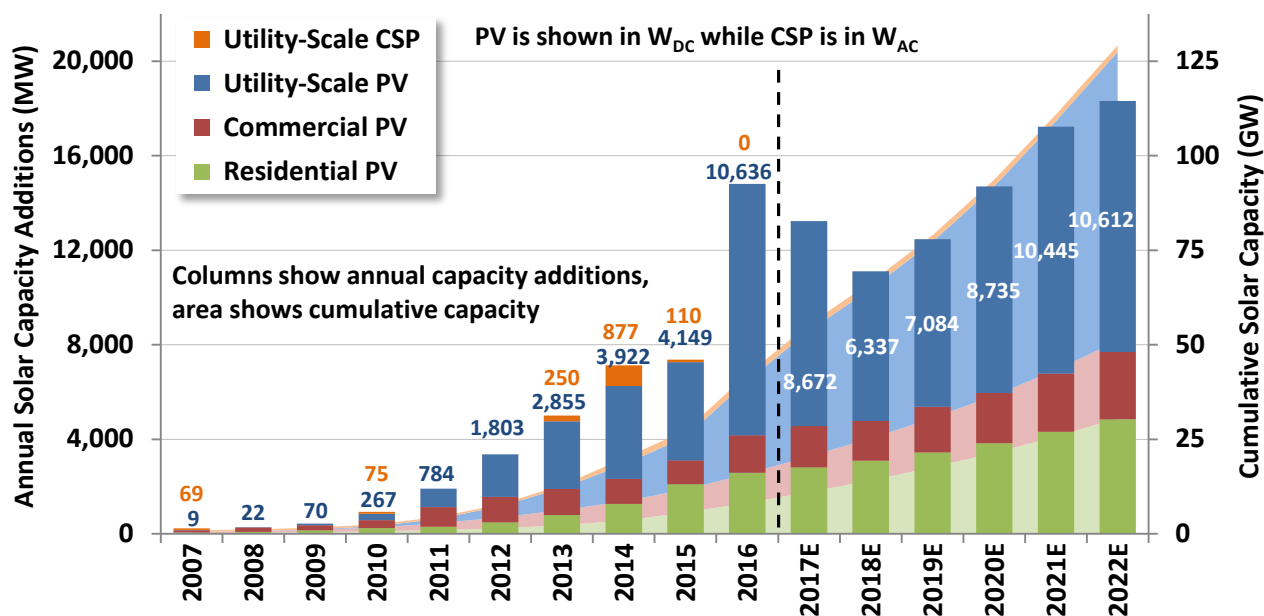
Figure 1. Historical and Projected PV and CSP Capacity by Sector in the United States 3
