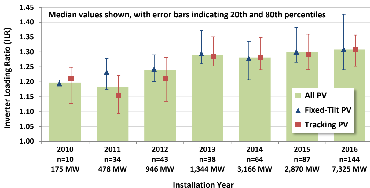
Figure 7. Trends in Inverter Loading Ratio by Mounting Type and Installation Year
