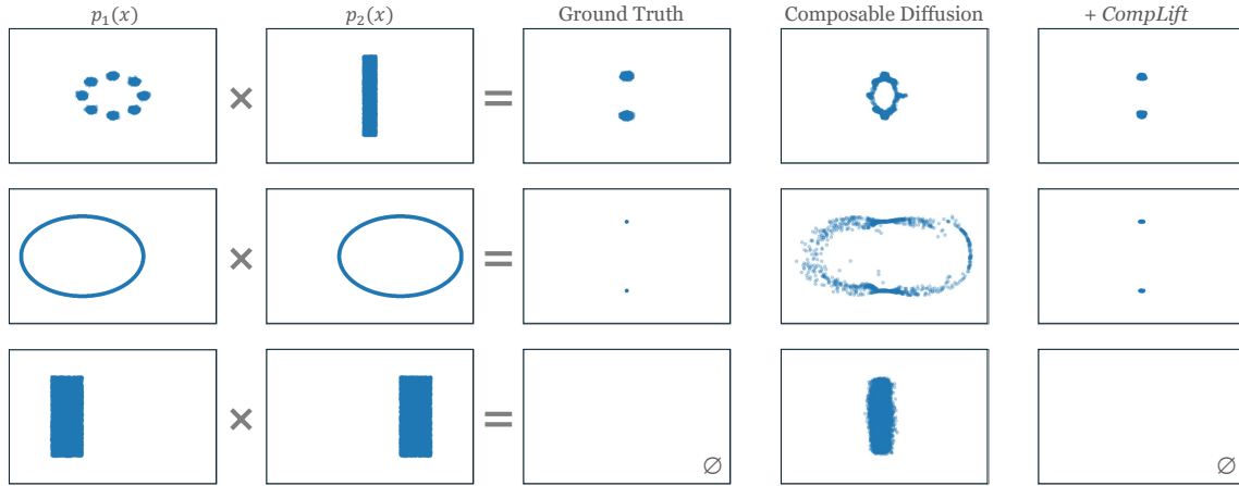
Figure 5.8: 2D synthetic result for product composition.
