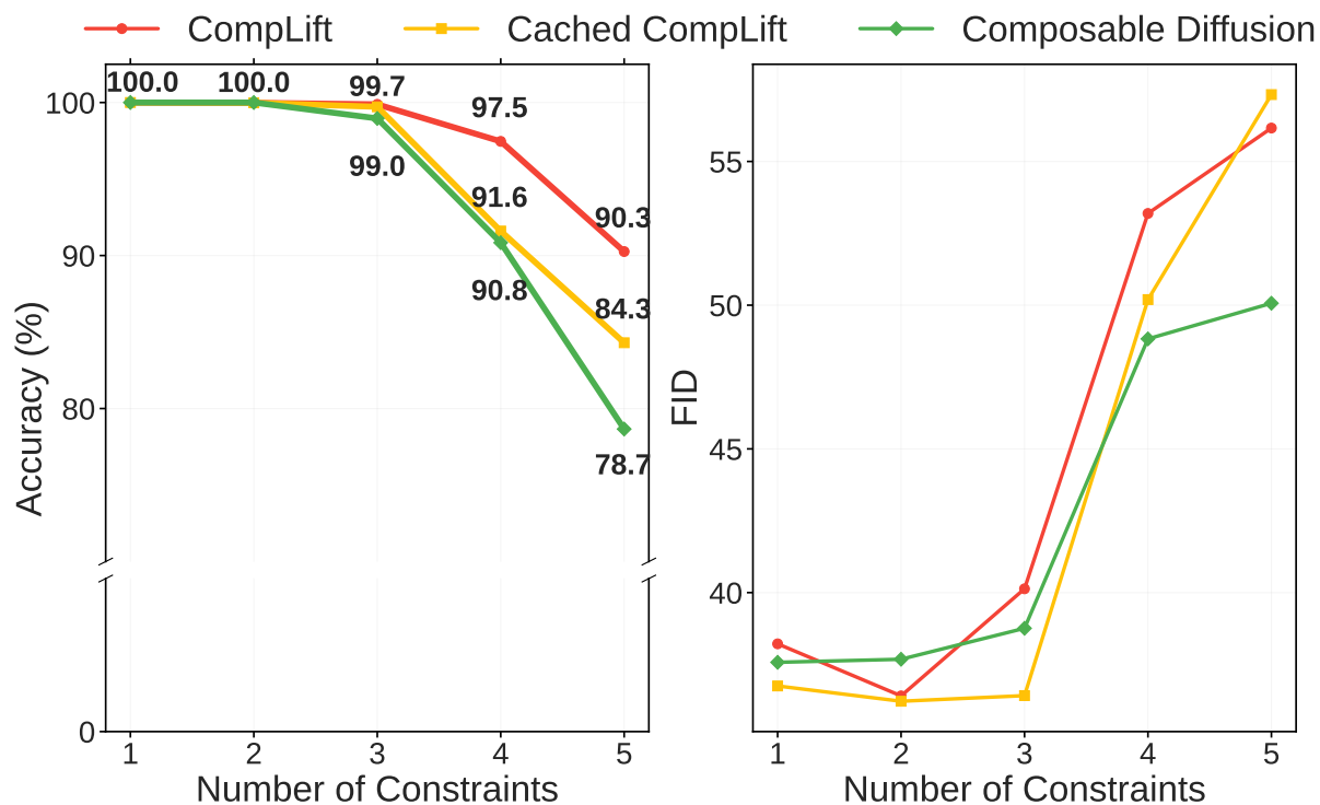
Figure 5.13: Quantitative results on CLEVR Position dataset.
