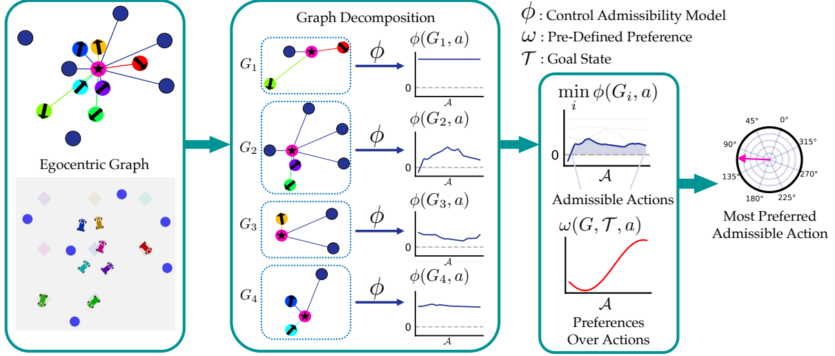
Figure 4.2: An overview of the proposed CAM approach. At each time step, the state of each agent is an egocentric graph. The graph is further decomposed at inference time into a set of subgraphs to follow the training data distribution. The CAM takes these subgraphs and outputs the admissibility scores along with a set of sampled candidate actions. We filter out the inadmissible actions by checking whether the minimum of the scores is below 0. Given a predefined preference over actions, the model outputs the most preferred action in the admissible set for each agent.
