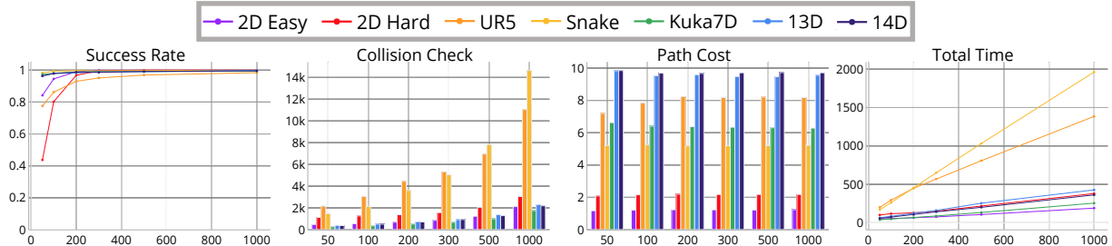
Figure 2.9: Comparison of performances for different probing samples from 2D to 14D problems.
