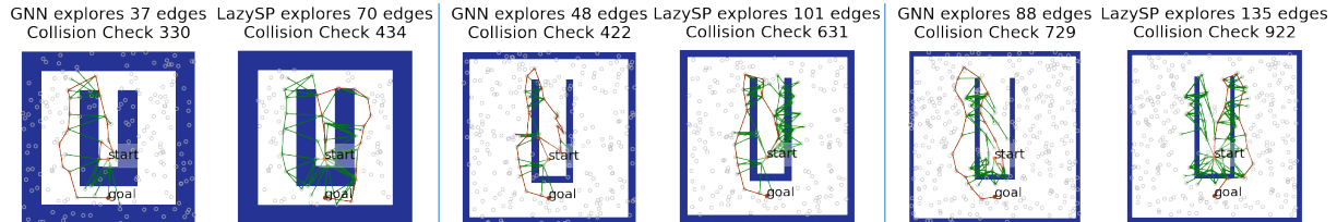
Figure 2.8: Comparison of performances with LazySP across different batch samples. The final path is colored red, and the other explored edges are colored green. From left to right we show examples of the search results with the batch size being 100, 200, and 300, respectively. We show obstacles of different thickness because the in-collision samples are also part of the inputs of the GNN planner, which can provide useful information about the topology of the environment.
