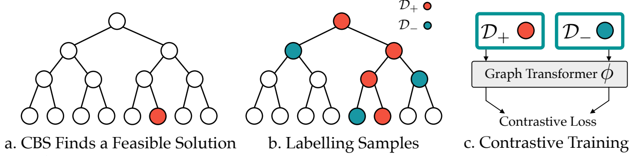
Figure 3.3: The training framework for Graph Transformer. We use a supervised Contrastive Loss. The labels are generated from the CBS search tree.
