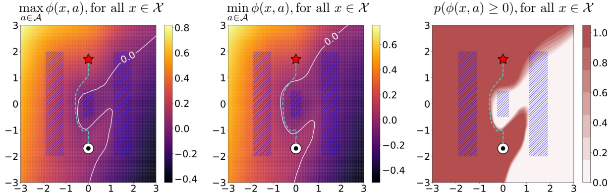
Figure 4.4: A proof of concept for the proposed CAM in a single-agent environment. The agent aims to reach the goal while avoiding obstacles. The black point denotes the starting state, and the red star denotes the goal state. The shaded blue regions denote the obstacles. Given the learned CAM \phi , action space \mathcal{A} : \{-0.1, 0.1\}^2 , and an arbitrary state x \in \mathcal{X} : \{-3, 3\}^2 , we illustrate \max_{a \in \mathcal{A}} \phi(x, a) , \min_{a \in \mathcal{A}} \phi(x, a) , and p(\phi(x, a) \geq 0) respectively. We show that the learned CAM never leaves the admissible set, i.e. \{x \in \mathcal{X} : \max_{a \in \mathcal{A}} \phi(x, a) \geq 0\} , along the trajectory.
