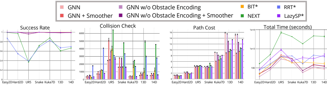
Figure 2.6: Comparison of performances on all environments from 2D to 14D, averaged over 4 random seeds. From left to right: (a) Success rate. (b) Collision checks. (c) Path cost. (d) Total planning time.
