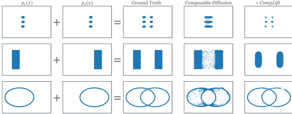
Figure 5.9: 2D synthetic result for mixture composition.
