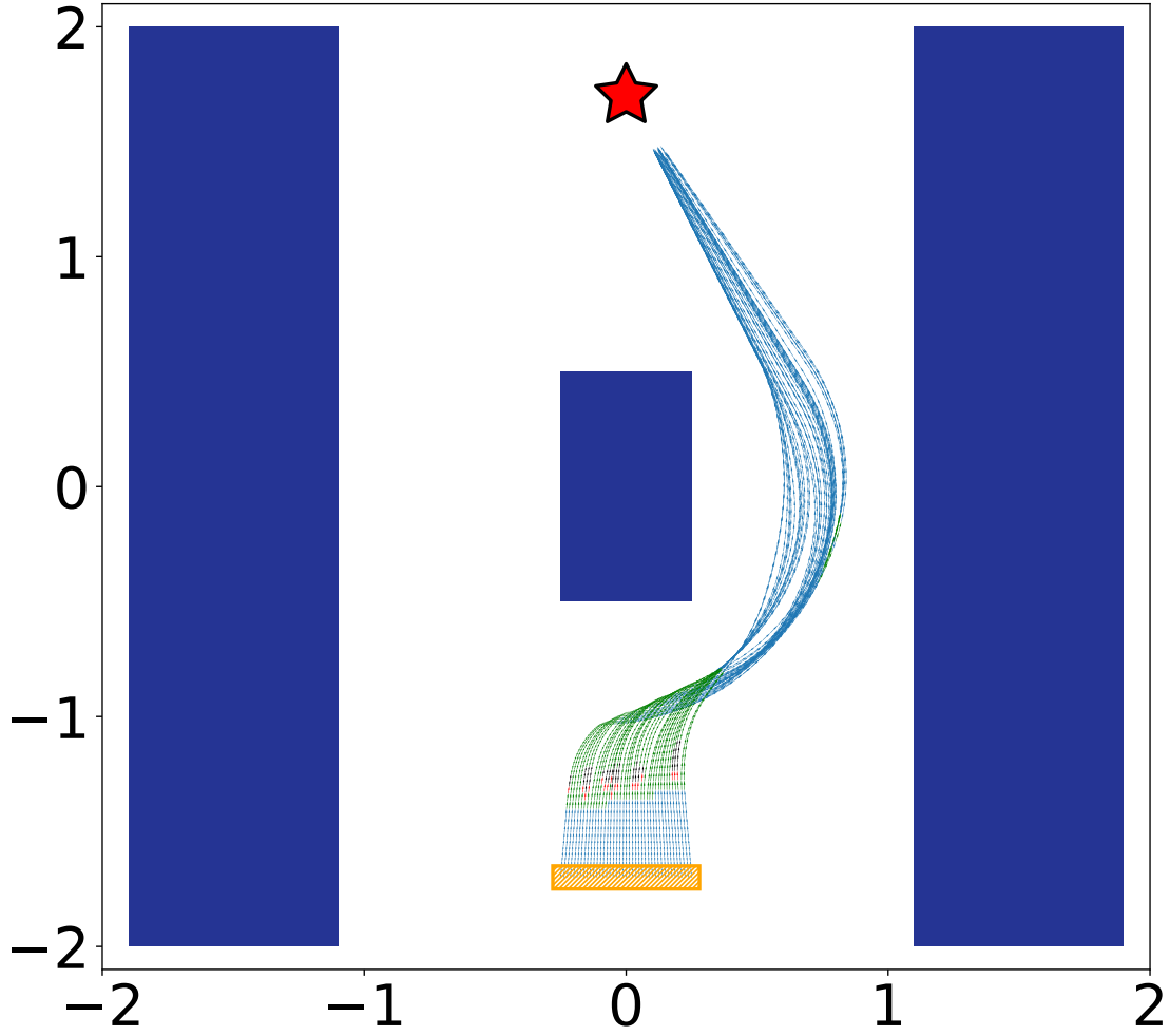
Figure 4.6: An additional single-agent example for the proposed CAM dealing with more complex dynamics, where the agent needs to catch failure early on. The red star represents the goal state, and three blue boxes represent the obstacles. The orange region denotes the set of initial states. We illustrate state-action pairs (x, a) on sampled trajectories starting from initial states. All trajectories reach the goal successfully with no collisions. The direction of each arrow indicates the action that CAM agent takes on each state x . The blue arrows represent the admissible region \{x \mid \forall a \in \mathcal{A}, \phi(x, a) \geq 0\} . Both the red and the green arrows represent the states on the boundary: \{x \mid \exists a_1, a_2 \in \mathcal{A}, \phi(x, a_1) \geq 0, \phi(x, a_2) < 0\} . Only the red arrows represent those boundary transitions that violate the forward-invariance property. The black arrows represent the states in the inadmissible region \{x \mid \forall a \in \mathcal{A}, \phi(x, a) < 0\} .
