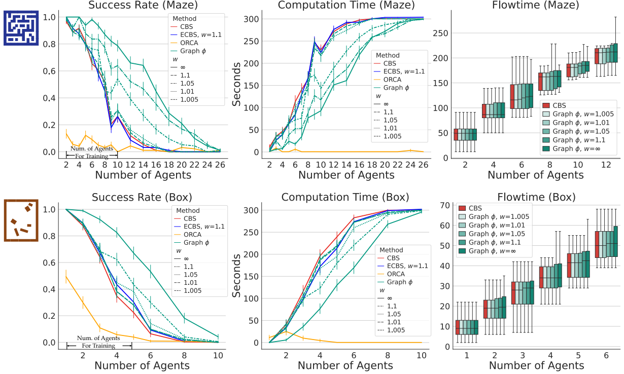
Figure 3.4: Success rates, computation time, and flowtime within the runtime limit of 5 minutes, as functions of the number of agents. The results are averaged over 100 test instances for each setting of the agent number. We evaluate our approach with w \in [1.005, 1.01, 1.05, 1.1, \infty] , and compare its performance with CBS, ECBS ( w = 1.1 ) and ORCA. Though trained with relatively few agents, results have shown that our approach generalizes well and significantly outperforms the baselines.
