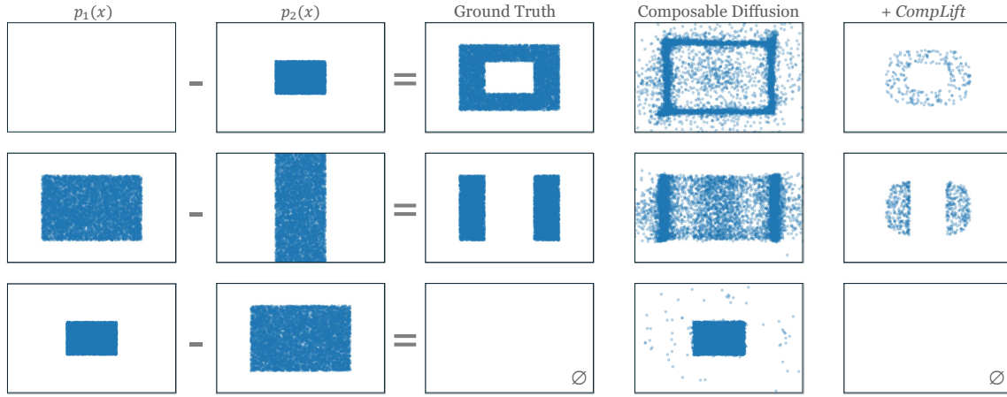
Figure 5.10: 2D synthetic result for negation composition.
