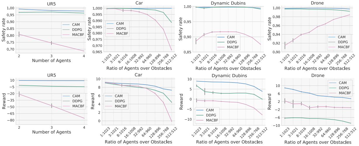
Figure 4.7: We show the performances of CAM and prior methods in the UR5, Car, Dynamic Dubins, and Drone environment, where each method is trained with 3 agents during training but tested up to 512 agents. CAM substantially outperforms prior approaches in all the environments.
