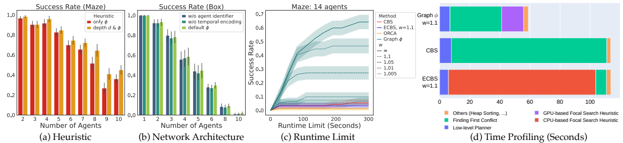
Figure 3.5: We conduct 4 various ablation studies to evaluate the proposed method systematically. See Section 3.5.2 for more details.
