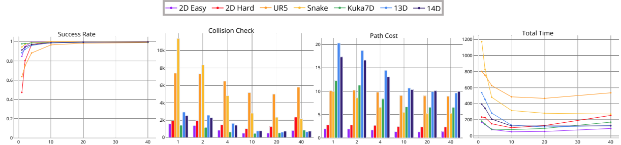
Figure 2.13: Ablation study on different k_0 for k-NN. Performances are best at k_0 \in [10, 20] .
