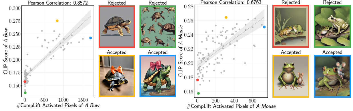
Figure 5.17: More examples of correlation between CLIP and CompLift . Prompt to generate left images: a turtle with a bow. Prompt to generate right images: a frog and a mouse.
