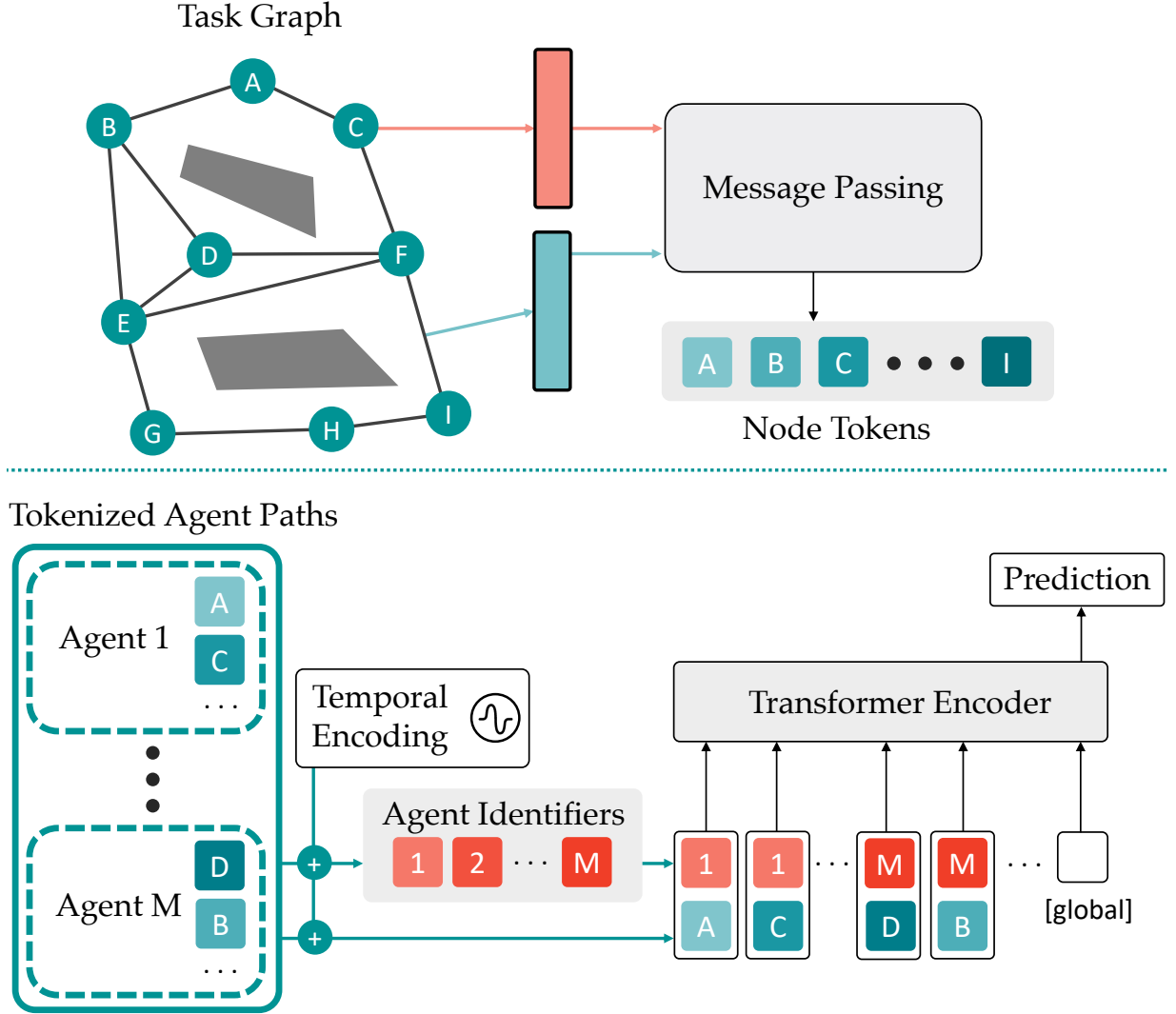
Figure 3.2: The proposed Graph Transformer architecture. It has several desired properties that are specifically designed to deal with MAPF inputs. See Section 3.4.1 for more details.
