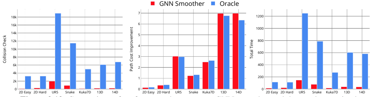
Figure 2.12: Comparison of performance between our GNN smoother and the oracle to trained on. Our GNN smoother learns to smooth the path with comparable improvement as the oracle, and also requires fewer collision checking steps and less total time.
