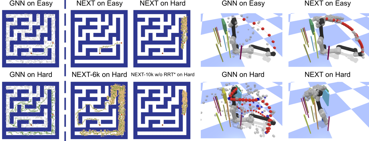
Figure 2.7: We test the generalization capability of GNN-based approaches and NEXt by constructing pairs of problems that have small but important difference in connectivity. The GNN models find paths on both environments quickly, while NEXt gets stuck in hard instances because of the lack of access to the graph structure provided by probing samples. The explored vertices of GNN on UR5 environment are colored in blue, and the edges on the path are colored in red.
