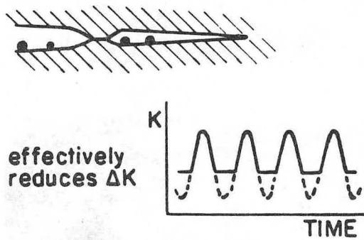
2) Crack Closure
