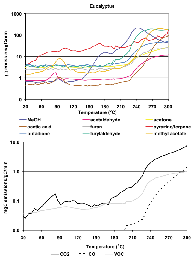
Fig. 2. Emission factors (μgC/gC) of the most abundant VOCs emissions versus temperature (top panel) and total VOC, CO 2 and CO emission (lower panel) for Eucalyptus leaf tissue.
