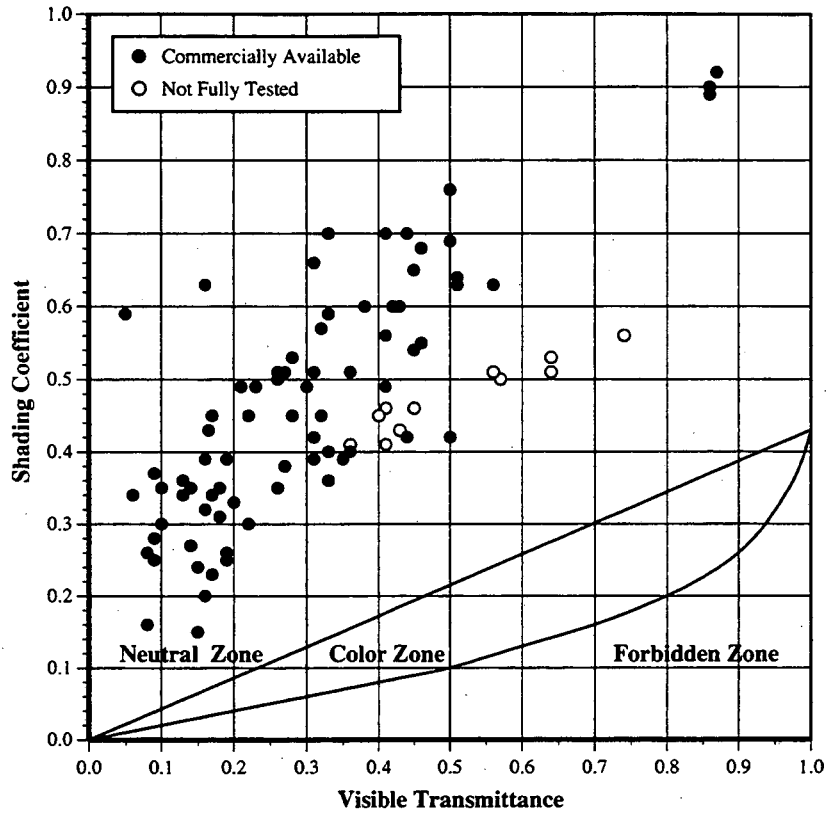
Figure 10. Spectral selectivity of coatings on plastic film that are laminated to clear or heat absorbing glazings. Open symbols represent new products that have not been fully tested.
