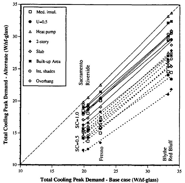
Figure 8. Peak demand ( \text{W}/\text{ft}^2\text{-glazing} ) for glazing shading coefficient values of 0.5 (dotted lines) and 1.0 (solid lines) for alternate housing characteristics in five California climates. Base case prototype glazing shading coefficient is 1.0. Glazing area is 3.5% window-area-to-floor-area ratio per orientation.
