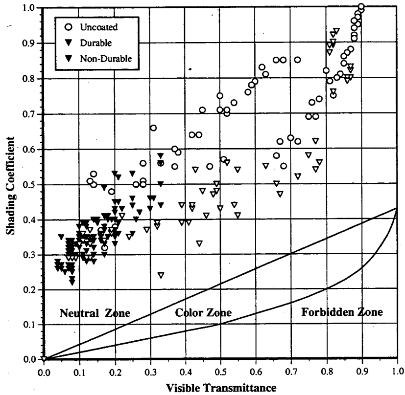
Figure 11. Spectral selectivity of commercial glazings and coatings applied to glass.
