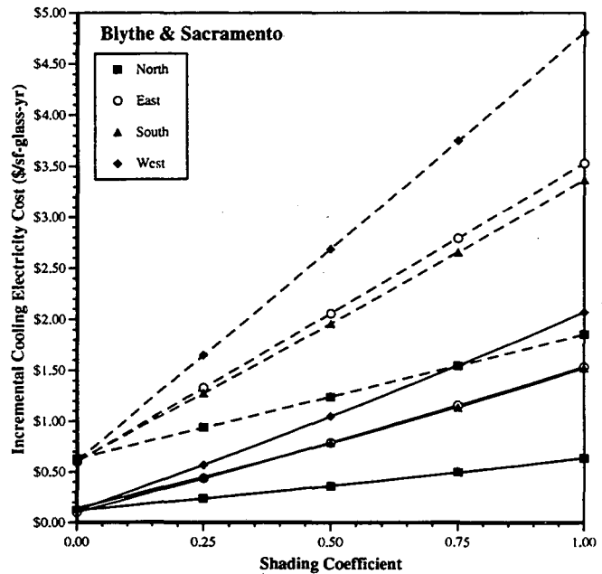
Figure 3. Incremental cooling electricity cost ( \$/\text{ft}^2\text{-glazing-yr} ) for a 1540 ft 2 (143 m 2 ) residence in Sacramento (solid lines) and Blythe (dotted lines), California with a glazing area of 3.5% window-area-to-floor-area ratio per orientation. Incremental is defined as the difference in energy cost between a window and an insulated wall.
