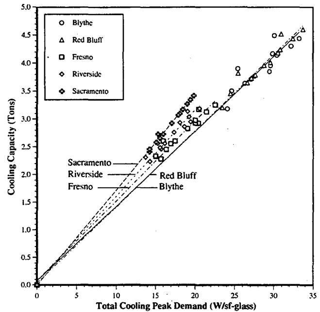
Figure 6. Total peak demand due to cooling ( W/ft^2 -glazing) versus cooling capacity of air-conditioning equipment for a 1540 ft^2 (143 m^2 ) residence in five California climates with a glazing area of 3.5% window-area-to-floor-area ratio per orientation. Datapoints include the base case prototype and all alternate housing characteristics for glazing shading coefficient values of 0.5 and 1.0.
