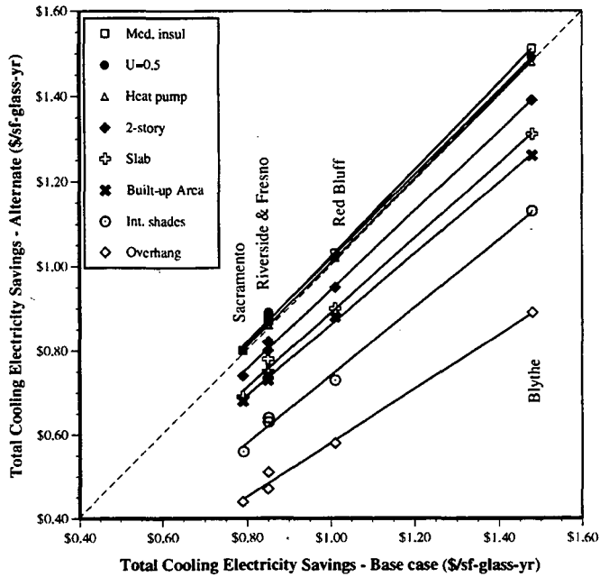
Figure 7. Total cooling electricity savings ( \$/\text{ft}^2\text{-glazing-yr} ) due to a reduction in glazing shading coefficient of 0.5 for alternate housing characteristics in five California climates. Glazing area is 3.5% window-area-to-floor-area ratio per orientation.
