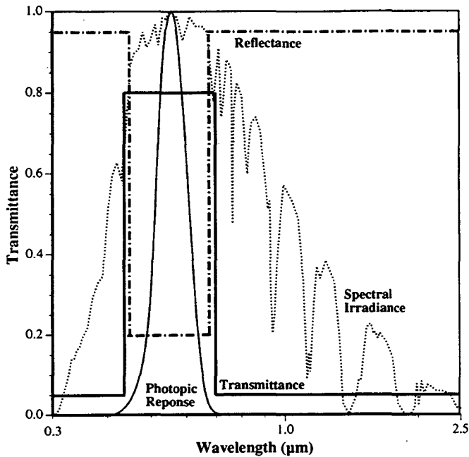
Figure 1. Solar spectral properties of an ideal spectrally selective glazing. The shaded region of the solar spectrum represents the response of the eye to light.
