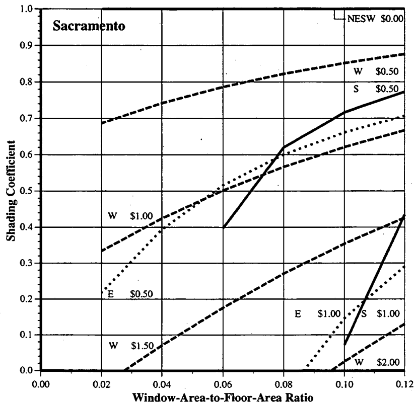
Figure 9b. Total cost savings (z-axis: $/ft 2 -glazing-yr) due to a reduction in shading coefficient from 1.0 to the y-coordinate value of SC and x-coordinate WFR for a 1540 ft 2 (143 m 2 ) residence in Sacramento, California. Notation on graph is: N=North, E=East, S=South, W=West window orientation.
