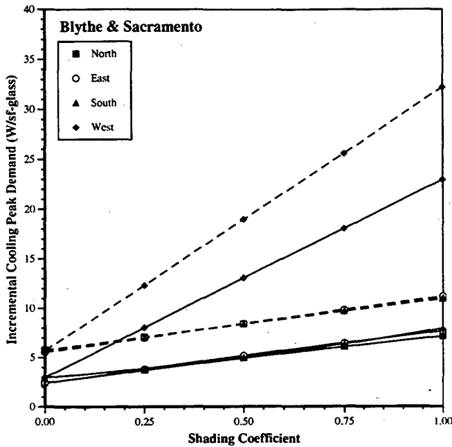
Figure 5. Incremental peak demand due to cooling ( W/ft^2 -glazing) for a 1540 ft^2 (143 m^2 ) residence in Sacramento (solid lines) and Blythe (dotted lines), California with a glazing area of 3.5% window-area-to-floor-area ratio per orientation.
