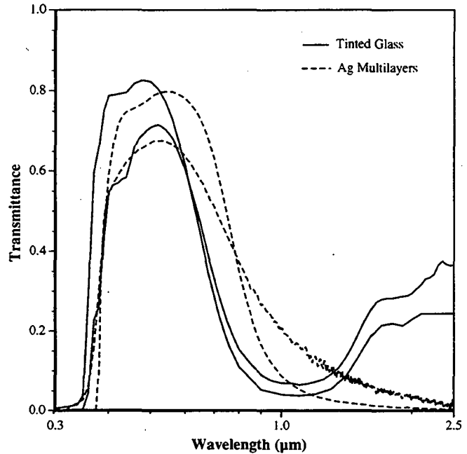
Figure 2. Solar transmission spectra of the best available spectrally selective glazings.
