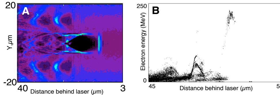
FIGURE 4. Simulations show that beam loading and pulse evolution turn off injection after the trapping of an initial bunch, resulting in a bunch isolated in phase space. This is visible in the density contour (A), where the wake amplitude is lowered following the bunch in the first bucket. The particles are then concentrated in energy at the dephasing length (B).
