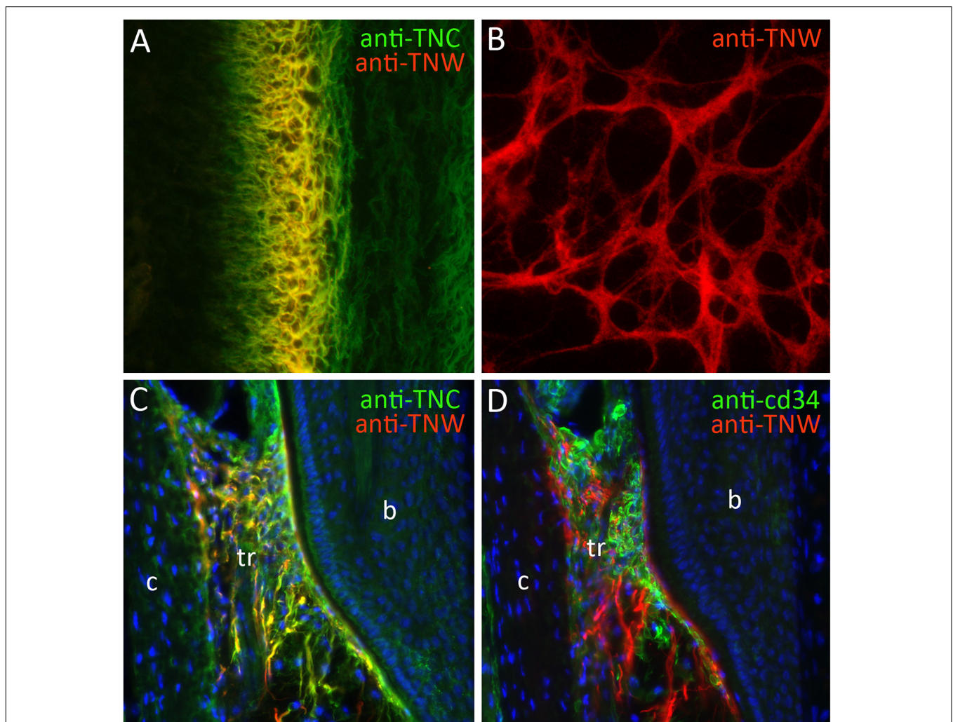
FIGURE 2 | The expression of tenascin-W (TNW). (A) Double-label immunohistochemical localization of tenascin-C (TNC) and TNW in the scleral ossicles of an E10 chicken. TNW is commonly expressed at sites of osteogenesis, where it is typically found in the subset of the extracellular matrix labeled with antibodies to TNC. (B) After 6 days in culture primary chicken osteoblasts elaborate a TNW-rich extracellular matrix in the presence of BMP2. (C) Anti-TNC and anti-TNW both label fibrils in the trabecular region (tr) of adult mouse whisker follicles between the bulge (b) and the capsule (c). TNW-positive fibrils are typically, but not always, a subset of the TNC-positive fibrils. (D) The TNW-rich trabecular region contains cd34-positive stem cells.
