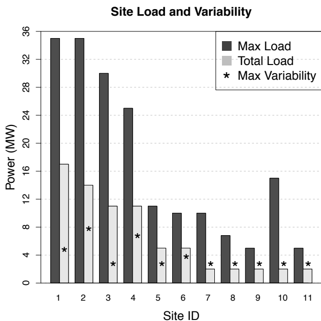
Fig. 1. Site Load and Variability
