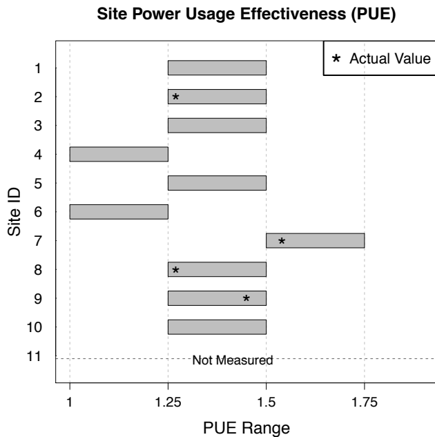
Fig. 2. Site Power Usage Effectiveness
