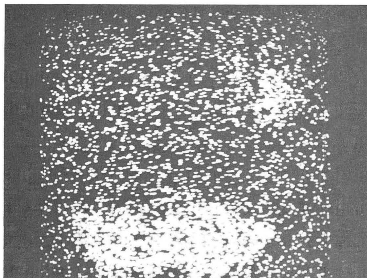
Fig. 8 Photomicrograph showing Al 2 O 3 pockets in undoped material.
