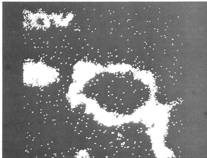
Fig. 6 Photomicrograph showing \text{Al}_2\text{O}_3 pockets in \text{Al}_2\text{O}_3 doped materials.
