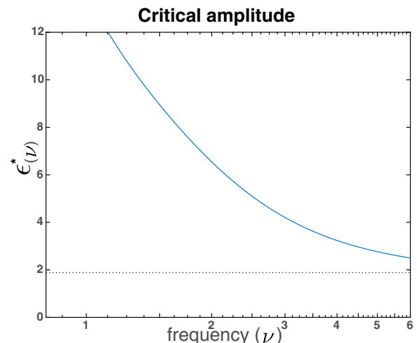
Fig. 9. Critical amplitude, \epsilon^*(\nu) = |\hat{a}_1(\nu)/\hat{a}_2(\nu)| . The asymptote at high frequencies is \epsilon^*(\infty) = 32/17 (dotted line).
