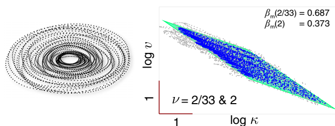
Fig. 6. Elliptic-spiral movement exhibiting a mixture of power laws. (Left) Movement trajectory drawn by a subject. (Right) Log speed vs. log curvature plot. The filtered data points form a parallelogram with sides having approximately -1/3 and -2/3 slopes (green region). On each elliptic arc, the points form a straight line with -1/3 slope. Successive arcs translate along a broader line with -2/3 slope as the ellipse size slowly changes. Gray dots: raw data. Blue dots: smoothed data with a dual-band filter centered at \nu=2/33 and \nu=2 . \beta_m : measured exponent for each frequency band. (Scale bar: 1.0.)
