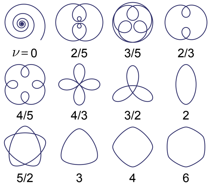
Fig. 4. Examples of pure frequency curves shown with their characteristic frequencies, \nu . See https://www.youtube.com/watch?v=waXW0vYqFE for a movie showing how the shape of the curve varies with continuously changing angular frequency.
