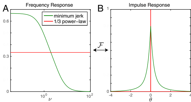
Fig. 8. (A) The frequency-dependent power law exponent, \beta(\nu) , can be understood as the frequency response function of a linear low-pass filter. The one-third power law has a flat frequency response. (B) Corresponding impulse response functions, \hat{\beta}(\theta) . The width of this noncausal filter is \approx 1 radian. The one-third power law has a delta function impulse response.
