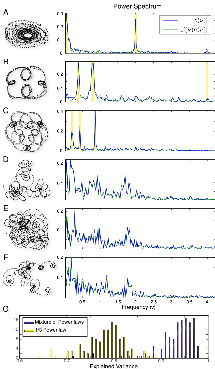
Fig. 7. Complex free-hand movements ( Left ) and corresponding amplitude spectra ( Right ) comparing log speed [ \tilde{z}(\nu) , blue line] and the power law exponent times log curvature [ \beta(\nu)\tilde{h}(\nu) , green line]. Vertical yellow bars indicate the specified frequency components. ( A ) An elliptic-spiral movement exhibiting peaks at 2 and 2/33, corresponding to contributions from the elliptical and the spiral components, respectively. ( B ) Multifrequency movements with peaks at 2/5, 4/5, and a minor peak at 4. ( C ) Multifrequency movements with three peaks at 3/14, 3/7, 6/7. ( D–F ) Random doodles with broadband power spectra. ( G ) Histogram showing the proportion of the log speed variance explained by the model [ \beta(\nu)\tilde{h}(\nu) , purple bars] or the 1/3 power law (yellow bars) for multifrequency movements, including A–F .
