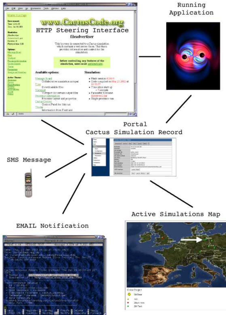
Fig. 2. Diagram displaying the current range of interactions between the ASC Portal and a running Cactus simulation. The application announces to the portal, sending information such as the hostname, the username, the name of the executable, and the location of the data being created. It also sends a URL for contacting the Cactus simulation via an HTTP steering interface, displayed in the upper left corner of the diagram. The ASC Portal notifies group members that the simulation has started by sending emails and/or messages to cellphones. Users may view the location of active simulations on an interactive map.
