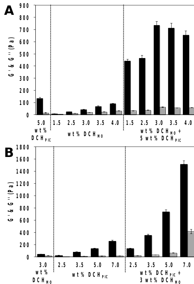
Figure 2. Mechanical properties of single and dual compartment diblock copolyptide hydrogels. (A) G' (Pa, black) and G'' (Pa, white) of DCH_{DC} composed of 5 wt% DCH_{PIC} and varying concentrations of DCH_{MO} in 1× PBS buffer at 25 °C. Data for individual 5 wt% DCH_{PIC} and DCH_{MO} hydrogel components at different concentrations in 1× PBS buffer at 25 °C are included for reference. (B) G' (Pa, black), and loss modulus, G'' (Pa, white), of DCH_{DC} composed of 3 wt% DCH_{MO} and varying concentrations of DCH_{PIC} in 1× PBS buffer at 25 °C. Data for individual 3 wt % DCH_{MO} and DCH_{PIC} hydrogel components at different concentrations in 1× PBS buffer at 25 °C are included for reference. All G' and G'' values were measured at an angular frequency of 5 rad/s and a strain amplitude of 0.01, and are averages of triplicate runs with bars indicating standard deviations.
