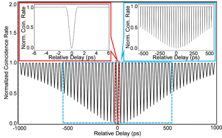
Fig. 2.11. Hong-Ou-Mandel quantum revival of the high-dimensional biphoton frequency combs.
