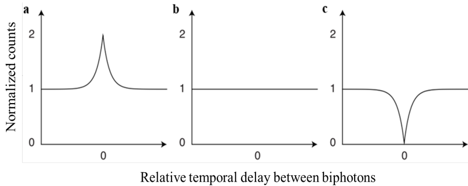
Fig. 2.2. Second-order coherence functions g^{(2)}(\tau) for thermal, coherent and quantum light sources. a) Bunching statistics of thermal light. b) Coherent light statistics. c) Anti-bunching statistics of quantum light.
