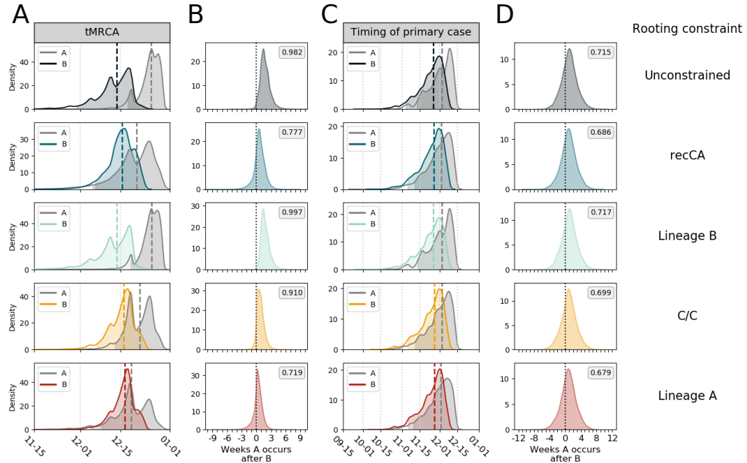
Figure B.25. The timing of the MRCA and primary case for lineage A and lineage B with a shorter doubling time. The simulations used here have a doubling time of 2.65 days (95% HDI: 1.50-4.10). Each row represents a different rooting constraint in phylodynamic analysis, with the bottom three representing a fixed ancestral haplotype. (A) The tMRCA for lineages A and B. (B) The number of weeks the tMRCA of lineage A occurs after the tMRCA of lineage B. (C) The timing of the primary case for lineages A and B. (D) The number of weeks the time of the primary case of lineage A occurs after the time of the primary case of lineage B. Long dashed lines indicate the median and shading represents the 95% HPD for each distribution. Short dashed lines indicate 0 weeks difference between lineages A and B. Posterior probability that lineage A originated after lineage B is reported in the grey box.
