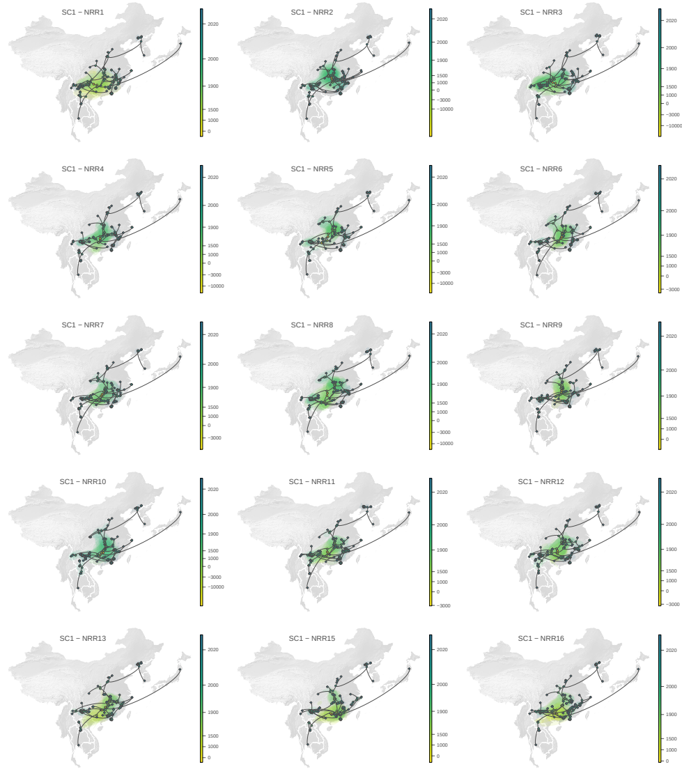
Figure C.9. Continuous phylogeographic reconstruction of the dispersal history of viral lineages for the SARS-CoV-1-like (SC1) viruses. We report the reconstructions obtained for NRRs 1-13 and 15-16 (NRR14 being reported in the main Fig. 3.3g; see Fig. C.10 for NRRs 17-31). For each NRR, we map the maximum clade credibility (MCC) tree whose nodes are coloured from yellow (the time of the most recent common ancestor) to blue (most recent collection date) and are superimposed on 80% HPD polygons coloured according to the same log-transformed time scale and reflecting the uncertainty of the Bayesian phylogeographic inference. HPD polygons were only computed and reported for the last 1,000 years. As in Fig. 3.3g-h, MCC tree tip nodes are displayed as squares (as opposed to dots for internal ones) and dispersal direction (anti-clockwise) of viral lineages is indicated by the edge curvature.
