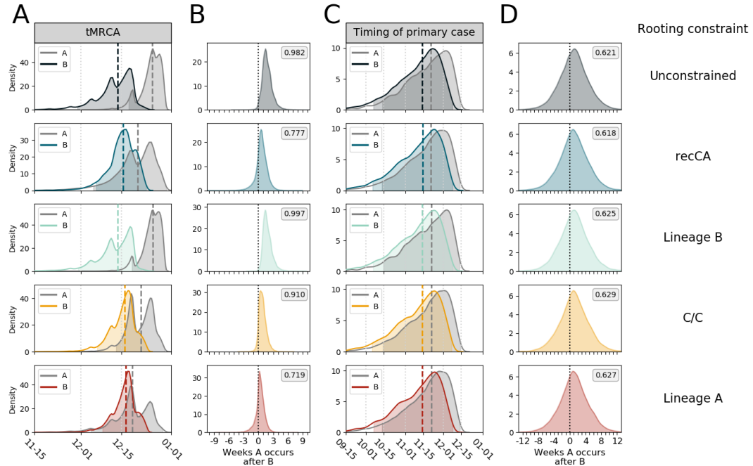
Figure B.26. The timing of the MRCA and primary case for lineage A and lineage B with a longer doubling time. The simulations used here have a doubling time of 4.45 days (95%: HDI: 1.50-7.44). Each row represents a different rooting constraint in phylodynamic analysis, with the bottom three representing a fixed ancestral haplotype. (A) The tMRCA for lineages A and B. (B) The number of weeks the tMRCA of lineage A occurs after the tMRCA of lineage B. (C) The timing of the primary case for lineages A and B. (D) The number of weeks the time of the primary case of lineage A occurs after the time of the primary case of lineage B. Long dashed lines indicate the median and shading represents the 95% HPD for each distribution. Short dashed lines indicate 0 weeks difference between lineages A and B. Posterior probability that lineage A originated after lineage B is reported in the grey box.
