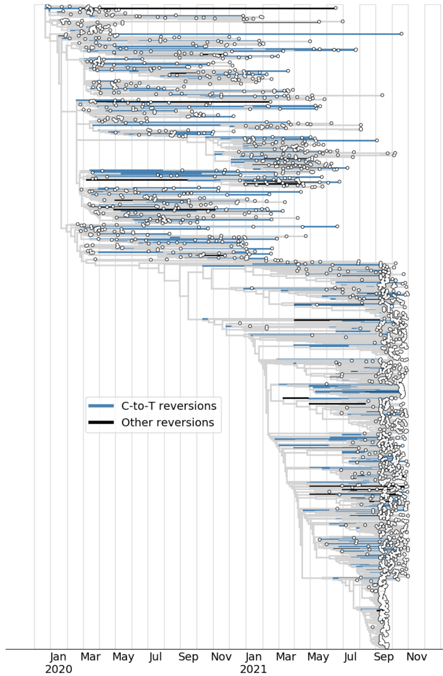
Figure B.16. Subsampled global phylogeny showing reversions. Subsampled SARS-CoV-2 time-resolved phylogeny from Nextstrain, with reversions colored blue if a C-to-T reversion and black otherwise.
