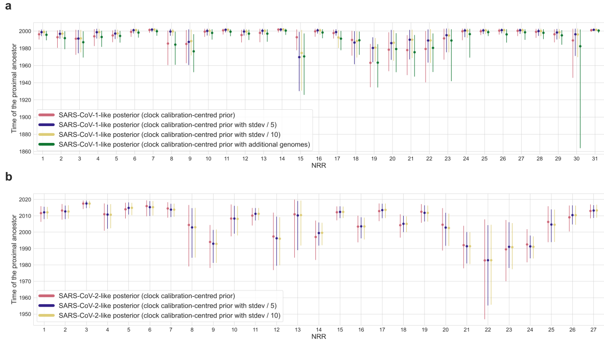
Figure C.5. Time of the closest-inferred ancestor sensitivity analysis. a, Time of the closest-inferred ancestor of SARS-CoV-1 across the 31 NRRs of the SARS-CoV-1-like viruses with the calibrated molecular clock from the SARS-CoV-1 analysis, the calibrated molecular clock but the standard deviation of the clock rate divided by 5, the calibrated molecular clock but the standard deviation of the clock rate divided by 10, and when adding in one SARS-CoV-1 genome from a civet and an additional SARS-CoV-1 genome from a human. b, Time of the closest-inferred ancestor of SARS-CoV-2 across the 27 NRRs of the SARS-CoV-2-like viruses with the calibrated molecular clock from the SARS-CoV-2 analysis, the calibrated molecular clock but the standard deviation of the clock rate divided by 5, and the calibrated molecular clock but the standard deviation of the clock rate divided by 10. The dots indicate the median and the lines are the 95% HPD. Refer to Supplementary Tables 3 and 4 for numerical values.
