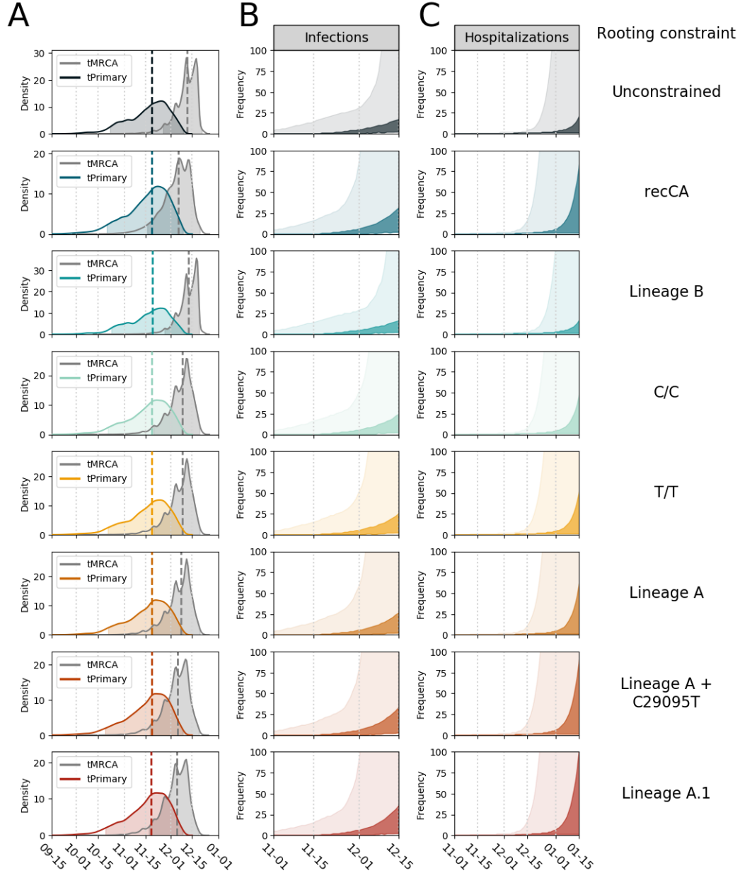
Figure B.29. Single-introduction timing of the MRCA and primary case and subsequent epidemic growth. (A) Posterior distributions of the timing of the MRCA (tMRCA) and primary case (tPrimary), with dashed lines indicating the median and shading representing the 95% HPD for each distribution. (B) Estimated number of infections in late 2019. Darker shading represents 50% HPD; lighter shading represents 95% HPD. (C) Estimated number of hospitalizations in late 2019. The legend indicates the phylodynamic model used: the unconstrained model uses just the SARS-CoV-2 genomes; the recCA-constrained model constrains the ancestor of the MRCA of SARS-CoV-2 as the recCA; the remaining models constrain the MRCA of SARS-CoV-2 as a particular sequence (Fig. B.20; see methods).
