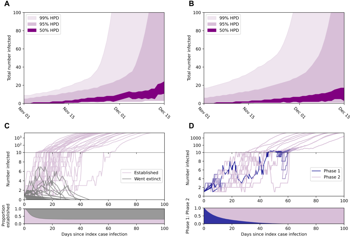
Figure 1.4. Epidemic growth in compartmental simulations. (A) Total estimated people infected in late-2019. Dark purple shading is central 50% HPD, intermediate purple shading is central 95% HPD, and light purple is central 99% HPD. (B) Total estimated people infected in late-2019 for a two-phase epidemic. (C) The number of people infected over time in a sample of epidemic simulations that established (purple; n=30 ) and went extinct (grey; n=70 ). The y-axis transitions to log-scale once \geq 10 people are infected at any given time. The lower panel shows the proportion of simulations that still have \geq 1 infected individual over time (persisting epidemics in purple; extinct epidemics in grey). (D) A sample ( n=10 ) of two-phase epidemic simulations transitioning from less-fit Phase 1 (blue) to more-fit Phase 2 (purple). Each line represents a single simulation and its transition over time. The lower panel shows the average proportion of Phase 1 to Phase 2 infected individuals over time.
