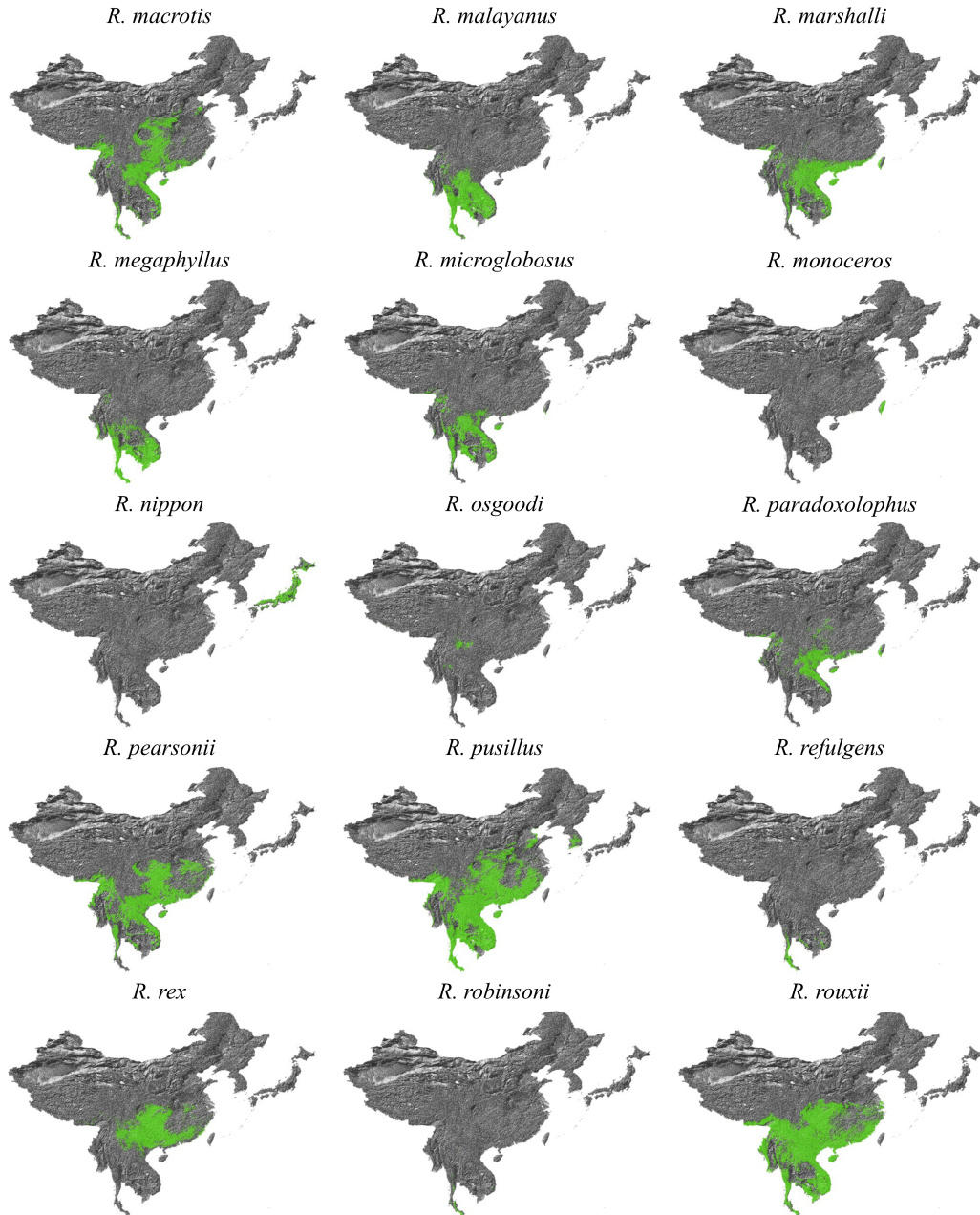
Figure C.14. Distribution maps for species of the Rhinolophus genus, part 2. See Fig. C.13 and C.15 for remaining bat distribution maps.
