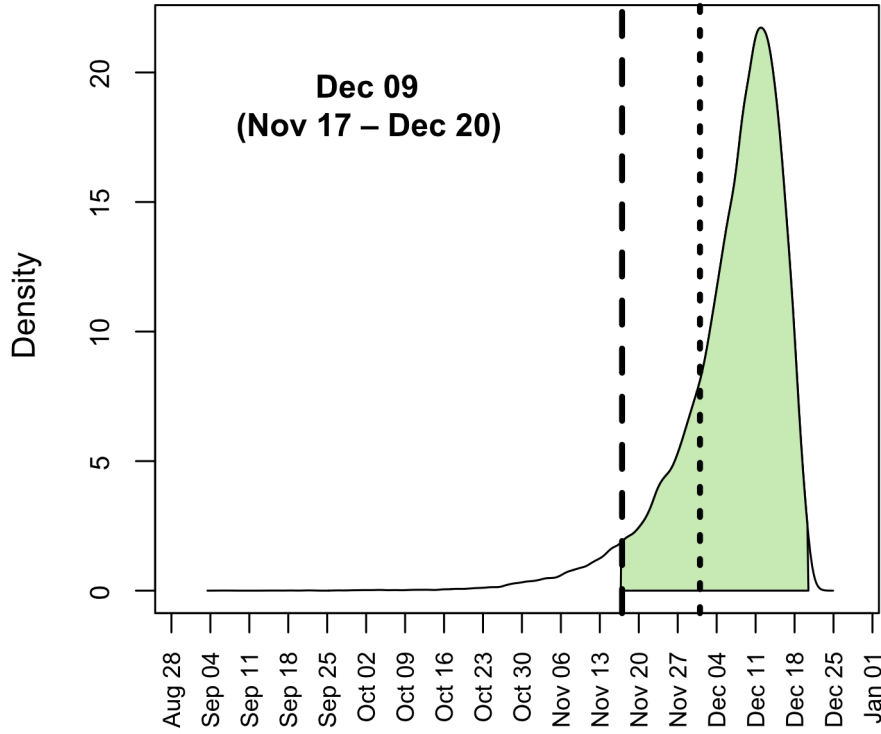
Figure 1.1. Posterior distribution for the time of the most recent common ancestor (tMRCA) of 583 sampled SARS-CoV-2 genomes circulating in China between December 2019 and April 2020. Inference was performed using a strict molecular clock and a Bayesian Skyline coalescent prior. Shaded area denotes 95% HPD. Long-dashed line is 17 November 2019, and short-dashed line is 01 December 2019.
