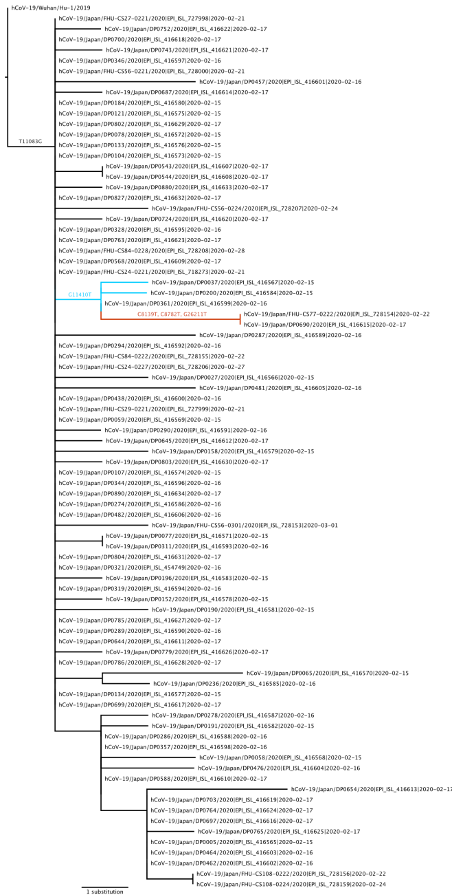
Figure B.2. Maximum likelihood phylogeny of SARS-CoV-2 genomes from the Diamond Princess outbreak. The tree is rooted on Hu-1. Substitutions found in T/T genomes relative to Hu-1 annotated on branches. The G11410T clade is colored blue, with the branch leading to the T/T genomes colored red.
