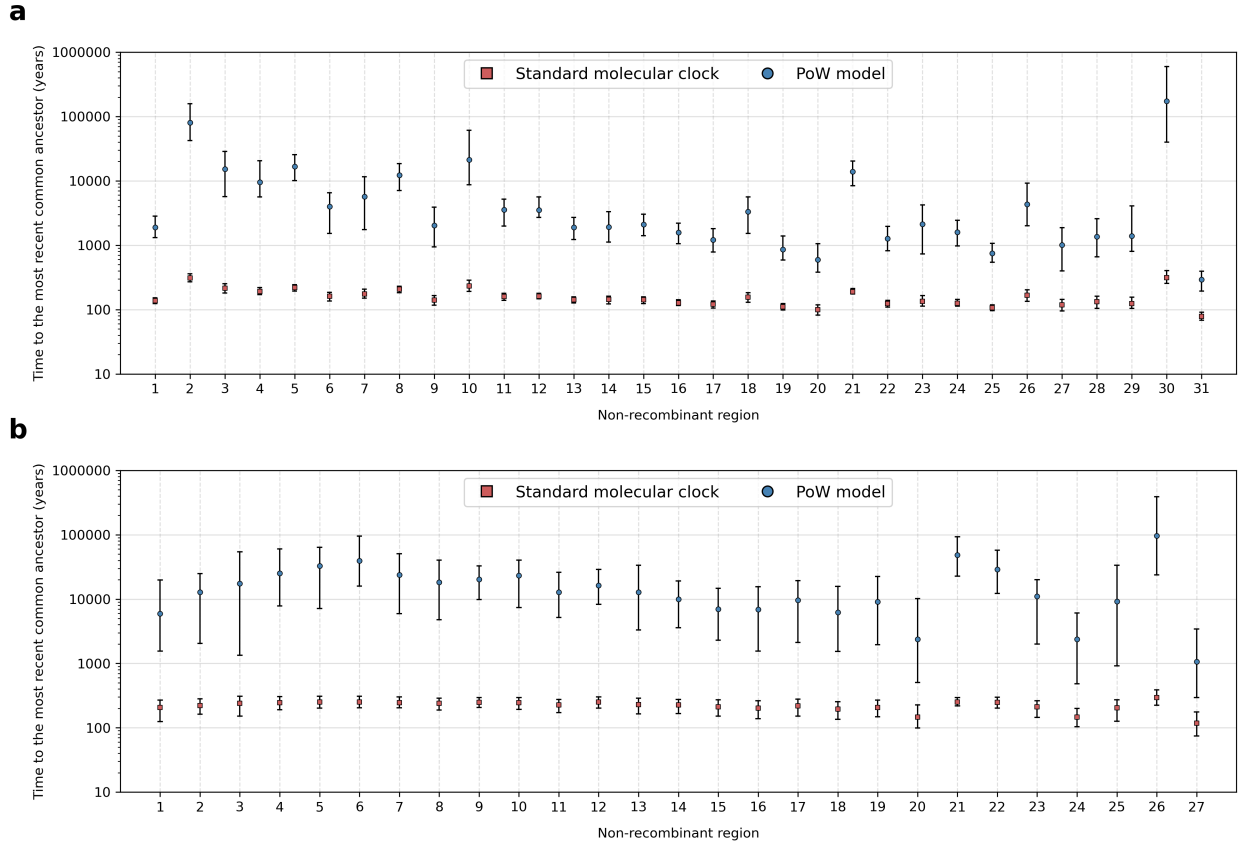
Figure C.8. Time to the most recent common ancestor (tMRCA) after PoW transformation. Estimates of time to the most recent common ancestor for the (a) SARS-CoV-1-like viruses and (b) SARS-CoV-2-like viruses for each NRR when using a standard molecular clock or the PoW model. Each square indicates the median tMRCA and the lines indicate the 95% HPD.
