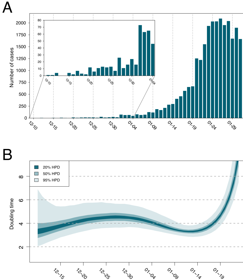
Figure B.21. Growth of the early pandemic. (A) Daily case count after combining the data from the WHO report 26 and Li et al. 23 through January 2020. Inset shows daily case count through 4 January 2020. See Methods for how data were combined. (B) Inferred doubling times of the pandemic in December 2019 and January 2020.
