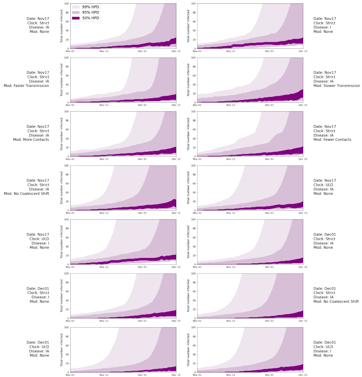
Figure A.11. Robustness analysis for the number of people infected SARS-CoV-2 based on the SAPHIRE model in late 2019. Innermost shading is 50% HPD, middle shading is 95% HPD, and outer shading is 99% HPD. Dates indicates the minimum bound for rejection sampling (Nov 17 or Dec 01). Clock indicates whether the tMRCA was inferred using a strict or relaxed (ULD) clock. Disease denotes which stage of infection in the SAPHIRE model (IA, Ascertained or Unascertained; or I, Ascertained only) must have been reached by the given date for rejection sampling.
