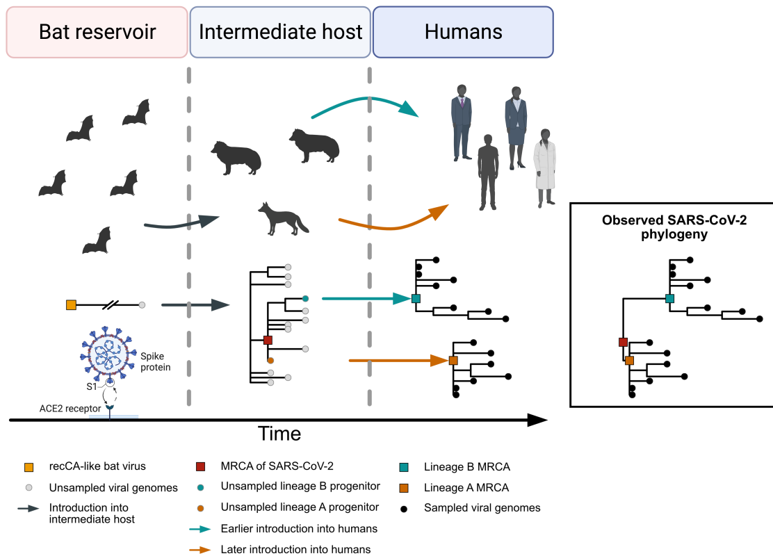
Figure B.30. Schematic depicting the multiple zoonotic origin of SARS-CoV-2. A recCA-like virus was circulating in bats, and likely after gaining the ability to bind ACE2, jumped into an intermediate host. Therein, lineages A and B appeared and were separately introduced into humans shortly thereafter. An example phylogeny of viruses in the intermediate host is depicted, leading to separate phylogenies for lineages A and B. The resulting SARS-CoV-2 phylogeny from the combined lineage A and B viruses is presented in the black box. This scenario depicts a lineage A ancestral haplotype. See Figure B.31 for intermediate and lineage B ancestral haplotypes.
