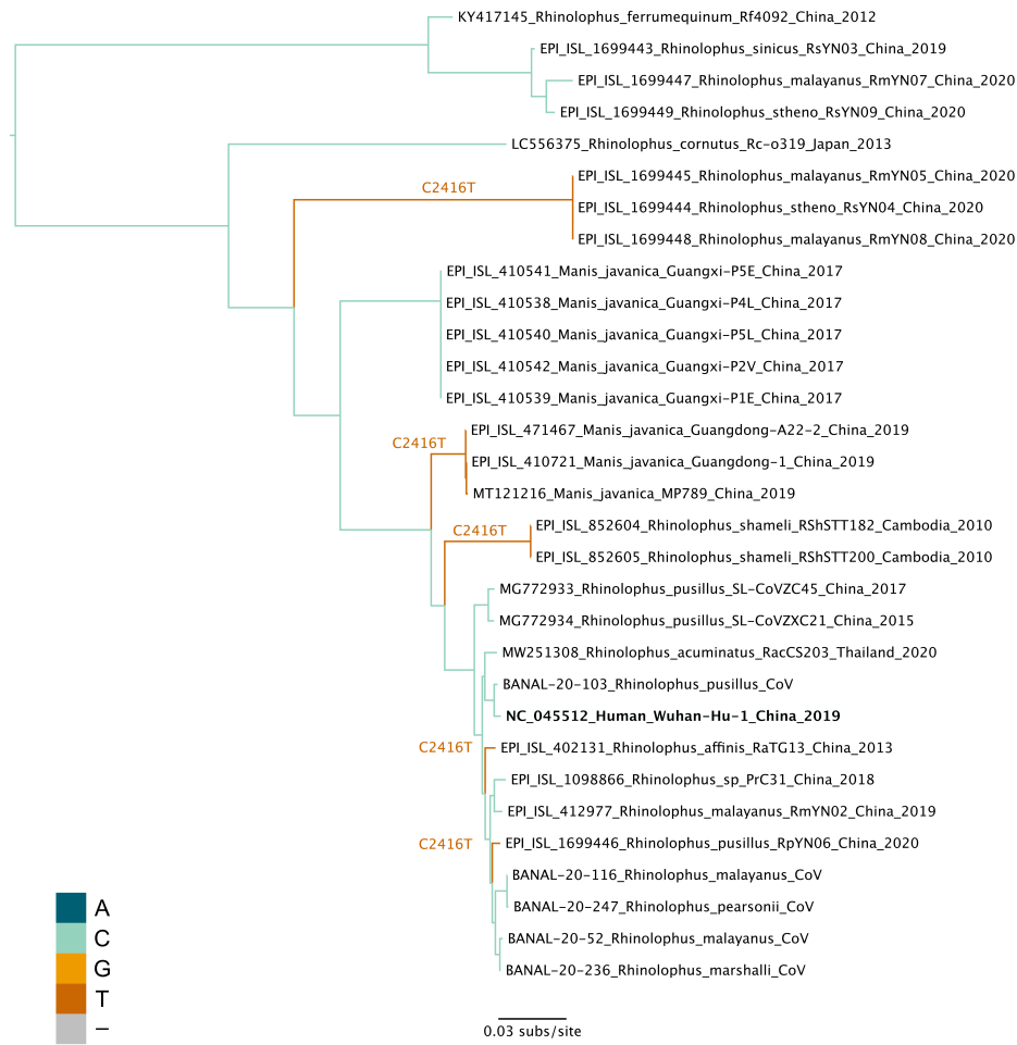
Figure B.8. Maximum likelihood tree of non-recombinant region 2 with branches colored based on the nucleotide at position 2416. Some substitution labels shifted for clarity.
