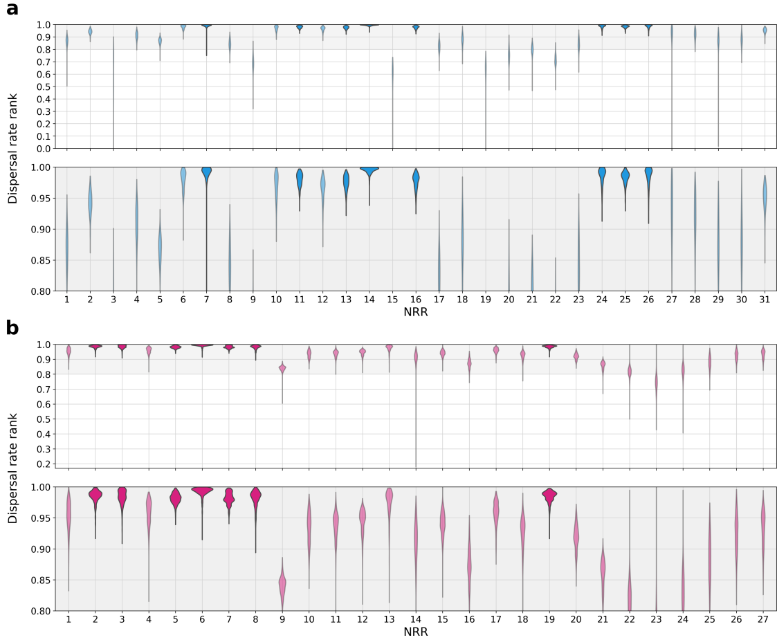
Figure C.18. Ranking of dispersal velocity for the closest-inferred bat virus ancestor to reach the province of emergence. a, The rank for the dispersal velocity necessary to travel from the location of the closest-inferred bat virus ancestor of SARS-CoV-1 from each NRR to the nearest point in Guangdong Province, given the time between emergence and this ancestor and the bat virus dispersal velocities for each NRR. b, The rank for the dispersal velocity necessary to travel from the location of the closest-inferred bat virus ancestor of SARS-CoV-2 from each NRR to the nearest point in Hubei Province, given the time between emergence and this ancestor and the bat virus dispersal velocities for each NRR. The top 20% of the dispersal rate ranks are zoomed-in upon in the lower panels of a and b. Violins are darkened if at least 95% of the dispersal velocity rank posterior is greater than 0.95.
