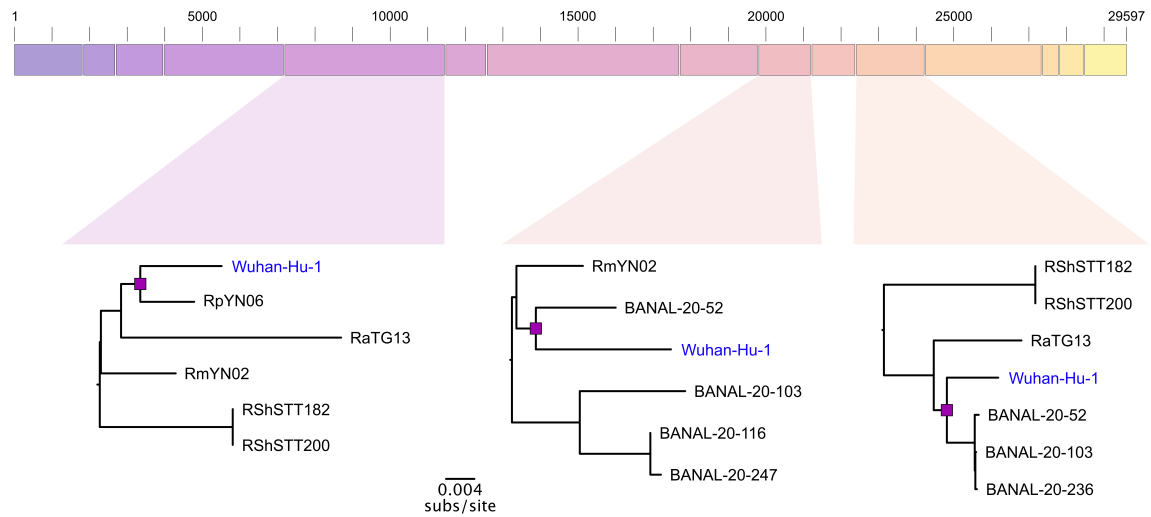
Figure B.6. Reconstructing the recombinant common ancestor (recCA) of SARS-CoV-2 infecting a non-human animal. The figure identifies 15 non-recombinant regions of SARS-CoV-2-like sarbecovirus genomes. Subtrees from sarbecovirus maximum likelihood phylogenies of example regions 5, 9, and 11 show the genomes most closely related to SARS-CoV-2. Ancestral state reconstruction at the MRCA (purple square) of SARS-CoV-2 (Wuhan-Hu-1) and the most closely related sarbecovirus for each of the 15 fragments is concatenated to construct the recCA.
