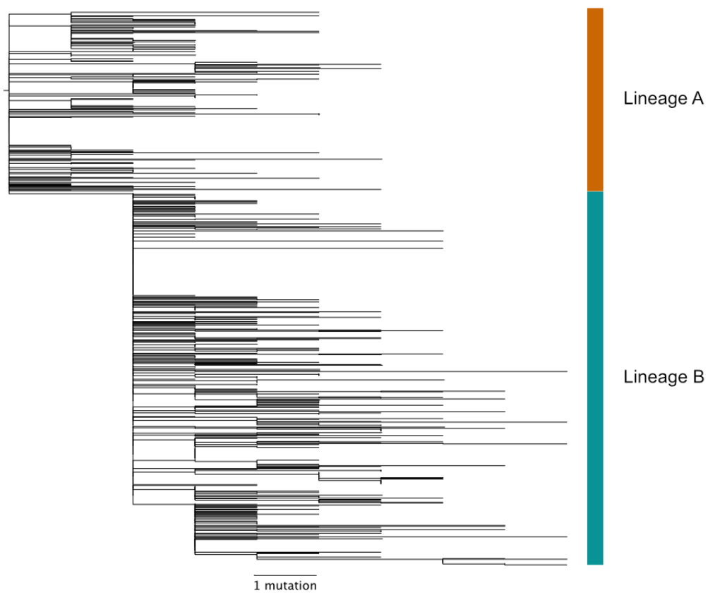
Figure B.19. SARS-CoV-2 maximum likelihood tree rooted on lineage A (n=787 taxa, through 14 February 2020).
