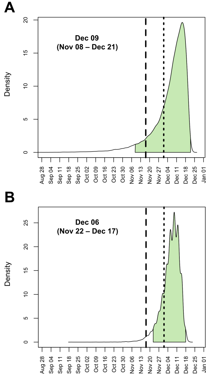
Figure A.1. Posterior distribution for the tMRCA of 583 sampled SARS-CoV-2 genomes circulating in China between December 2019 and April 2020 using (A) a relaxed molecular clock (ULD) and Skyline coalescent prior and (B) a strict clock model and Skygrid coalescent prior. Shaded area denotes 95% HPD. Long-dashed line is 17 November 2019, and short-dashed line is 01 December 2019.
