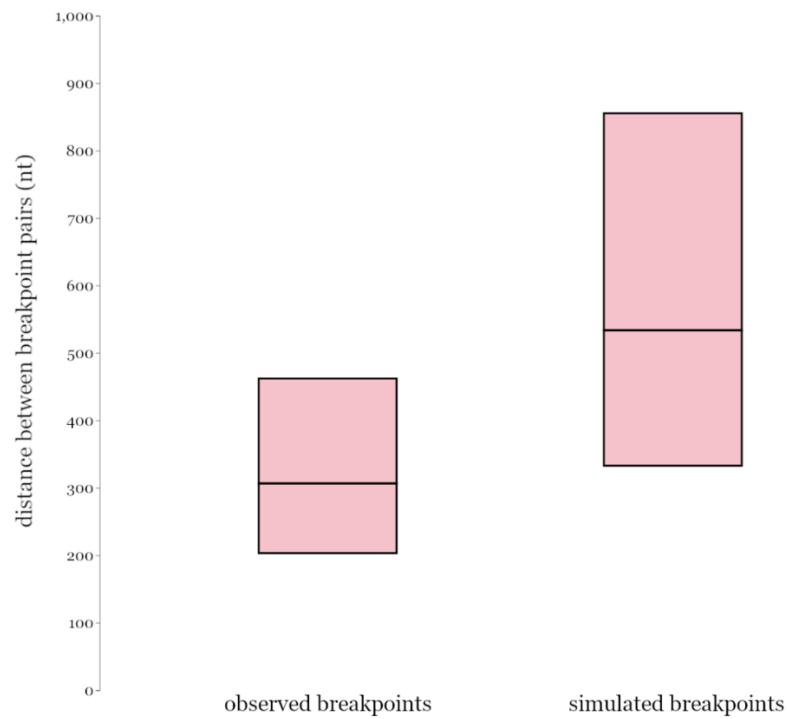
Figure C.3. Mean and 90% confidence intervals of the log-normal breakpoint pair distance distributions for the observed SARS-CoV-1-like and SARS-CoV-2-like estimated breakpoints and the simulated randomly sampled breakpoint sets.
