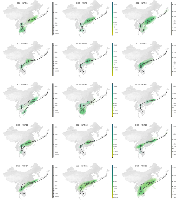
Figure C.11. Continuous phylogeographic reconstruction of the dispersal history of viral lineages for the SARS-CoV-2-like (SC2) viruses. We report the reconstructions obtained for NRRs 1-2 and 4-16 (NRR3 being reported in the main Fig. 3.3h; see Fig. C.12 for NRRs 17-27). For each NRR, we map the maximum clade credibility (MCC) tree whose nodes are coloured from yellow (the time of the most recent common ancestor) to blue (most recent collection date) and are superimposed on 80% HPD polygons coloured according to the same log-transformed time scale and reflecting the uncertainty of the Bayesian phylogeographic inference. HPD polygons were only computed and reported for the last 1,000 years. As in Fig. 3.3g-h, MCC tree tip nodes are displayed as squares (as opposed to dots for internal ones) and dispersal direction (anti-clockwise) of viral lineages is indicated by the edge curvature.
