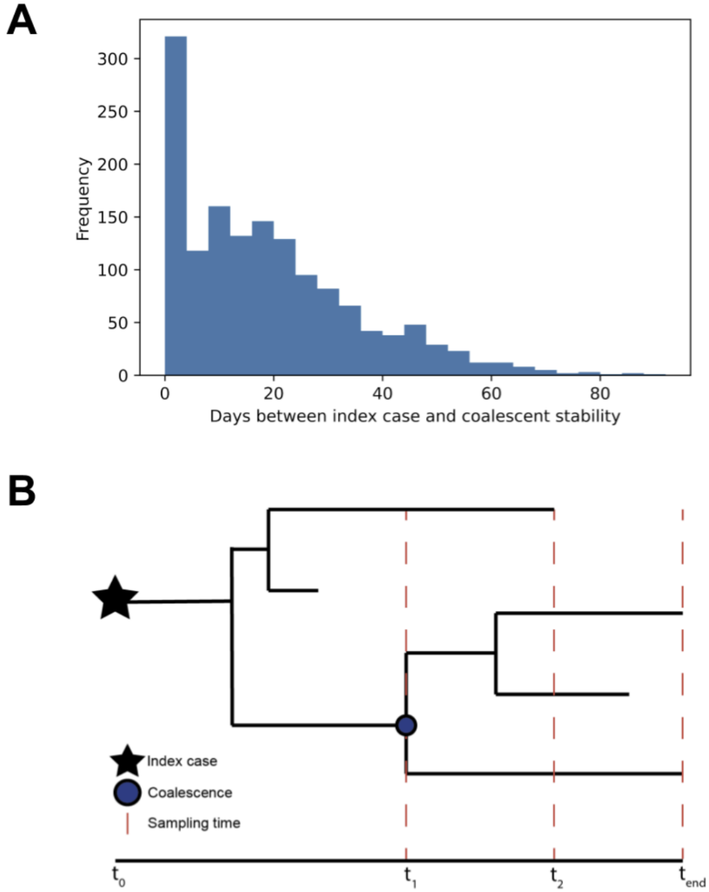
Figure A.16. Stable coalescence in forward compartmental simulations. (A) Days between index case infection and time stable coalescence is achieved in primary simulations. (B) Distinction between the date of index case infection (at t_0 ), the tMRCA of surviving lineages (at t_1 ), and the time at which stable coalescence is achieved when the last basal lineage goes extinct (at t_2 ).
