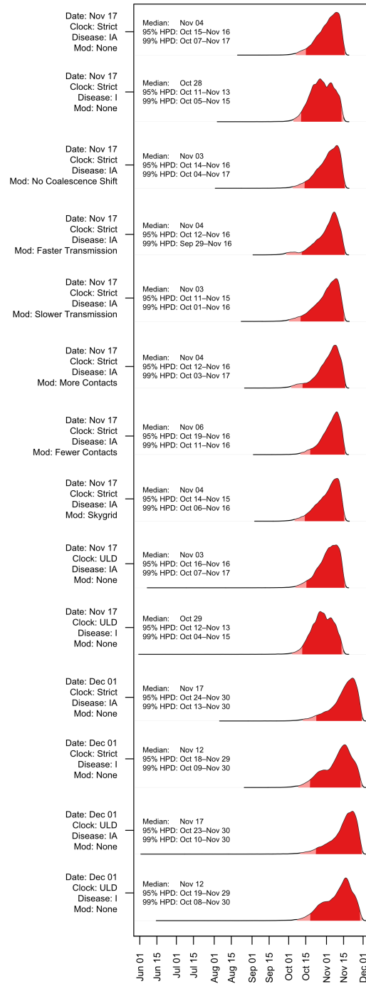
Figure A.7. Robustness analysis for timing of SARS-CoV-2 index case in Hubei province. The 95HPD is shown in dark red, and the 99% HPD is shown in light red. Primary analysis is shown on top. Dates indicates the minimum bound for rejection sampling (Nov 17 or Dec 01). Clock indicates whether the tMRCA was inferred using a strict or relaxed (ULD) clock. Disease denotes which stage of infection in the SAPHIRE model (IA, Ascertained or Unascertained; or I, Ascertained only) must have been reached by the given date for rejection sampling. 'Mod' denotes if any robustness modifications were explored.
