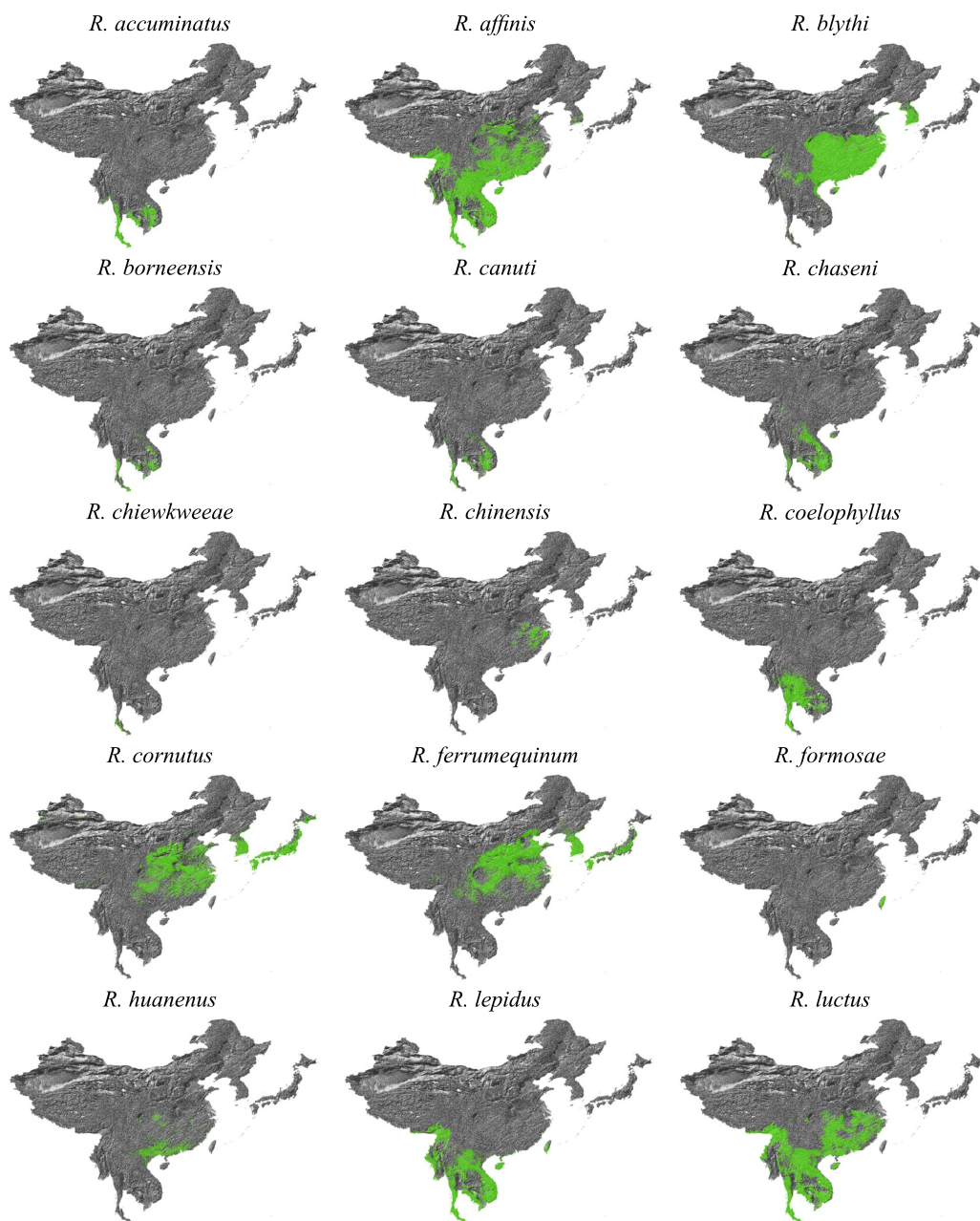
Figure C.13. Distribution maps for species of the Rhinolophus genus, part 1. See Fig. C.14-C.15 for remaining bat distribution maps.
