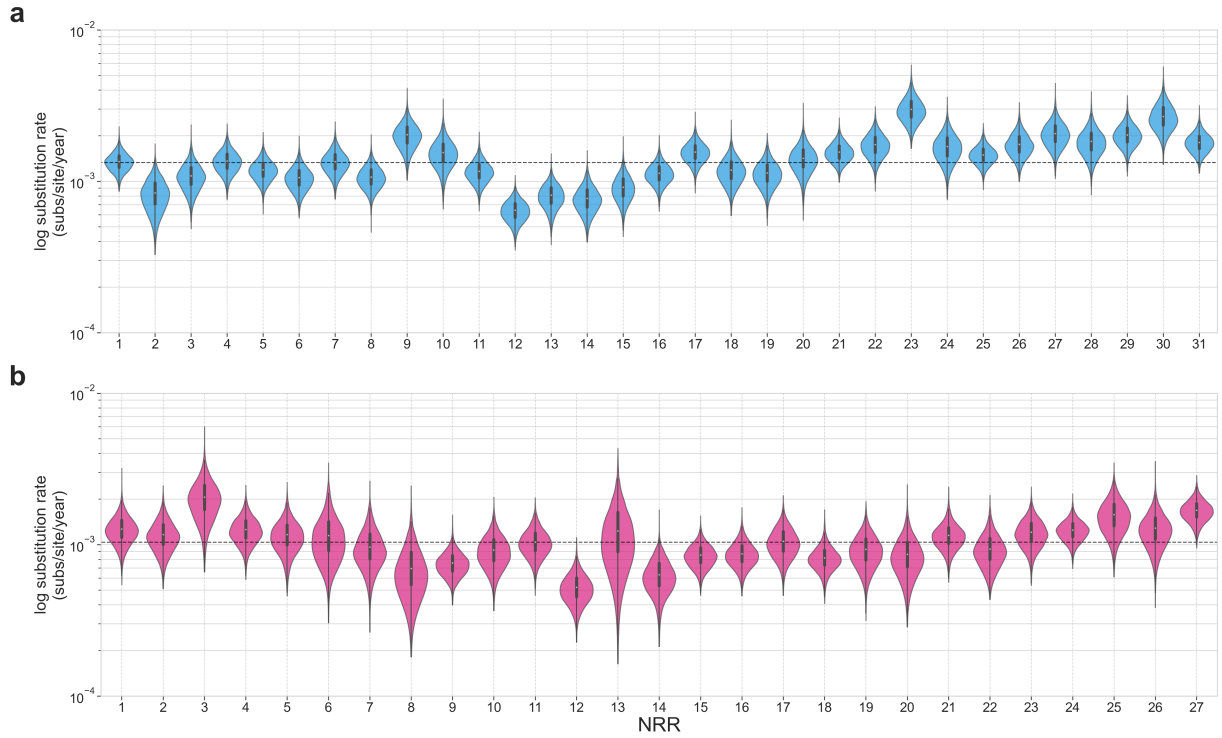
Figure C.4. Substitution rates for the SARS-CoV-1-like and SARS-CoV-2-like viruses. Substitution rates (substitutions/site/year) across the (a) 31 NRRs for the SARS-CoV-1-like viruses and (b) 27 NRRs for the SARS-CoV-2-like viruses. The dashed line in each panel is the respective median substitution rate. The dots and thick lines within the violins indicate the median and interquartile range.
