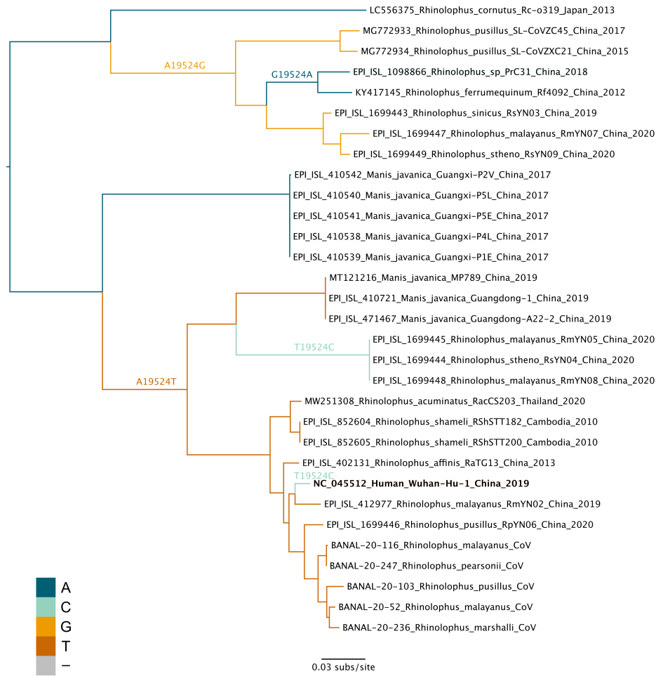
Figure B.9. Maximum likelihood tree of non-recombinant region 8 with branches colored based on the nucleotide at position 19524. Some substitution labels shifted for clarity.
