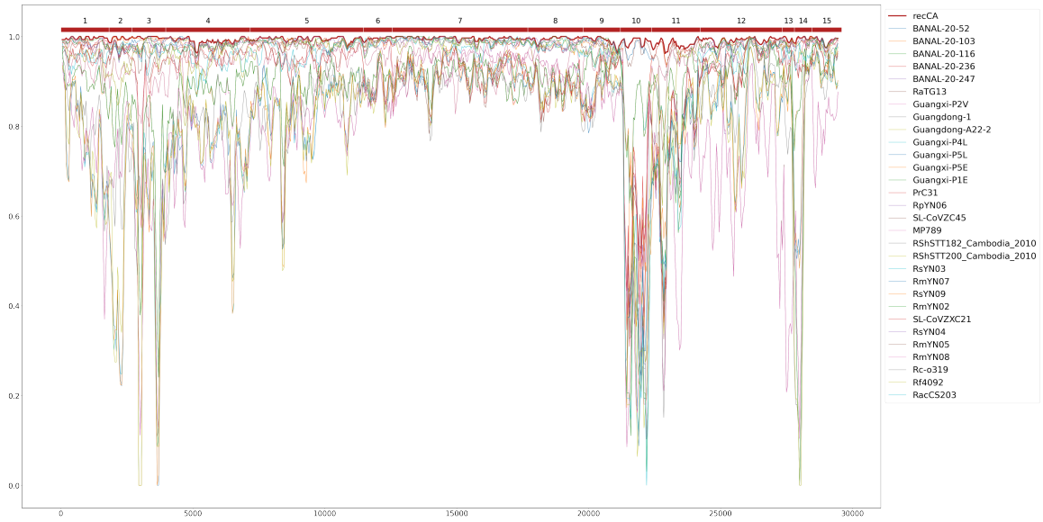
Figure B.7. Simplot of closely related sarbecoviruses and recCA with Hu-1 as the reference.
