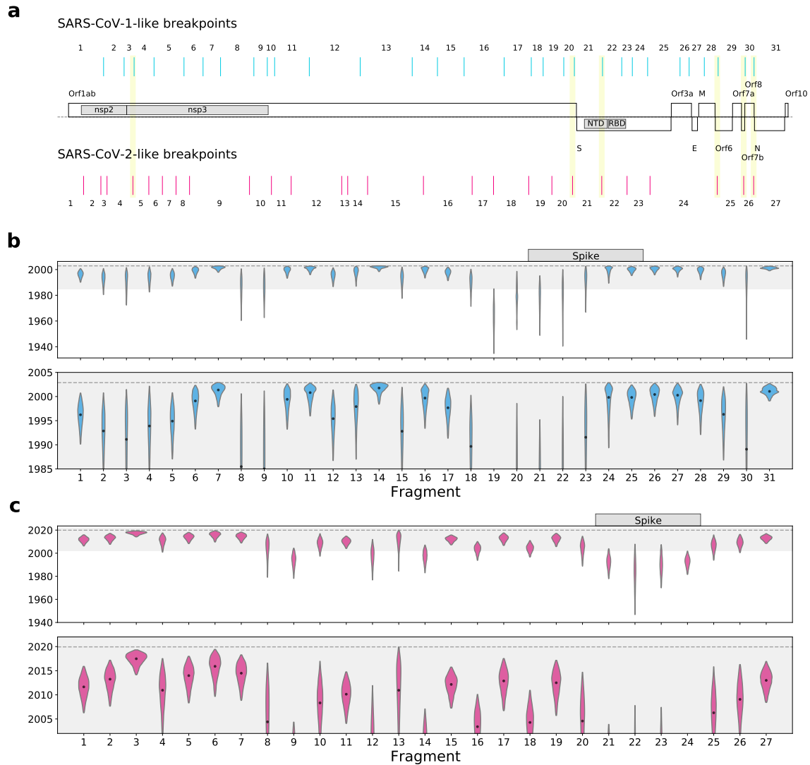
Figure 3.1. Recombination patterns and dating of the closest-inferred bat virus ancestor of SARS-CoV-1 and SARS-CoV-2 for each NRR. a , Distribution of SARS-CoV-1-like and SARS-CoV-2-like breakpoints across the sarbecovirus genome alignment. Schematic of major open-reading frames is displayed in the middle of the figure. Gene domains of interest are also shown within the schematic. Breakpoint pairs with significantly short distances ( \leq 10\% point of distribution) are highlighted in yellow. Numbers indicate NRRs resulting from breakpoints. The alignment is 31,243 nt long. b , Time of the closest-inferred bat virus ancestor of SARS-CoV-1 across the 31 NRRs of the SARS-CoV-1-like viruses. The 20 years before the emergence of SARS-CoV-1 is shown in gray in the upper panel and zoomed-in upon in the lower panel. c , Time of the closest-inferred bat virus ancestor of SARS-CoV-2 across the 27 NRRs of the SARS-CoV-2-like viruses. The 20 years before the emergence of SARS-CoV-2 is shown in gray in the upper panel and zoomed-in upon in the lower panel. The dashed line in each panel is the date of the earliest sampled human case of each SARS-CoV (16 November 2002 for SARS-CoV-1; 24 December 2019 for SARS-CoV-2). The violin plots correspond to the 95% highest posterior density (HPD) intervals and the dot within each violin plot indicates the median. NRRs corresponding to the Spike gene are indicated in the top panels of b-c.
