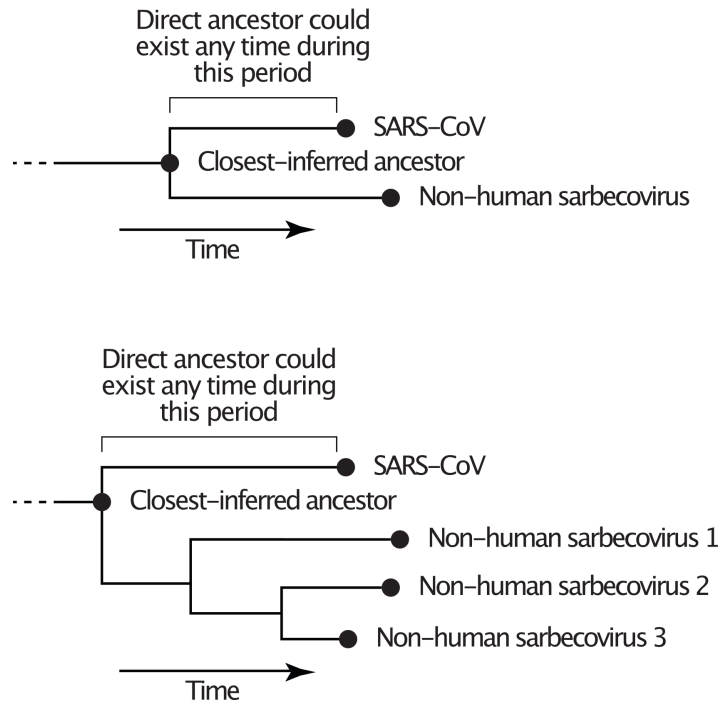
Figure C.1. Schematics illustrating the relationship between a SARS-CoV, the direct ancestor, and the closest-inferred ancestor. The closest-inferred ancestor could be the tMRCA of a given SARS-CoV and one non-human sarbecovirus (top) or the tMRCA of the SARS-CoV and multiple non-human sarbecoviruses (bottom); the closest-inferred ancestor is the parent node of the SARS-CoV. The direct ancestor is the bat sarbecovirus that was involved in each cross-species transmission event leading to the SARS-CoV and could have existed at any point on the branch leading from the closest-inferred ancestor to the SARS-CoV.
