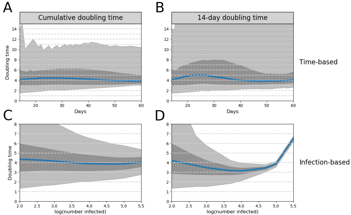
Figure B.22. Inferred doubling times of simulated epidemics. Inferred doubling times of the 1100 primary simulations. (A) Cumulative doubling time since the start of the simulation. (B) 14-day doubling time from day 14 until the end of the simulation, with cumulative doubling time reported prior to day 14. (C) cumulative doubling time once a certain number of individuals are infected (e.g., the cumulative doubling time at the 100th infection). (D) 14-day doubling time once a certain number of individuals are infected, with cumulative doubling time reported if that number of infections occurred before day 14 in the simulation. The center blue line represents the median doubling time across the simulations. Darker and lighter shading represent the 50% and 95% HDI, respectively.
