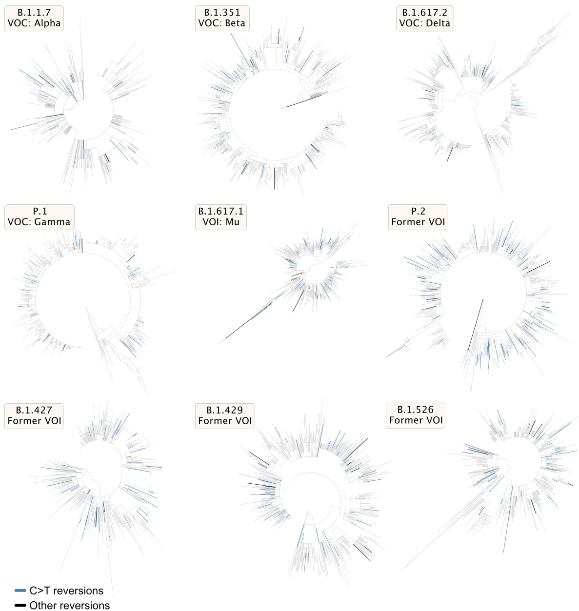
Figure B.15. Maximum likelihood phylogenies of variants of concern (VOC) and variants of interest (VOI) with branches containing reversions colored.
