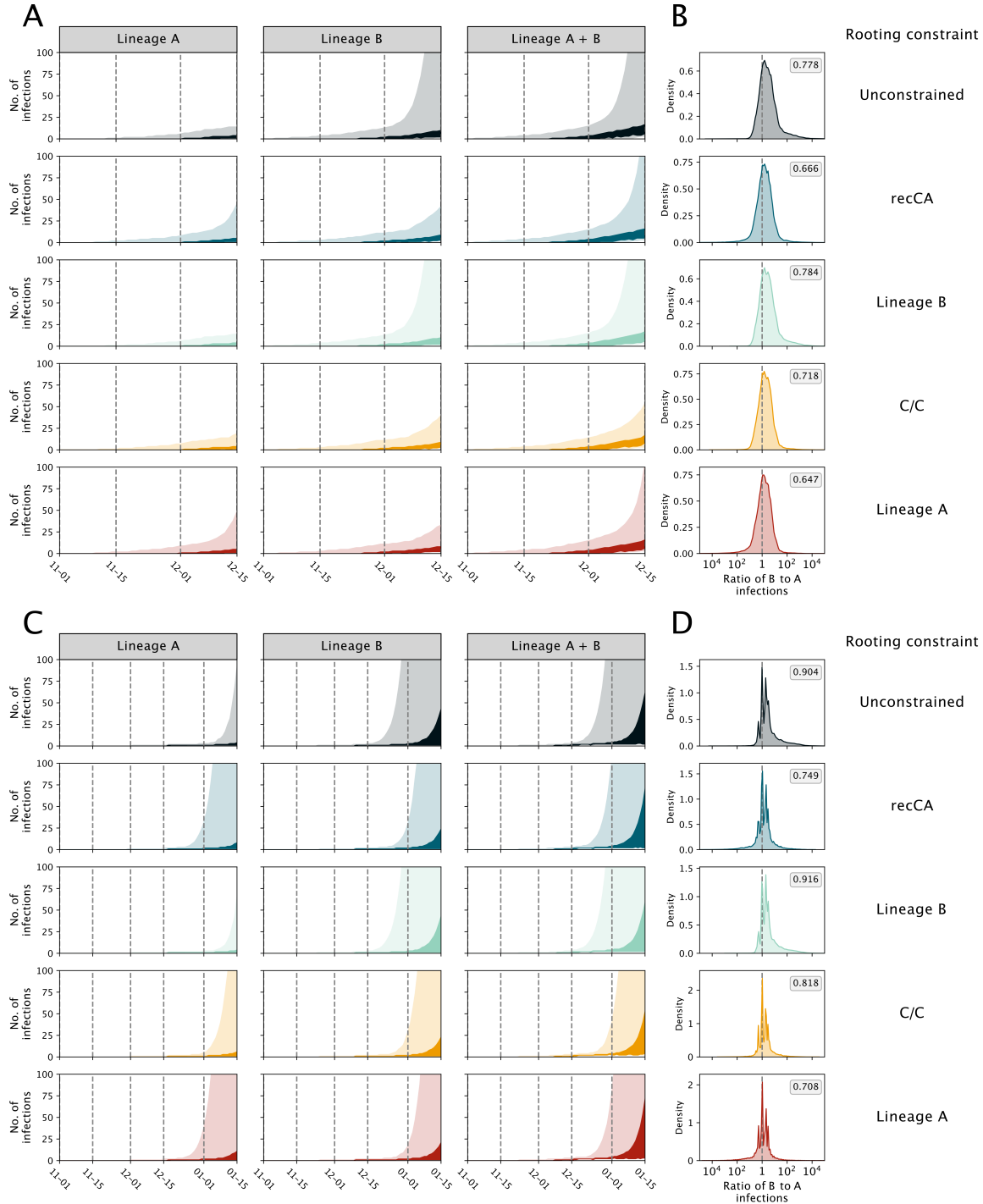
Figure B.27. Dynamics of SARS-CoV-2 resulting from separate introductions of lineages A and B and a shorter doubling time. The simulations used here have a doubling time of 2.65 days (95% HDI: 1.50-4.10). Each row represents a different phylodynamic analysis, with the bottom three representing an enforced ancestral haplotype. (A) Estimated number of infections. The header of each column indicates whether the infections are caused by lineage A, lineage B, or the two lineages combined. Darker and lighter shading represent the 50% and 95% HPD, respectively. (B) The log ratio of lineage B to lineage A infections on 15 December 2019. (C) Estimated number of hospitalizations, with column headers and shading identical to (A). (D) The log ratio of lineage B to lineage A hospitalizations on 1 January 2020. The proportion of the posterior with more lineage B infections or hospitalizations than lineage A in (B, D) is reported in the grey box.
