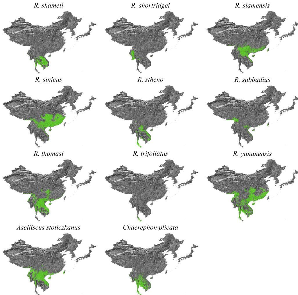
Figure C.15. Distribution maps for species of the Rhinolophus , Ascelliscus , and Chaerephon genera, part 3. Species from the Ascelliscus and Chaerephon genera are limited to those that were hosts to sarbecoviruses in our analyses. See Fig. C.13–C.14 for remaining bat distribution maps.
