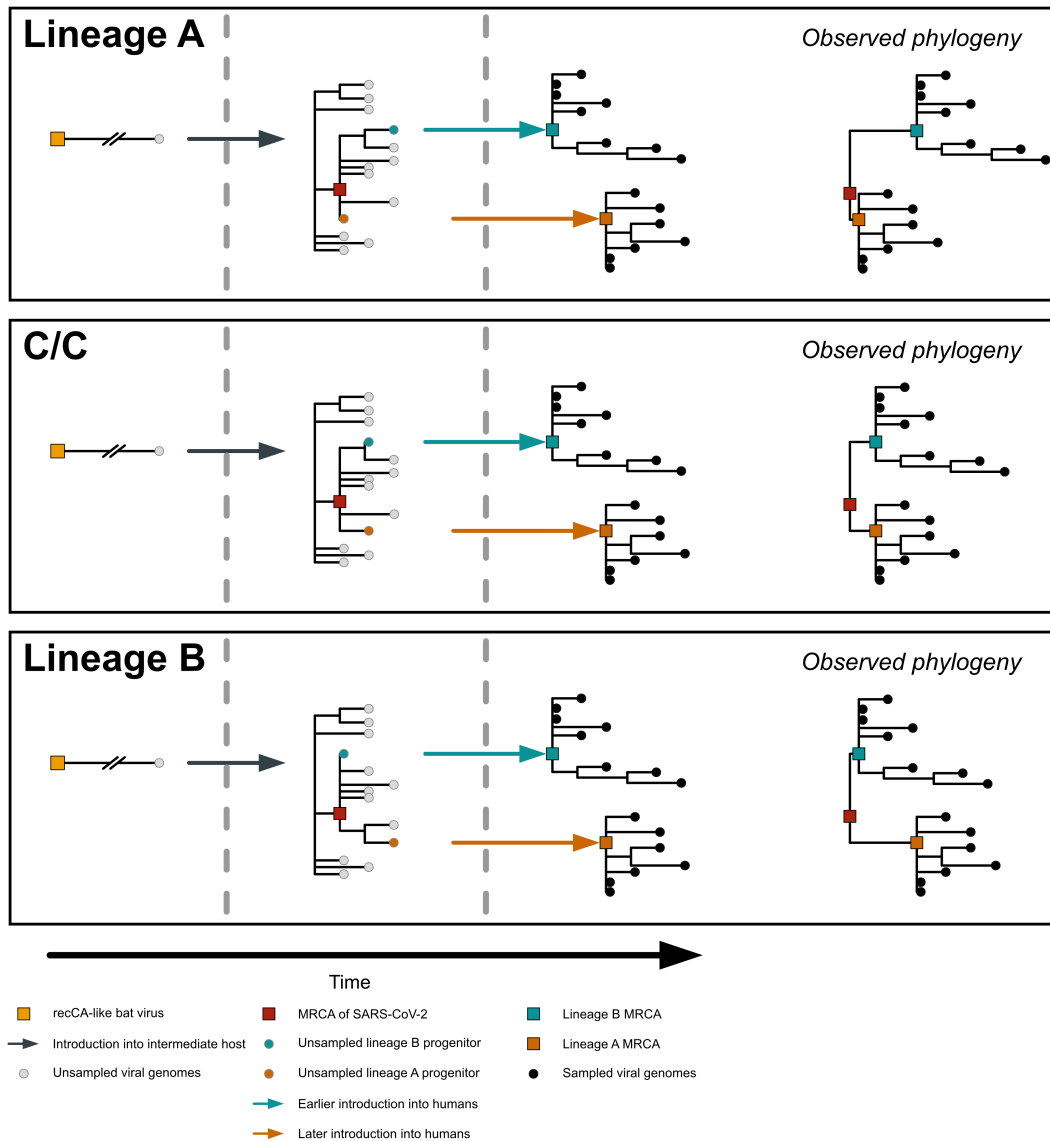
Figure B.31. Rooting orientations of observed SARS-CoV-2 phylogenies resulting from different MRCAs and multiple introductions from the intermediate host. See Figure B.30 for host depictions. The haplotype of the MRCA (red square in the left-center panel) is depicted in the upper left of each box.
