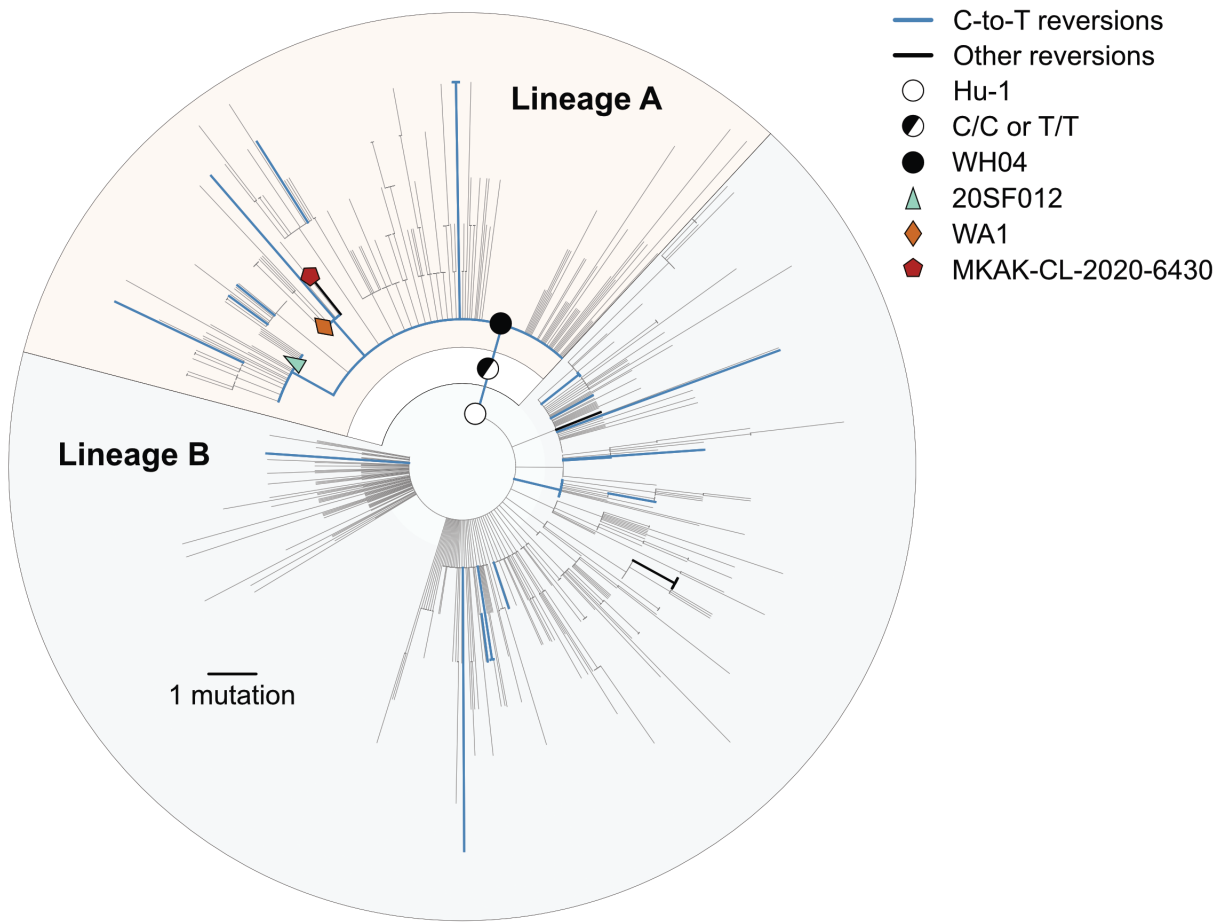
Figure 2.1. Maximum likelihood phylogeny of the early SARS-CoV-2 pandemic, showing nucleotide reversions and putative candidates for the ancestral haplotype at the most common recent ancestor (MRCA). Putative ancestral haplotypes are identified with colored shapes. Reversions from the Hu-1 reference genotype to the recCA are colored. Blue represents C-to-T reversions and black indicates all other reversions. The tree is rooted on Hu-1 to show reversion dynamics to the recCA.
