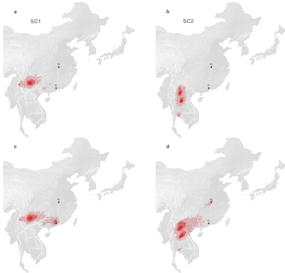
Figure C.17. Comparison of the estimated position of the recCA according to continuous phylogeographic reconstructions that did not consider (a-b) or did consider (c-d) the human and pangolin sequences in the analyses. As in Figure 4g-h, the estimated position of the recCA is based on the continuous phylogeographic reconstruction of all NRRs. We here display the 95%, 75% and 50% HPD regions with an increasing red color darkness. “G.” and “W.” indicate the position of the cities of Guangzhou and Wuhan, respectively.
