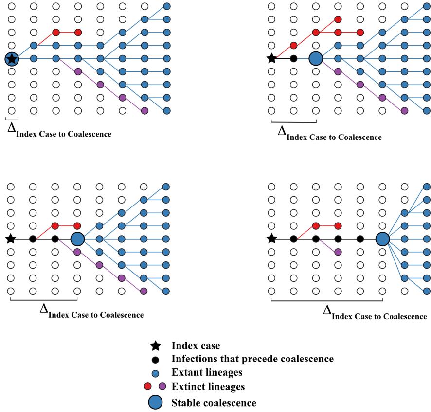
Figure 1.2. Hypothetical coalescent scenarios depicting how the time between index case infection and time of stable coalescence can vary based on stochastic extinction events of basal viral lineages. Coalescence can occur within or contemporaneously with the index case (upper left) or in cases infected later in the course of the epidemic with one (upper right) or more (lower left) basal lineages going extinct. In extreme cases, the epidemic can persist at low levels for a long time before stable coalescence (lower right).
