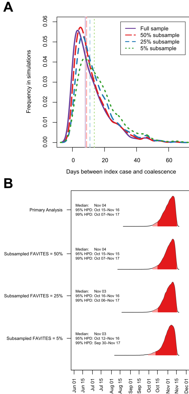
Figure A.17. Impact of subsampling taxa from FAVITES epidemic simulations. (A) Days between index case and stable coalescent with varying amounts of subsampling. (B) Timing of the index case in Hubei province upon subsampling. The primary analysis (from Fig. 1.3C) is shown on top. Inference is conditioned on an ascertained or unascertained case (I or A in SAPHIRE model) by 17 November using a strict clock. The 95% HPD is shown in dark red, and the 99% HPD is shown in light red.
