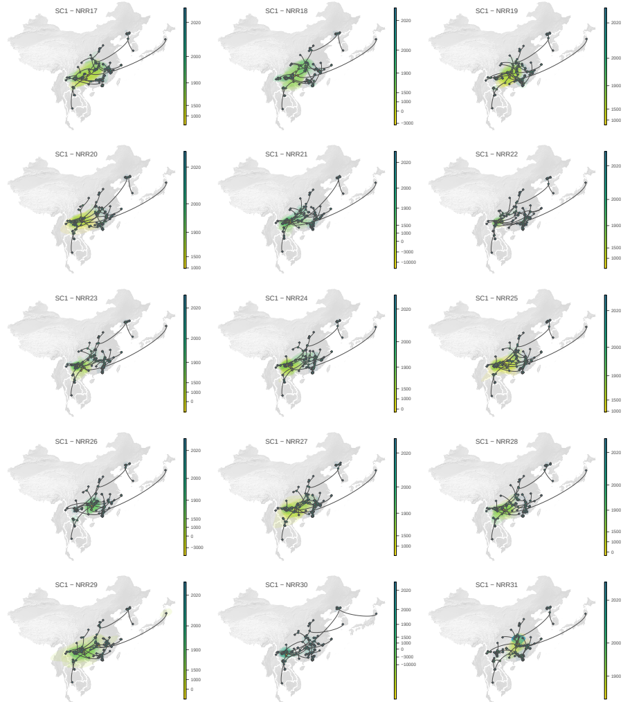
Figure C.10. Continuous phylogeographic reconstruction of the dispersal history of viral lineages for the SARS-CoV-1-like (SC1) viruses. We report the reconstructions obtained for NRRs 17-31 (see Fig. C.9 for NRRs 1-13 and 15-17, NRR14 being reported in the main Fig. 3.3g). For each NRR, we map the maximum clade credibility (MCC) tree whose nodes are coloured from yellow (the time of the most recent common ancestor) to blue (most recent collection date) and are superimposed on 80% HPD polygons coloured according to the same log-transformed time scale and reflecting the uncertainty of the Bayesian phylogeographic inference. HPD polygons were only computed and reported for the last 1,000 years. As in Fig. 3.3g-h, MCC tree tip nodes are displayed as squares (as opposed to dots for internal ones) and dispersal direction (anti-clockwise) of viral lineages is indicated by the edge curvature.
