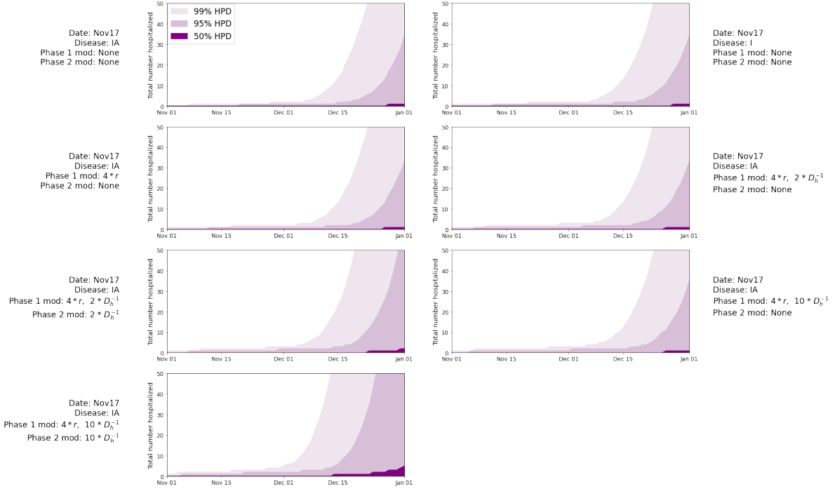
Figure A.14. Number of people hospitalized with SARS-CoV-2 based on the SAPHIRE model in late 2019 using two-phase simulations. Innermost shading is 50% HPD, middle shading is 95% HPD, and outer shading is 99% HPD. Dates indicates the minimum bound for rejection sampling (Nov 17 or Dec 01). Clock indicates whether the tMRCA was inferred using a strict or relaxed (ULD) clock. Disease denotes which stage of infection in the SAPHIRE model (IA, Ascertained or Unascertained; or I, Ascertained only) must have been reached by the given date for rejection sampling. D_h is the average time to hospitalization and r is the ascertainment rate, with the same values as in the primary analysis (Table A.1).
