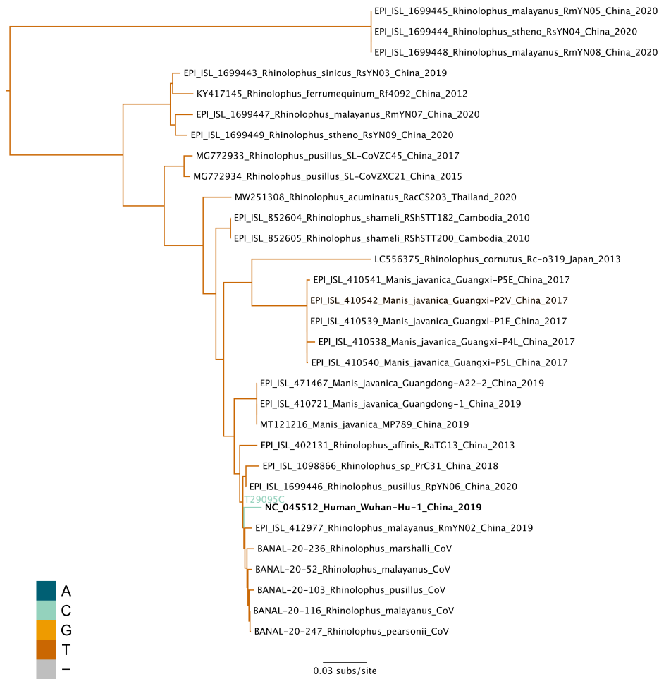
Figure B.14. Maximum likelihood tree of non-recombinant region 15 with branches colored based on the nucleotide at position 29095.
