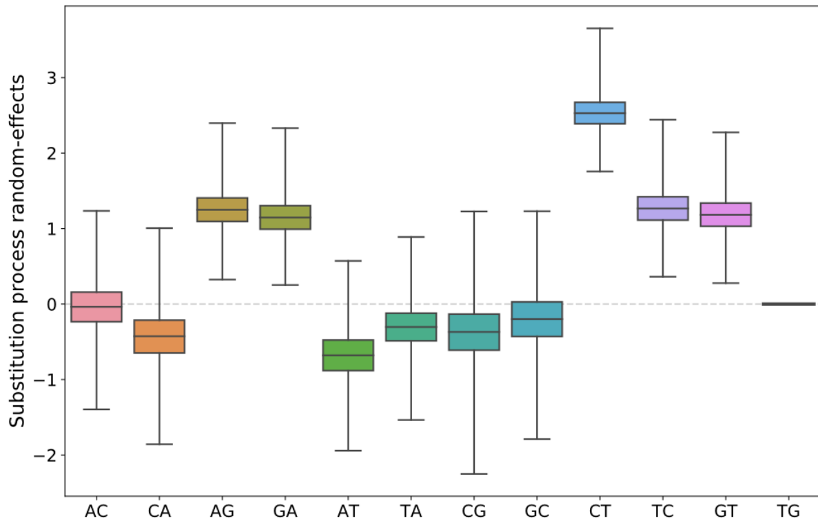
Figure B.17. Substitution process random-effects for the unconstrained rooting model. The random effects for transitions were rescaled with \kappa , and then all random effects were made relative to T-to-G (fixed to 0). The posterior probabilities that e^{C-to-T} > e^{T-to-C} and e^{G-to-T} > e^{T-to-G} is 1.00 for both, indicating the C-to-T transition and G-to-T transversion biases were present in every sample in the posterior.
