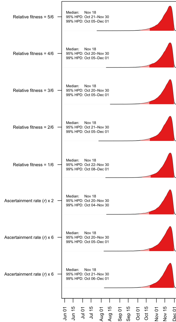
Figure A.18. Impact of relative fitness and virulence of Phase 1 variant on the timing of the index case in Hubei province during two-phase epidemic simulations. The primary two-phase analysis described in the main text (Fig. 1.3F-H) used a relative fitness of 3/6 (or 0.5). Virulence is modulated by the ascertainment rate ( r in the SAPHIRE model). Inference is conditioned on an ascertained or unascertained case (I or A in SAPHIRE model) by 17 November using a strict clock. The 95% HPD is shown in dark red, and the 99% HPD is shown in light red.
