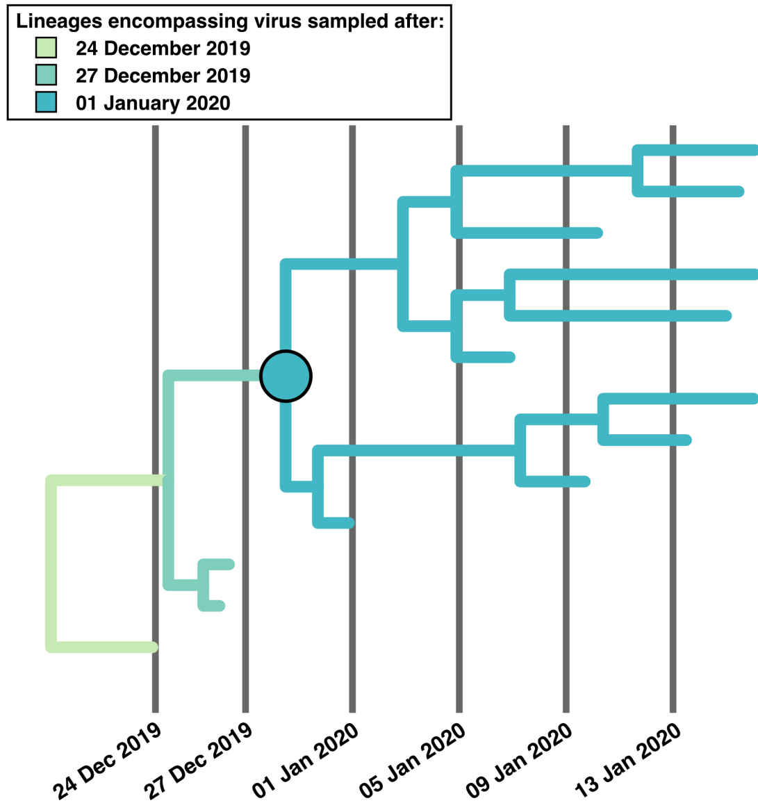
Figure A.2. Example of how coalescence of all sampled genomes can shift forward when analyzing viral genomes sampled in late-December 2019 and January 2020 as basal lineages are lost and cease to propagate. In this example, viruses sampled after 01 January 2020 have a stable tMRCA, indicated by the large circle.
