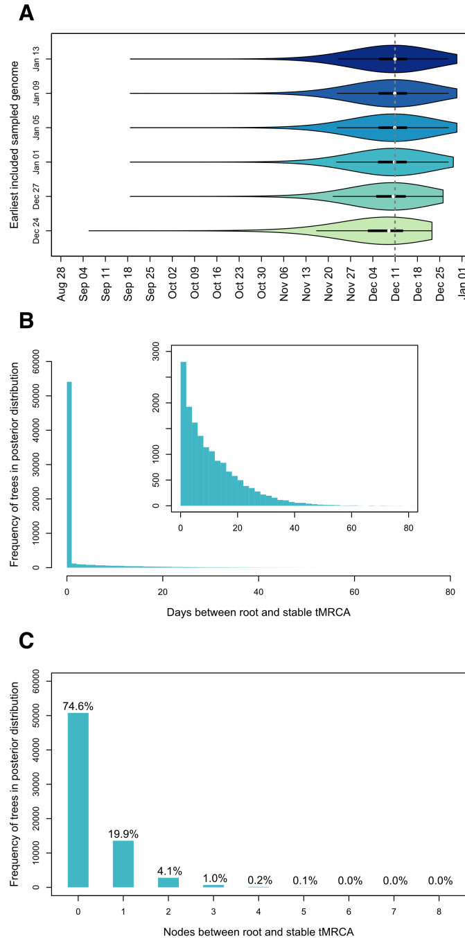
Figure A.3. Shifting of tMRCA in empirical molecular clock analyses. (A) Violin plots of tMRCA estimates upon excluding the earliest sampled genomes between 24 December 2019 and 13 January 2020 (darker colors exclude progressively more early sampled genomes). Mean tMRCA are depicted with white dots. The dashed grey line represents the mean estimate when including only genotypes sampled on 13 January 2020 or later. (B) The number of days between the tMRCA of all genomes (i.e., root) and the tMRCA of genomes sampled on or after 01 January 2020. Inset excludes BEAST samples with <1 day shift. (C) Number of nodes between the tMRCA of all genomes (i.e., root) and the tMRCA of genomes sampled on or after 01 January 2020. Percentage denotes the number of BEAST samples represented in column.
