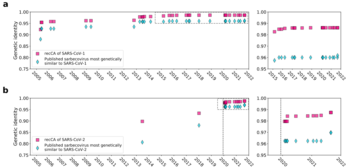
Figure 3.2. The recCA (recombinant common ancestor) and the most closely related sarbecovirus over time. a , The similarity of the recCA of SARS-CoV-1 and the most closely related sarbecovirus in the SARS-CoV-1 viruses to SARS-CoV-1 as a function of time. b , The similarity of the recCA of SARS-CoV-2 and the most closely related sarbecovirus in the SARS-CoV-2 viruses to SARS-CoV-2 as a function of time. The right panels for a and b are zoomed-in panels of the dashed box in the left panels. The dashed vertical line in b is the sampling date of the earliest sampled genome of SARS-CoV-2.
