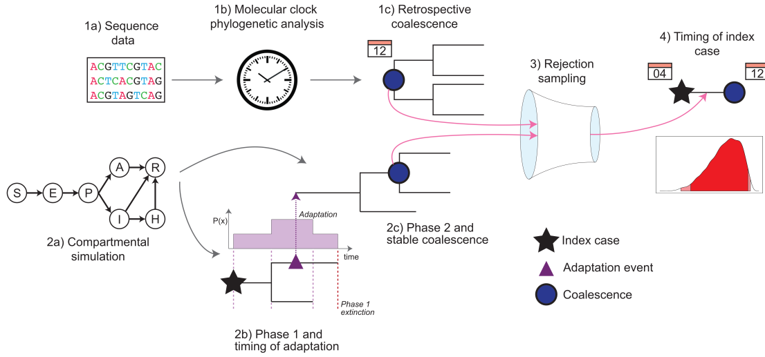
Figure A.9. Combined simulation and phylogenetic workflows to estimate the timing of the Hubei index case in a two-phase epidemic. (1a) Using sequence and epidemiological data, (1b) BEAST performs a phylodynamic molecular clock analysis to (1c) determine the tMRCA. (2a) FAVITES simulates the epidemic in Hubei using a SAPHIRE compartmental model, (2b) estimates a prior distribution for the length of Phase 1 of the epidemic, and (2c) estimates a prior distribution for the time from adaptation to the stable coalescence for Phase 2 of the epidemic. The timing of adaptation (2b) is calculated based on the number of circulating lineages at a given time in Phase 1 (see Methods). The results of (1) and (2) are combined via rejection sampling (3; Fig. A.6) to (4) determine the timing of the index case and its posterior distribution.
