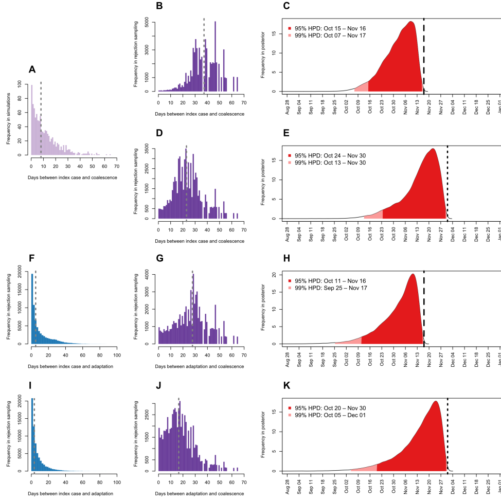
Figure 1.3. Forward simulations estimating the timing of the index case in Hubei province. (A) Days between index case infection and stable coalescence in forward compartmental epidemic simulations ( n=1000 ). (B) Days between index case infection and stable coalescence after rejection sampling and (C) posterior distribution for date of index case infection, conditioned on an ascertained case by 17 November 2019 denoted by long-dashed line. (D-E) Epidemic simulation, conditioned on an ascertained case by 01 December 2019 denoted by short-dashed line. Two-phase epidemic (F) days between index case carrying less fit variant and adaptation ( n=2000 ), (G) days between adaptation and stable coalescence ( n=1000 ), and (H) posterior distribution for date of index case infection, conditioned on an ascertained case by 17 November 2019. (I-K) Two-phase epidemic conditioned on an ascertained case by 01 December 2019. Grey dashed lines indicate median estimates.
