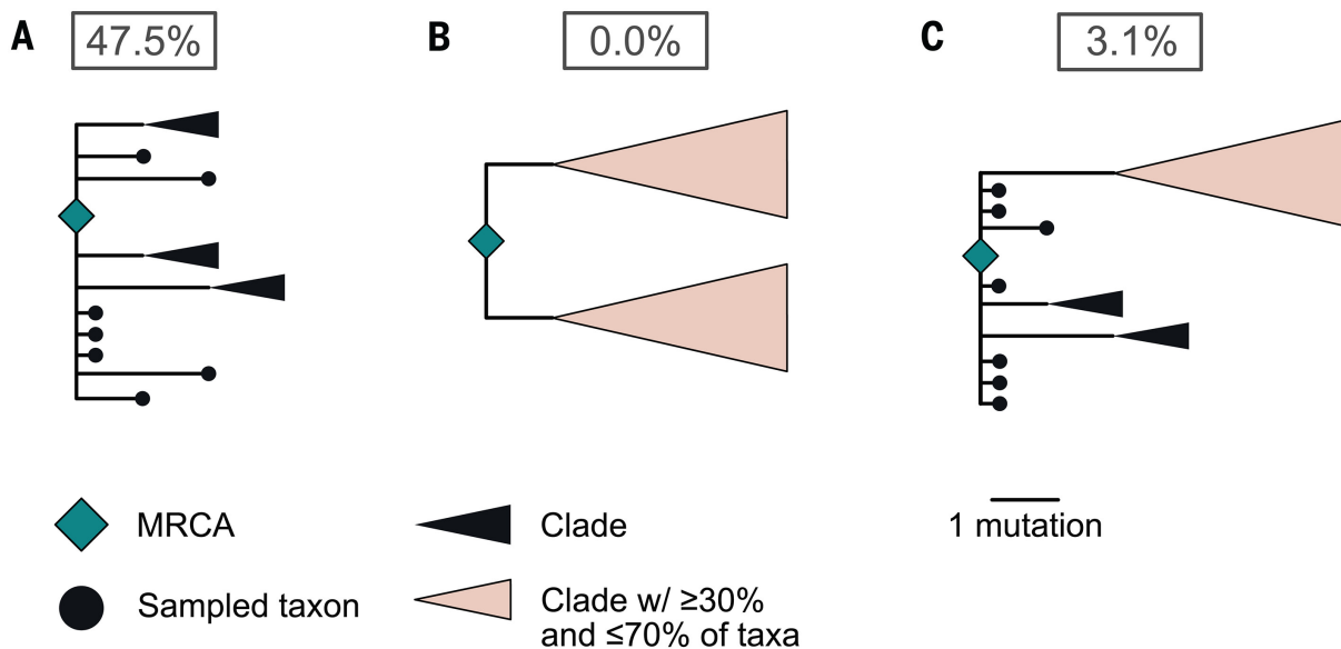
Figure 2.2. Probability of phylogenetic structures arising from a single introduction of SARS-CoV-2 in epidemic simulations. (A) A large polytomy of at least 100 descendent lineages, consistent with the base of both lineages A and B. (B) Topology matching a C/C ancestral haplotype: two clades each one mutation from the ancestor, both with polytomies of at least 100 descendent lineages. (C) Topology matching either a lineage A or lineage B ancestral haplotype: a basal polytomy with at least 100 descendent lineages including a large clade separated by two mutations, also possessing a polytomy of at least 100 descendent lineages. Basal taxa have short branch lengths for clarity. The probability of each phylogenetic structure after a single introduction is reported in the respective boxes.
