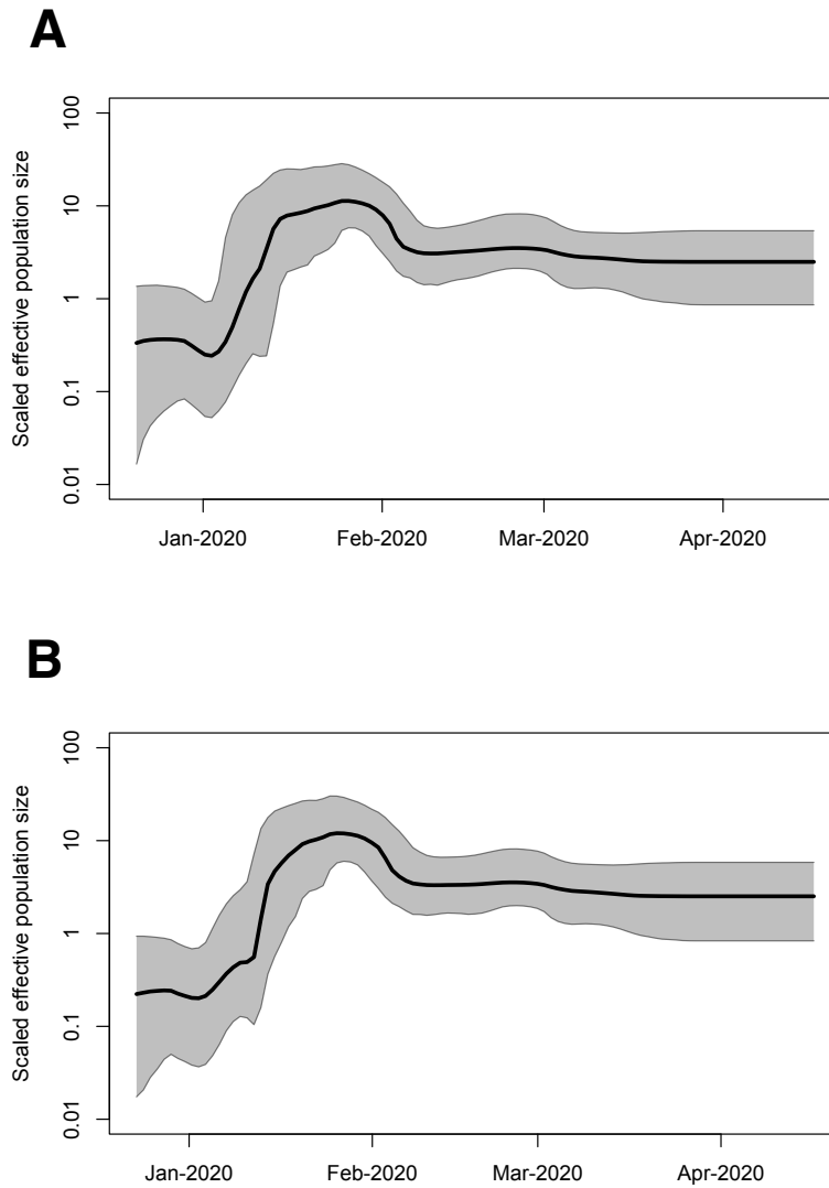
Figure A.15. Bayesian skyline plot reconstruction. (A) Strict molecular clock analysis and (B) ULD relaxed molecular clock. Solid line is the median estimate. Shaded area is the 95% HPD.
