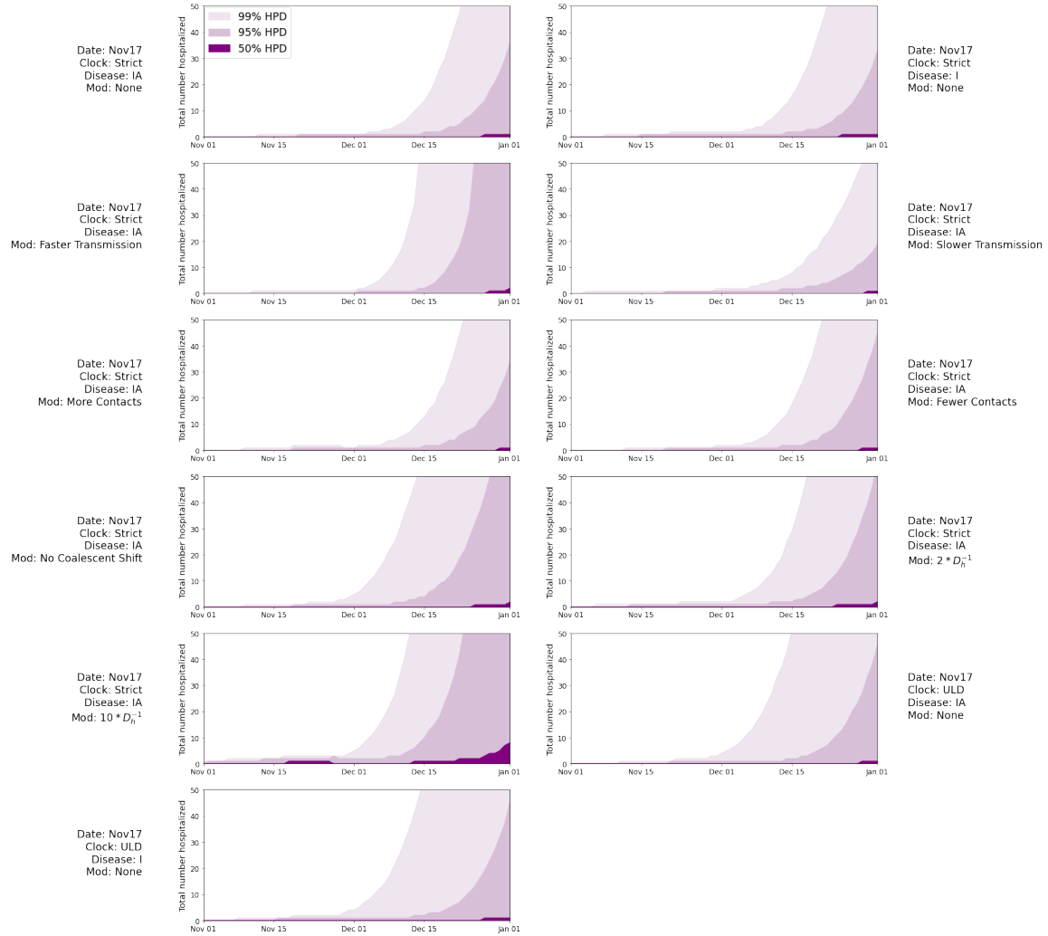
Figure A.13. Number of people hospitalized with SARS-CoV-2 based on the SAPHIRE model in late 2019. Innermost shading is 50% HPD, middle shading is 95% HPD, and outer shading is 99% HPD. Dates indicates the minimum bound for rejection sampling (Nov 17 or Dec 01). Clock indicates whether the tMRCA was inferred using a strict or relaxed (ULD) clock. Disease denotes which stage of infection in the SAPHIRE model (IA, Ascertained or Unascertained; or I, Ascertained only) must have been reached by the given date for rejection sampling.
