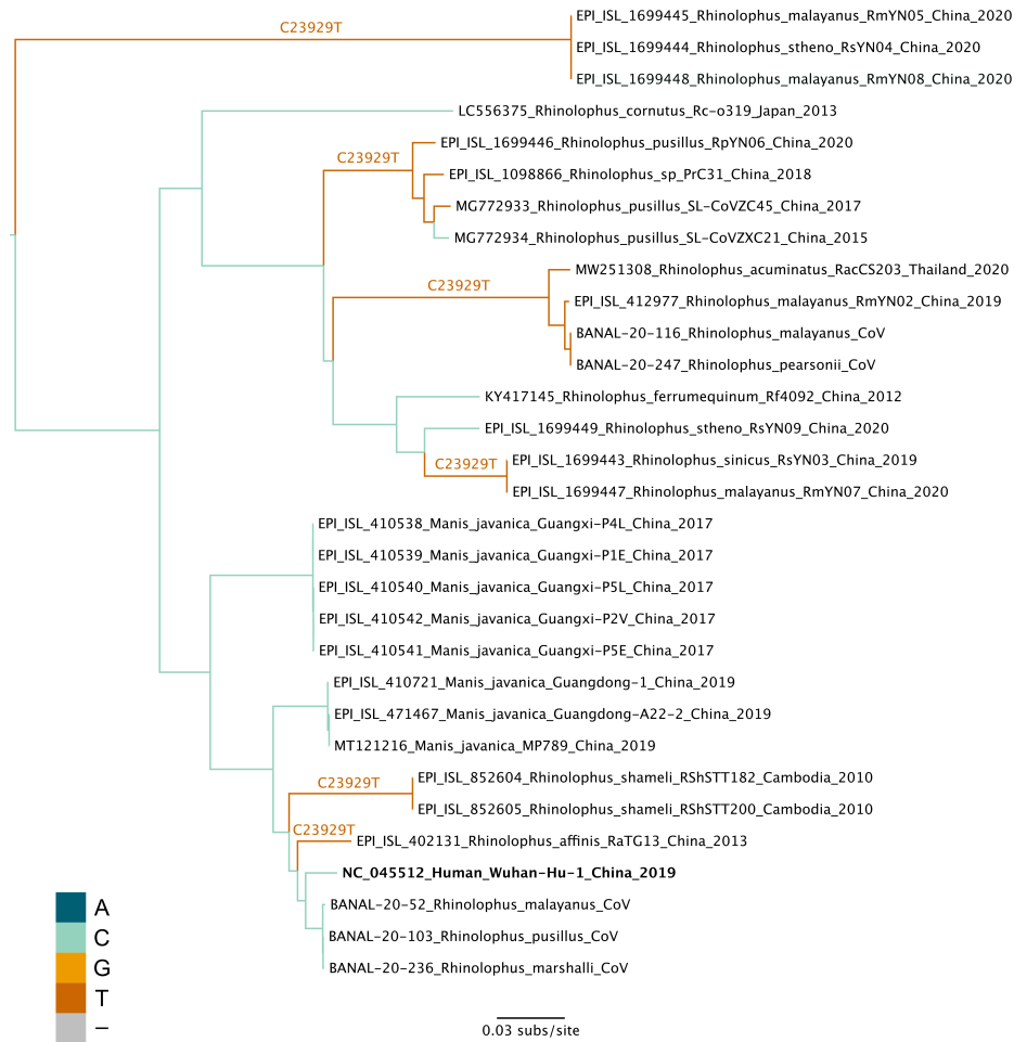
Figure B.10. Maximum likelihood tree of non-recombinant region 11 with branches colored based on the nucleotide at position 23929. Some substitution labels shifted for clarity.
