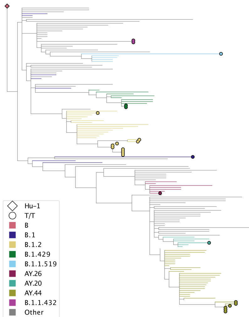
Figure B.4. Subtree showing the placement of T/T genomes in the San Diego SEARCH dataset. 24 T/T genomes were placed on a global tree of 3 million genomes (v2022-01-21) using UShER. The node branches are colored by the assigned PANGO lineage. The T/T genomes are highlighted using circles.
