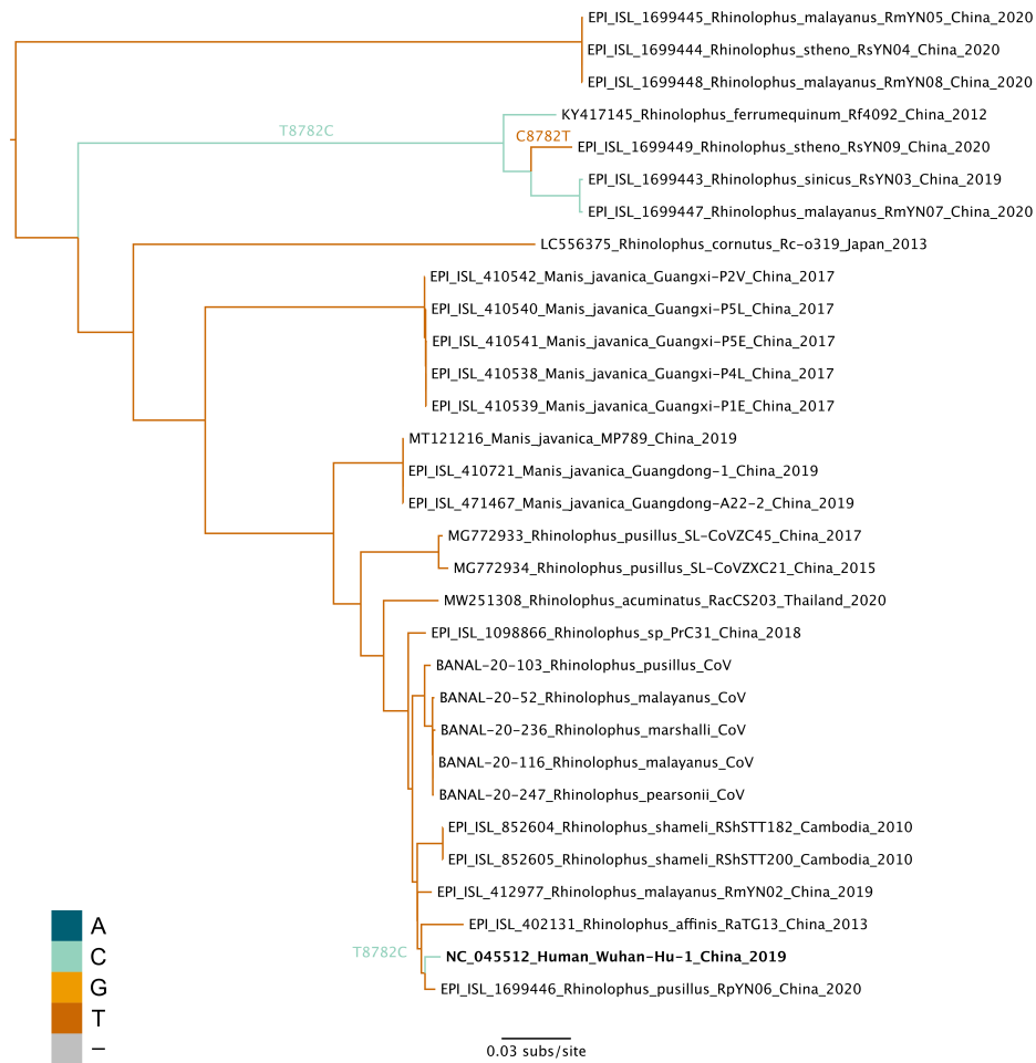
Figure B.11. Maximum likelihood tree of non-recombinant region 5 with branches colored based on the nucleotide at position 8782. Some substitution labels shifted for clarity.
