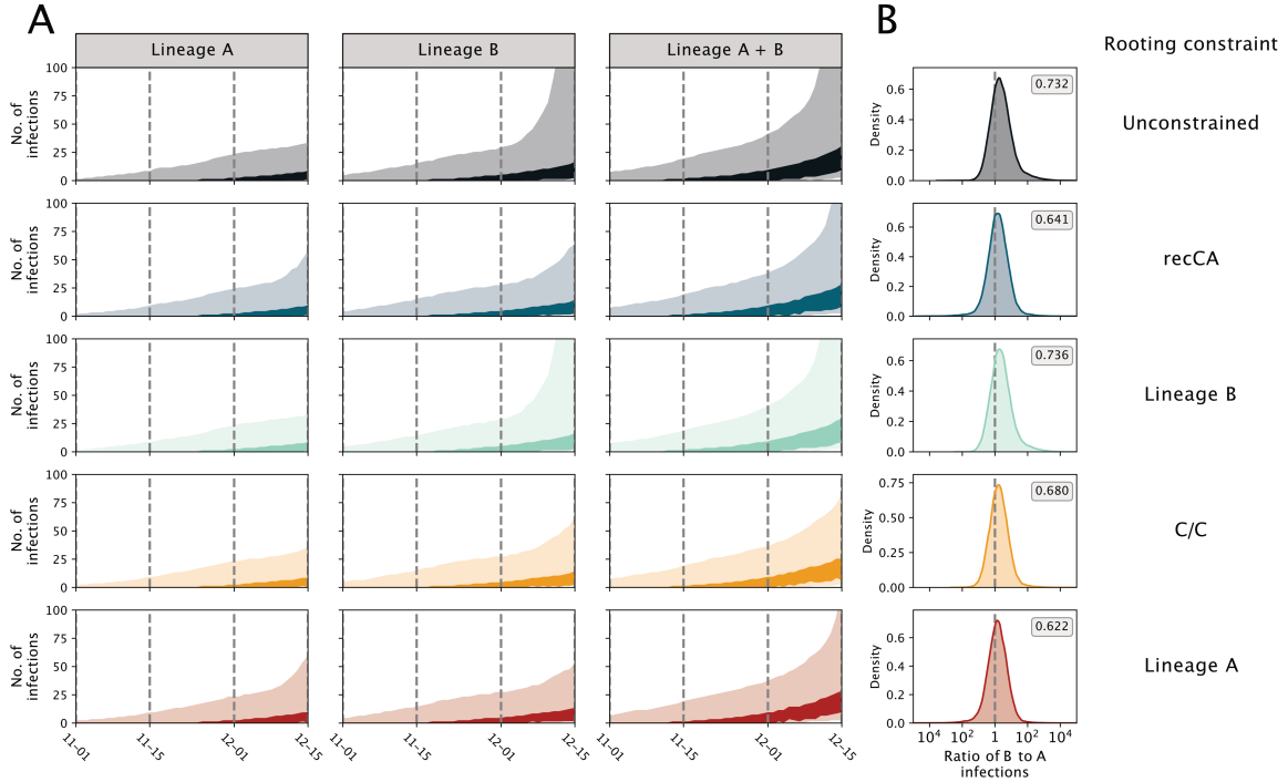
Figure 2.4. Dynamics of simulated SARS-CoV-2 epidemics resulting from separate introductions of lineages A and B. Each row represents a different rooting constraint in phylodynamic analysis, with the bottom three representing a fixed ancestral haplotype. (A) Estimated number of infections. The header of each column indicates whether the number of infections are caused by lineage A, lineage B, or the two lineages combined. Darker and lighter shading represent the 50% and 95% HPD, respectively. (B) The log ratio of lineage B to lineage A infections on 15 December 2019. Posterior probability of having more lineage B infections than lineage A reported in the grey box.
