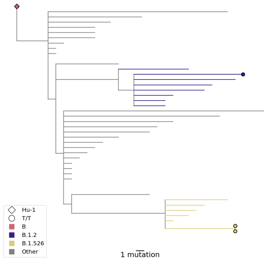
Figure B.3. Subtree showing the placement of T/T genomes in the NYC Public Health Laboratories dataset. 3 T/T genomes were placed on a global tree of 3 million genomes (v2022-01-21) using UShER. The node branches are colored by the assigned PANGO lineage. The T/T genomes are highlighted using circles.
