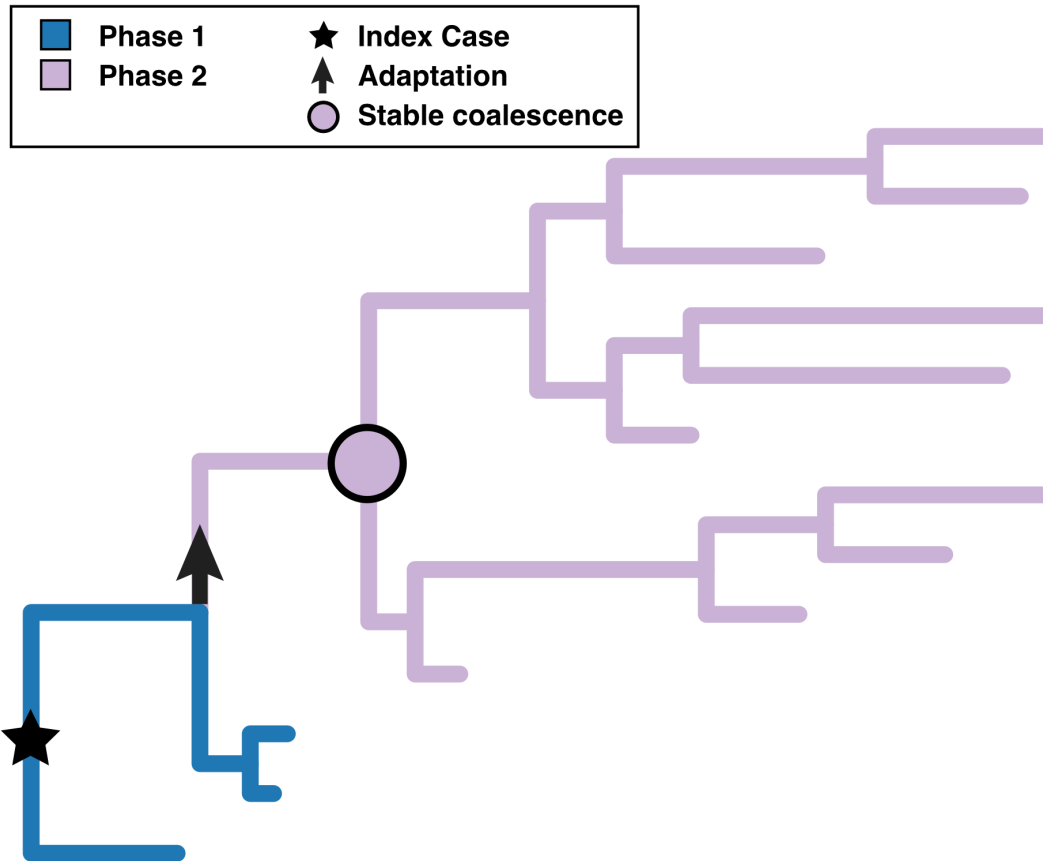
Figure A.8. Example phylogeny of the two-phase epidemic simulations. The index case occurs during Phase 1, characterized by a less-fit viral variant (shown in blue). At some point before Phase 1 goes extinct, an adapted variant arises (arrow), giving rise to Phase 2, characterized by the variant observed in Hubei province (shown in light purple). The stable coalescence (circle) occurs during Phase 2.
