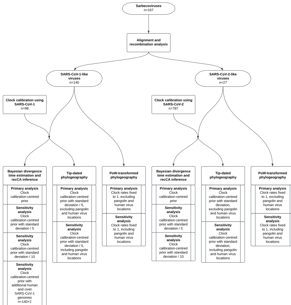
Figure C.2. Workflow to perform phylogenetic and phylogeographic analyses. Starting with 167 sarbecovirus genomes, we align and perform recombination analysis to determine the number of SARS-CoV-1-like and SARS-CoV-2-like viruses and their corresponding NRRs for subsequent analyses. We then calibrate the molecular clock for SARS-CoV-1-like viruses and SARS-CoV-2-like viruses using SARS-CoV-1 genomes and SARS-CoV-2 genomes (these datasets are separate from the SARS-CoV-1-like viruses and SARS-CoV-2-like viruses), respectively. Finally, we perform Bayesian divergence time estimation, recCA inference, and phylogeography analyses, each of which comprised both primary and sensitivity analyses. Ovals indicate the number of sarbecovirus genomes included in subsequent steps. Rectangles without inner vertical lines indicate analyses performed; rectangles with inner vertical lines indicate primary versus sensitivity analyses, with non-bolded text describing the details of the analysis performed.
