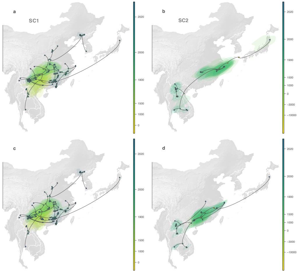
Figure C.16. Comparison of the continuous phylogeographic reconstructions for two selected NRRSs (NRR14 for SARS-CoV-1-like viruses [SC1] on the left, and NRR3 for SARS-CoV-2-like viruses [SC2] on the right) when not considering (a-b) or when considering (c-d) the human and pangolin sequences in the analyses. Comparison of the continuous phylogeographic reconstructions for two selected NRRSs (NRR14 for SARS-CoV-1-like viruses [SC1] on the left, and NRR3 for SARS-CoV-2-like viruses [SC2] on the right) when not considering (a-b) or when considering (c-d) the human and pangolin sequences in the analyses. For each reconstruction, we map the corresponding MCC tree whose nodes are coloured from yellow (the time of the most recent common ancestor) to blue (most recent collection date) and are superimposed on 80% HPD polygons coloured according to a log-transformed time scale and reflecting the uncertainty of the Bayesian phylogeographic inference. HPD polygons were only computed and reported for the last 1,000 years. As in Fig. 3.3g-h, MCC tree tip nodes are displayed as squares (as opposed to dots for internal ones) and dispersal direction (anti-clockwise) of viral lineages is indicated by the edge curvature.
