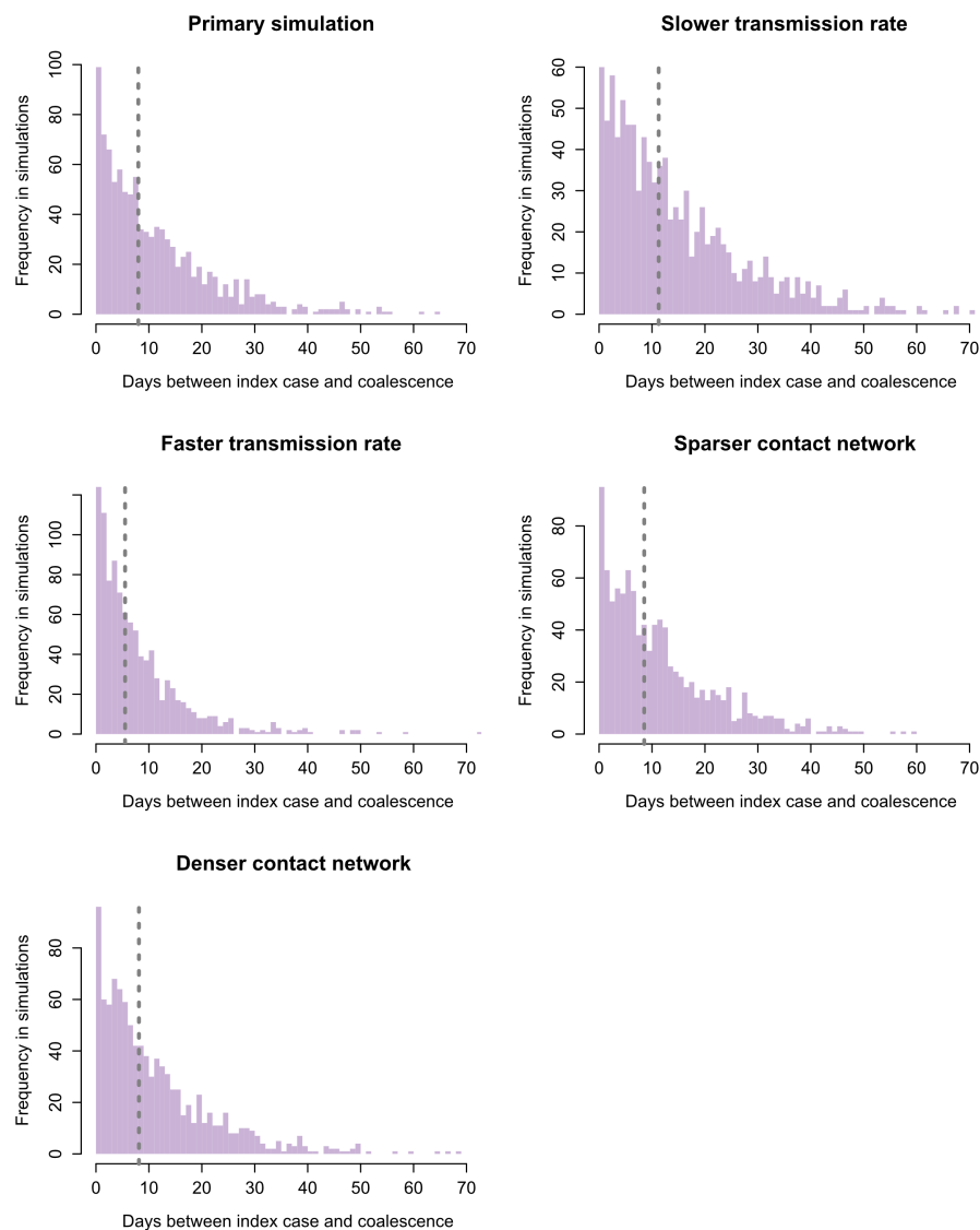
Figure A.4. FAVITES robustness analyses. Number of days between the index case the coalescence when simulated transmission rate is slower and faster and when the contact network has fewer (mean=10) and more (mean=26) contacts.
