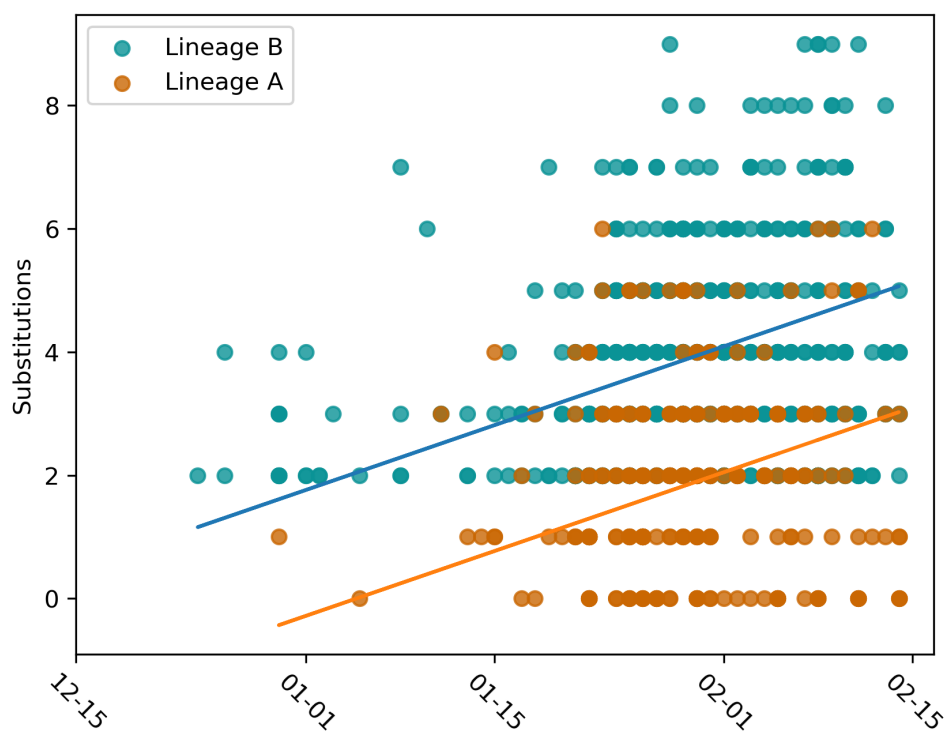
Figure B.20. Substitution counts of SARS-CoV-2 genomes through 14 February 2020 from the root of the maximum likelihood tree when rooted on lineage A (Fig. B.19). The plotted lines have a slope of 27.51 substitutions/year, are fit to their respective lineages, and are separated by 2.04 substitutions, showcasing the greater divergence of lineage B than lineage A when the tree is rooted on lineage A.
