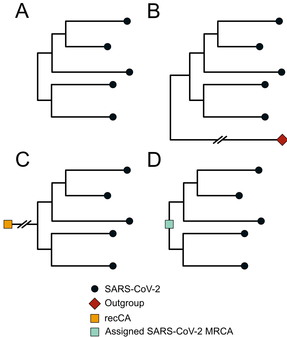
Figure B.18. Schematic depicting the rooting strategies used in different phylodynamic models. (A) An unconstrained rooting model with only SARS-CoV-2 where the root is inferred from the molecular clock calibrated using SARS-CoV-2 sampling dates. (B) An unconstrained rooting with SARS-CoV-2 and a sarbecovirus outgroup. (C) A constrained model where the ancestor of SARS-CoV-2 is constrained to be the recombinant common ancestor (recCA). (D) A constrained model with only SARS-CoV-2, but the MRCA forced to be a pre-specified haplotype.
