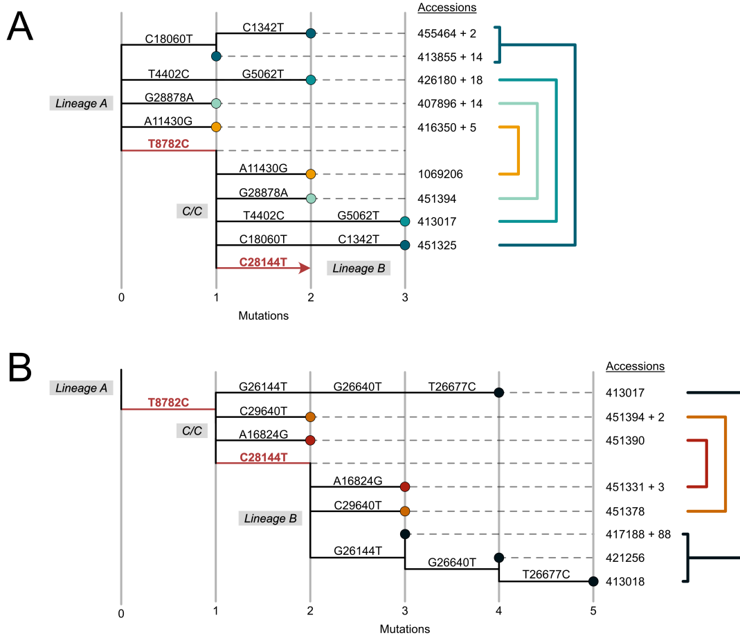
Figure B.1. Mutation map of SARS-CoV-2 intermediate C/C genomes and their shared mutations within lineages A and B. (A) Shared mutations across lineage A and C/C. (B) Shared mutations across lineage B and C/C. Mutations relative to the Hu-1 reference genome are shown above each branch. Lineage-defining mutations (8782 and 28144) are colored in red. Derived mutations not shared by both lineages are excluded. The taxon names are GISAID accession numbers, and the total number of additional matching homoplastic sequences are indicated. Sequences that share derived mutations are connected by the lines on the right, and brackets indicate that a group of sequences share the derived mutations that cannot be individually resolved.
