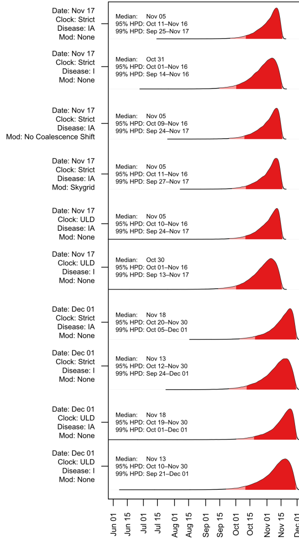
Figure A.10. Robustness analysis for timing of SARS-CoV-2 index case in Hubei province in the two-phase epidemic simulations. Primary two-phase analysis (from Fig. 1.3H) is shown on top. Dates indicates the minimum bound for rejection sampling (Nov 17 or Dec 01). Clock indicates whether the tMRCA was inferred using a strict or relaxed (ULD) clock. Disease denotes which stage of infection in the SAPHIRE model (IA, Ascertained or Unascertained; or I, Ascertained only) must have been reached by the given date for rejection sampling. 'Mod' denotes if any robustness modifications were explored. The 95% HPD is shown in dark red, and the 99% HPD is shown in light red.
