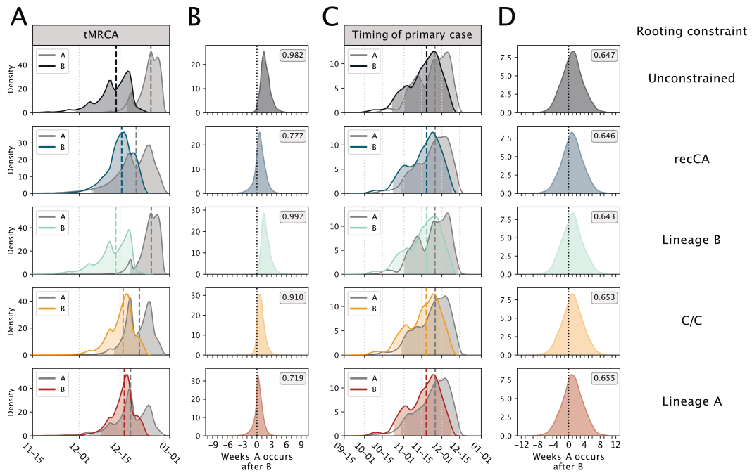
Figure 2.3. Comparison of the tMRCA and primary case dates for lineage A and lineage B across rooting strategies. Each row represents a different rooting constraint in phylodynamic analysis, with the bottom three representing a fixed ancestral haplotype. (A) The tMRCA for lineages A and B. (B) The number of weeks the tMRCA of lineage A occurs after the tMRCA of lineage B. (C) The timing of the primary case for lineages A and B. (D) The number of weeks the time of the primary case of lineage A occurs after the time of the primary case of lineage B. Long dashed lines indicate the median and shading represents the 95% HPD for each distribution. Short dashed lines indicate 0 weeks difference between lineages A and B. Posterior probability that lineage A originated after lineage B is reported in the grey box.
