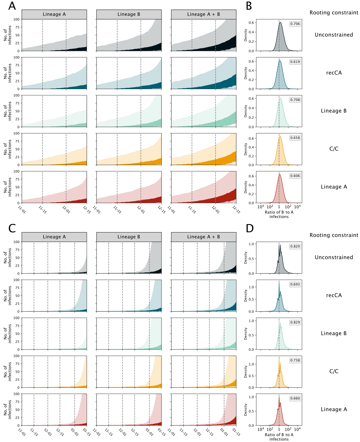
Figure B.28. Dynamics of SARS-CoV-2 resulting from separate introductions of lineages A and B and a longer doubling time. The simulations used here have a doubling time of 4.45 days (95%: HDI: 1.50-7.44). Each row represents a different phylodynamic analysis, with the bottom three representing an enforced ancestral haplotype. (A) Estimated number of infections. The header of each column indicates whether the infections are caused by lineage A, lineage B, or the two lineages combined. Darker and lighter shading represent the 50% and 95% HPD, respectively. (B) The log ratio of lineage B to lineage A infections on 15 December 2019. (C) Estimated number of hospitalizations, with column headers and shading identical to (A). (D) The log ratio of lineage B to lineage A hospitalizations on 1 January 2020. The proportion of the posterior with more lineage B infections or hospitalizations than lineage A in (B, D) is reported in the grey box.
