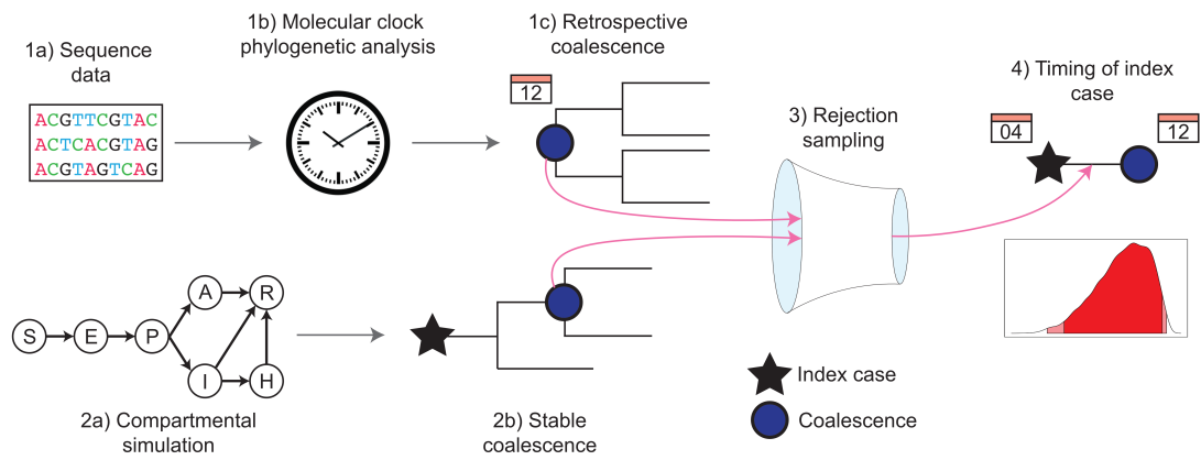
Figure A.5. Combined simulation and phylogenetic workflows to estimate the timing of the Hubei index case in a one-phase epidemic. (1a) Using sequence and epidemiological data, (1b) BEAST performs a phylodynamic molecular clock analysis to (1c) determine the tMRCA. (2a) FAVITES simulates the epidemic in Hubei using a SAPHIRE compartmental model (22) and (2b) estimates a prior distribution for the time from index case to the stable coalescence. The results of (1) and (2) are combined via rejection sampling (3; Fig. A.6) to (4) determine the timing of the index case and its posterior distribution.
