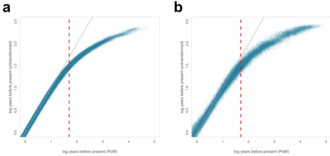
Figure C.7. Prisoner of War (PoW) transformation comparison. The log number of years of each internal node before the most recently sampled taxon compared to the log number of years of the same node after applying a PoW transformation for (a) 100 SARS-CoV-1-like posterior phylogenies for each NRR and (b) 100 SARS-CoV-2-like posterior phylogenies for each NRR. Red dashed line at 50 years before the most recently sampled taxon indicates a threshold beyond which saturation effects substantially influence tMRCA estimates. Diagonal dotted line depicts a line of equality, with a one-to-one correspondence between the two inferences on the two axes.
