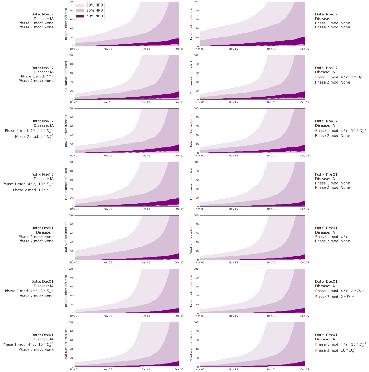
Figure A.12. Robustness analysis for the number of people infected SARS-CoV-2 based on the SAPHIRE model in late 2019 using two-phase simulations. Innermost shading is 50% HPD, middle shading is 95% HPD, and outer shading is 99% HPD. Dates indicates the minimum bound for rejection sampling (Nov 17 or Dec 01). Clock indicates whether the tMRCA was inferred using a strict or relaxed (ULD) clock. Disease denotes which stage of infection in the SAPHIRE model (IA, Ascertained or Unascertained; or I, Ascertained only) must have been reached by the given date for rejection sampling. D_h is the average time to hospitalization and r is the ascertainment rate, with the same values as in the primary analysis (Table A.1).
