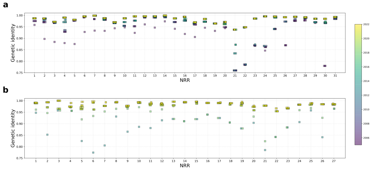
Figure C.6. Genetic similarity of the NRRs of the recCA to each SARS-CoV over time. a, The similarity of each NRR of the recCA of SARS-CoV-1 to SARS-CoV-1 as a function of time. b, The similarity of each NRR of the recCA of SARS-CoV-2 to SARS-CoV-2 as a function of time. Each square represents the similarity of the NRR of the recCA to its relative SARS-CoV at one point in time and is colored by date of the most recent non-human sarbecovirus in the reconstruction. See Fig. 3.2 for the similarity of the complete recCA of each SARS-CoV to its relative SARS-CoV over time.
