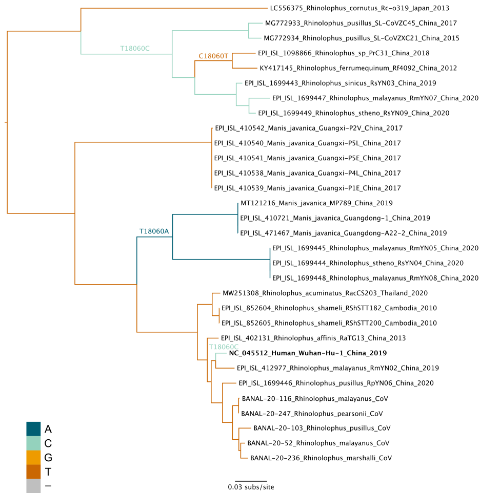
Figure B.12. Maximum likelihood tree of non-recombinant region 8 with branches colored based on the nucleotide at position 18060.
