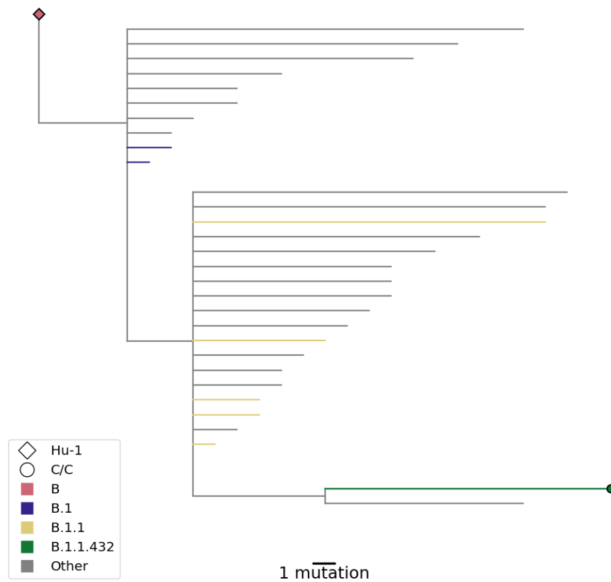
Figure B.5. Subtree showing the placement of C/C genome in the San Diego SEARCH dataset. 1 C/C genome was placed on a global tree of 3 million genomes (v2022-01-21) using UShER. The node branches are colored by the assigned PANGO lineage. The C/C genome is highlighted using a circle.
