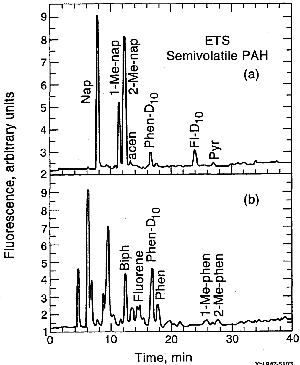
Figure 5. Dual-detector chromatograms of a silica-cleaned cyclohexane extract of the gas-phase semivolatile PAH collected from 0.7 m 3 simulated ETS on an XAD-4 sorbent bed. The timetable for excitation and emission wavelength changes is given in the text. Abbreviations are Nap, naphthalene; 1-Me-nap, 1-methylnaphthalene; 2-Me-nap, 2-methylnaphthalene; acen, acenaphthene and acenaphthylene; Biph, biphenyl; Phen-D 10 , deuterated phenanthrene; 1-Me-phen, 1-methylphenanthrene; and 2-Me-phen, 2-methylphenanthrene. Other abbreviations are listed in the caption for Fig 3.
