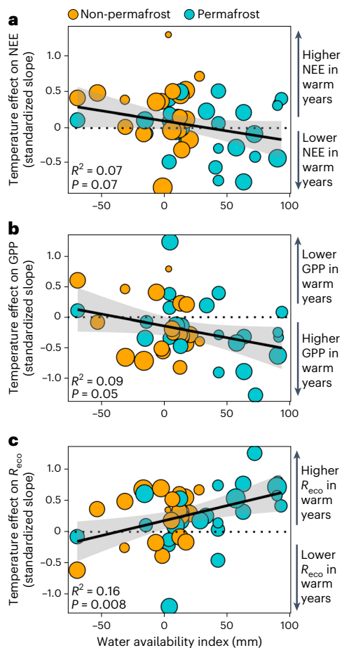
Fig. 6 | Effects of summer water use on summer \text{CO}_2 flux response to air temperature. a–c. Lines reflect linear regressions of the effects of summer water availability (x axis, 30 year mean \text{AET}_{\text{summer}} minus 30-year \text{MAP}_{\text{summer}} ) on the relationship between summer air temperature and NEE ( a ), GPP ( b ) and R_{\text{eco}} ( c ). Standardized slopes reflect the effect of 1 s.d. (z-score) of summer temperature on 1 s.d. of summer C flux. Positive x-axis values indicate sites where summer water use regularly exceeds precipitation inputs and near-surface soil water may be especially important. Points above the dashed zero line on the y axis represent sites where higher-than-average summer temperatures lead to higher-than-average NEE ( a ) and R_{\text{eco}} ( c ), or lower-than-average GPP ( b ). Larger points indicate greater confidence in the slope for each site and reflect model weights. Error bands represent 95% confidence intervals.
