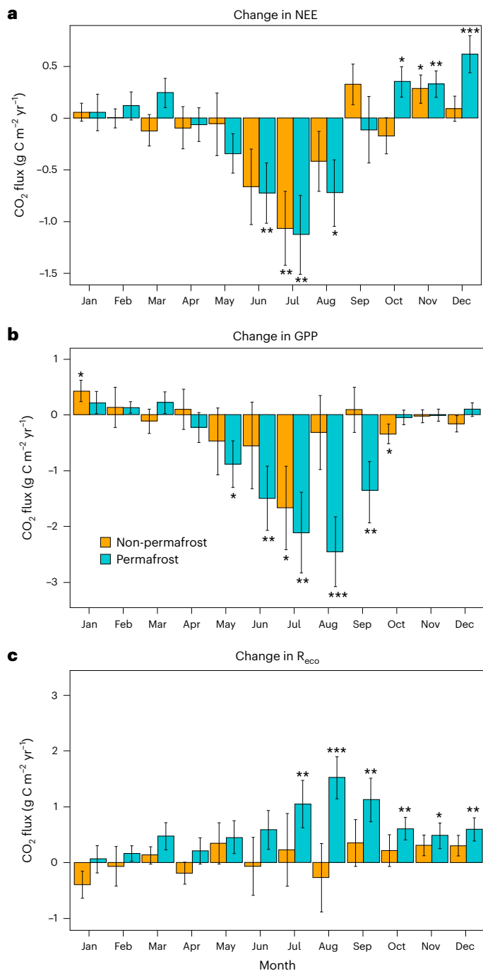
Fig. 4 | Decadal changes in NEE, GPP and R_{\text{eco}} by month. a–c. The monthly \text{CO}_2 flux changes in NEE (a), GPP (b) and R_{\text{eco}} (c) are shown. The y axis reflects the slope of change over time based on linear mixed-effects models with a random effect for site. Positive slope values indicate increasing NEE over time (decreasing net \text{CO}_2 uptake) and negative slope values indicate decreasing NEE over time (increasing net \text{CO}_2 uptake). Negative GPP slopes represent increasing productivity ( \text{CO}_2 uptake), and positive R_{\text{eco}} slopes represent increasing respiratory losses to the atmosphere. Error bars reflect the s.e. for each slope. Asterisks denote statistical significance of the slopes not adjusted for multiple comparisons; * P \leq 0.05 , ** P \leq 0.01 , *** P \leq 0.001 . Model parameters can be found in Supplementary Table 6.
