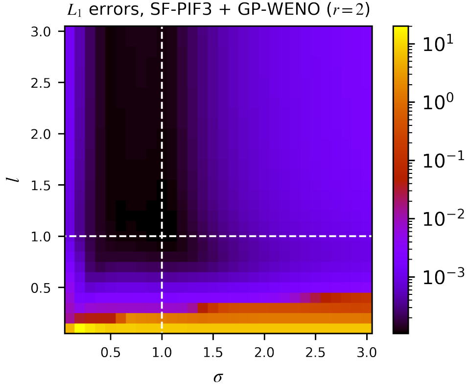
Figure 5.13: The L_1 errors of vortex advection problem in Section 5.1.2 solved by GP-WENO and SF-PIF3 on a 400 \times 400 grid resolution. The radius of GP-WENO stencil is r = 2 , which is the same stencil size of the fifth-order WENO method. Using other temporal solvers produces the same pattern, and omitted in this study. The white dotted-lines are represent the hyperparameters of minimum error.
