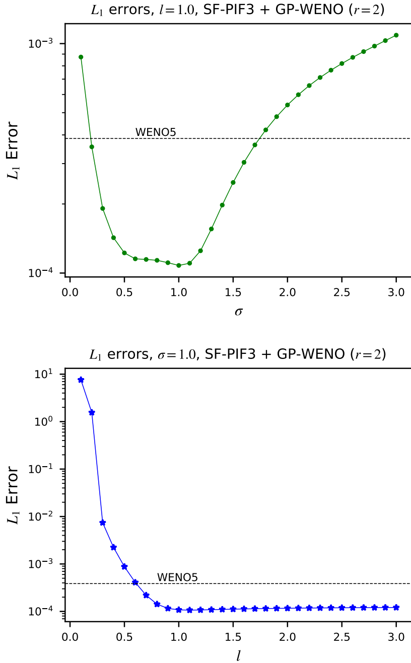
Figure 5.14: The slices of Fig. 5.13 at the minimum error. The horizontal dotted line is the target error obtained from WENO method with same configurations.
