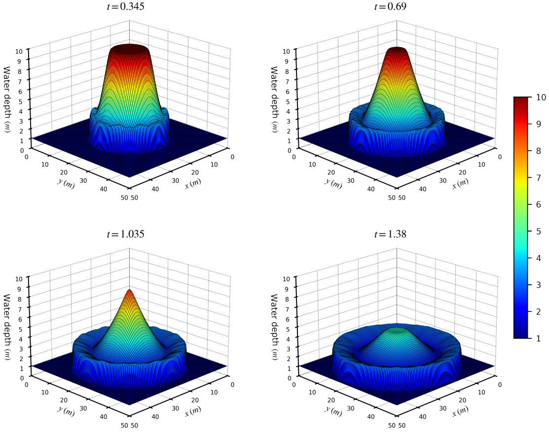
Figure 5.6: Snapshots of the circular dam breaking simulation at four different times, t = 0.345, 0.69, 1.035, and 1.38 seconds. A volume of water in rest is initially confined in a cylindrical dam of a radius r = 11 m and a height h = 10 m. The simulation starts with an instantaneous removal of the cylindrical wall located at the center of the domain [50 \text{ m} \times 50 \text{ m}] resolved on a grid resolution of 100 \times 100 . The gravitational force is exerted on the steady water, which triggers the onset of the gravitational collapse of the entire volume of water, making the circular splash in the outer rim as well as the ripple effects in the central region that move radially outward in time.
