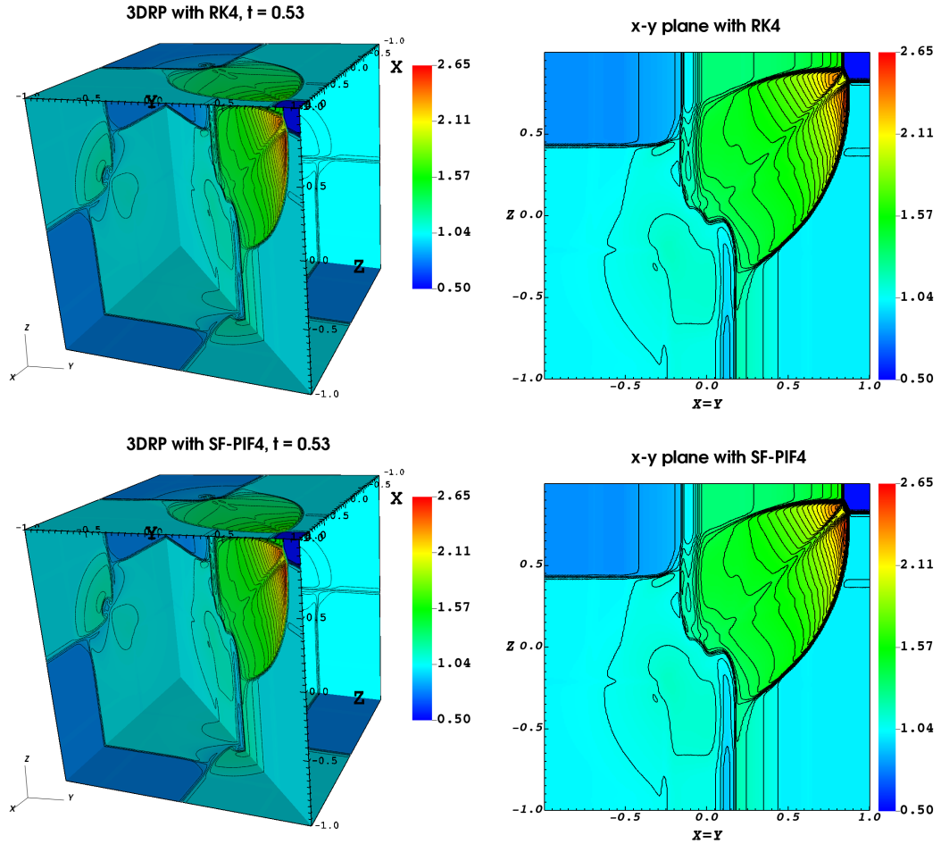
Figure 5.12: The density maps of the 3D Riemann problem test at t = 0.53 . Forty contour lines are over-plotted. The left panels show each face's geometrical views, while the right panels show the detailed picture of the diagonal planes. All simulations are performed on a 256 \times 256 \times 256 grid resolution, solved with RK4 ( top ) and SF-PIF4 ( bottom ) solvers. The Courant condition, C_{\text{cfl}} = 0.3 is used for calculating the timestep.
