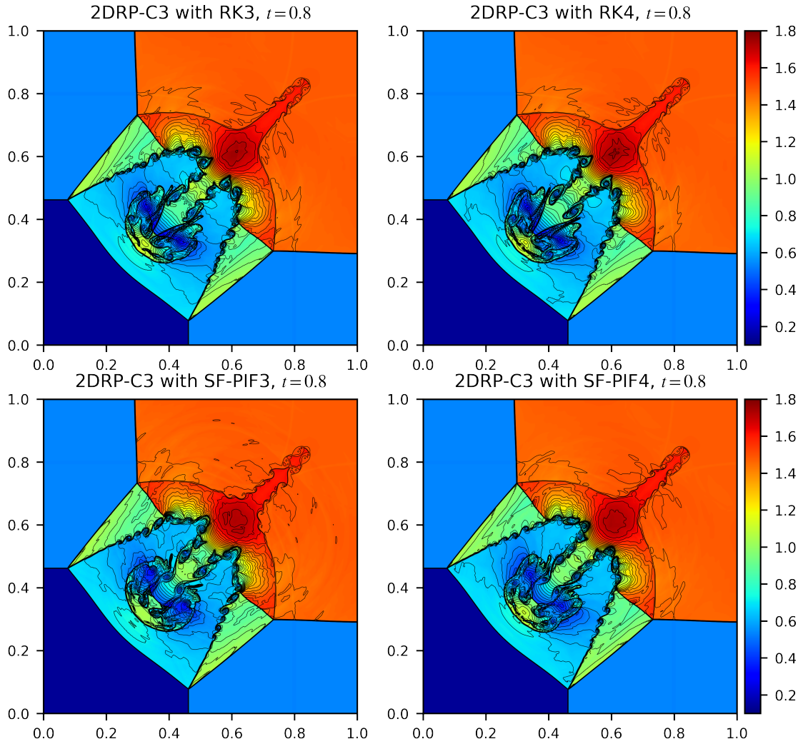
Figure 5.9: The density maps of Configuration 3 at t = 0.8 . Left column: The solutions using RK3 (top) and SF-PIF3 (bottom). Right column: The solutions using RK4 (top) and SF-PIF4 (bottom). Forty levels of black contour lines are over-plotted in each figure with the same range of the color map. All simulations are performed on a 1600 \times 1600 grid resolution.
