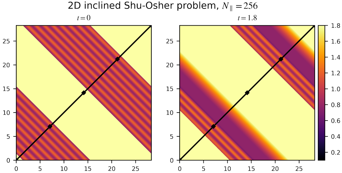
Figure 5.7: 2D density maps of inclined 2D Shu-Osher test problem at t = 0 and t = 1.8 . The test was performed on a 2D simulation box of 1024 \times 1024 resolution with the SF-PIF4 method. The solid black line represents the shock propagating direction, x_{\parallel} , and square markers divide the line in each quartile.
