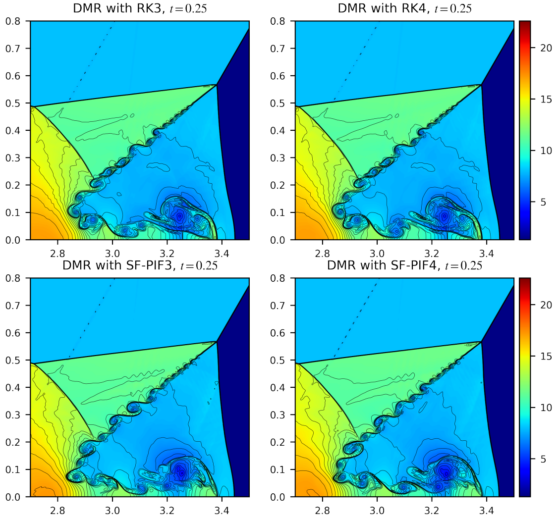
Figure 5.11: The density map of the double Mach reflection test at t = 0.25 zoomed-in near the jet. Forty levels of contour lines are over-plotted in solid black curves with the same range of the color map. All simulation results are performed on a 4096 \times 2048 grid resolution. Left column: The solutions using RK3 (top) and SF-PIF3 (bottom). Right column: The solutions using RK4 (top) and SF-PIF4 (bottom).
