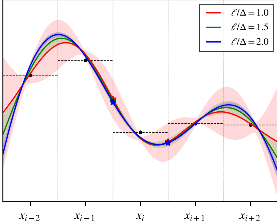
Figure 3.3: GP reconstructed profiles with the same data as Figs. 3.1 and 3.2 with different hyperparameters \ell/\Delta = 1.0, 1.5, 2.0 . The radius of GP stencil is r = 2 . Note that all the reconstructed profiles produce a new local minimum near x = x_{i+\frac{1}{2}} , which violates the monotonic-preserving condition and leads to numerical oscillations. The shaded areas represent 95% confidence regions from the posterior variance.
