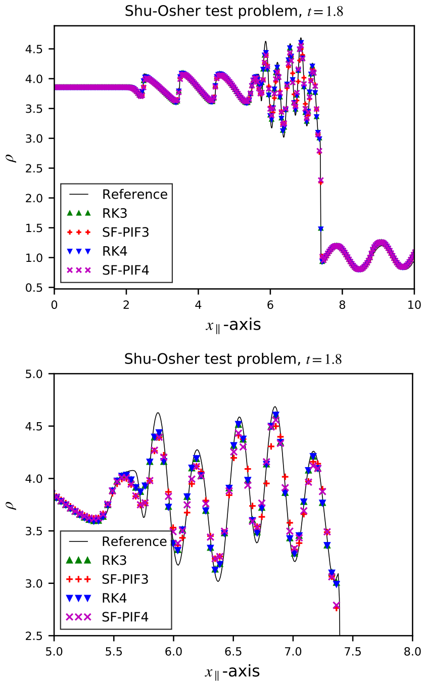
Figure 5.8: One dimensional density profiles along the x_{\parallel} direction of the inclined Shu-Osher problem at t = 1.8 . The solid line represents the reference solution, solved by RK4 with 1024 data points in the diagonal axis, i.e., N_{\parallel} = 1024 . All other solutions, represented by the symbols, are resolved on an N_{\parallel} = 256 grid resolution in the diagonal axis. The detailed view of the high-frequency region is shown on the right panel.
