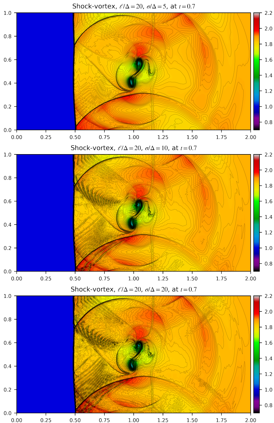
Figure 5.16: The density colormaps of the strong shock vortex interaction problem. The GP-WENO ( r = 2 ) + SF-PIF3 method are used for all simulation runs on [1024 \times 512] grid resolution with varying hyperparameter, \sigma/\Delta . The pseudocolors represent the density map ranging between [0.75, 2.2] , and 200 contour lines within the same range are over-plotted as solid black lines.
