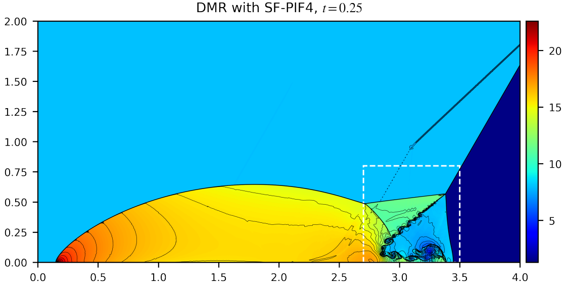
Figure 5.10: The solution density profile of Double Mach reflection test solved with SF-PIF4 method on a 4096 \times 2048 grid resolution. The solid black curves represent the forty levels of contour lines ranging within the same range of the colormap. The white-dotted rectangle is the main point of interest in this simulation, where the jet and the primary triple point are formed. More detailed view of the rectangle region with different temporal solvers are plotted in Fig. 5.11.
