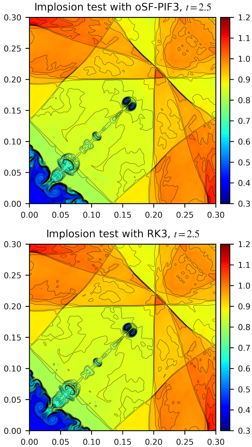
Figure 5.5: The density profile of the implosion test with oSF-PIF3 ( top ) and with RK3 ( bottom ) resolved on 400 \times 400 grid resolution. The color map ranges from 0.3 to 1.2, and 40 evenly-spaced contour lines are over-plotted with the same range.
