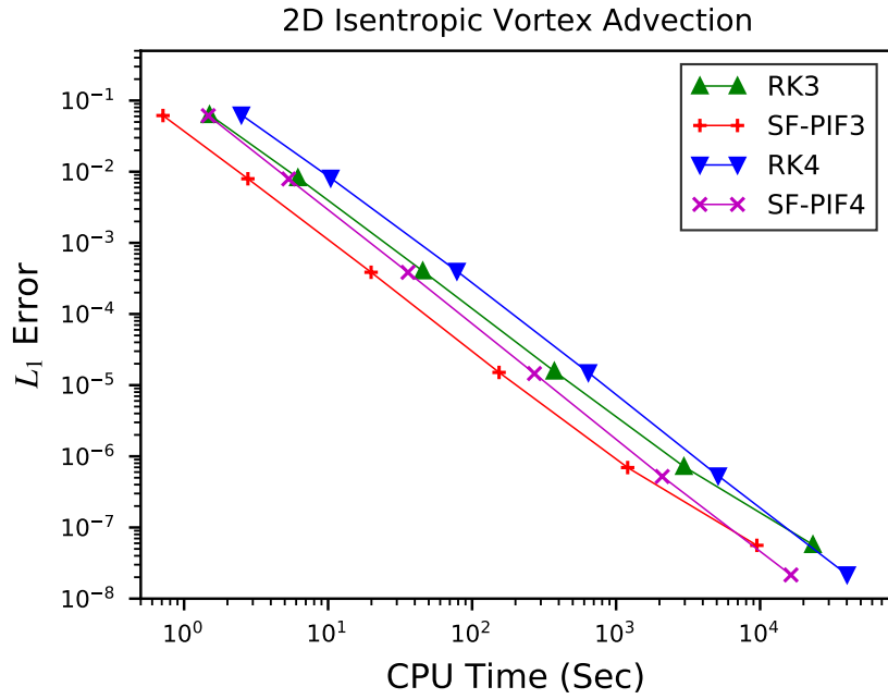
Figure 5.3: The L_1 errors of the isentropic vortex advection test problem solved by third- and fourth-order temporal schemes combined with WENO5 spatial method. The L_1 errors with respect to the grid resolutions ( top ); with respect to the computation time ( bottom ).
