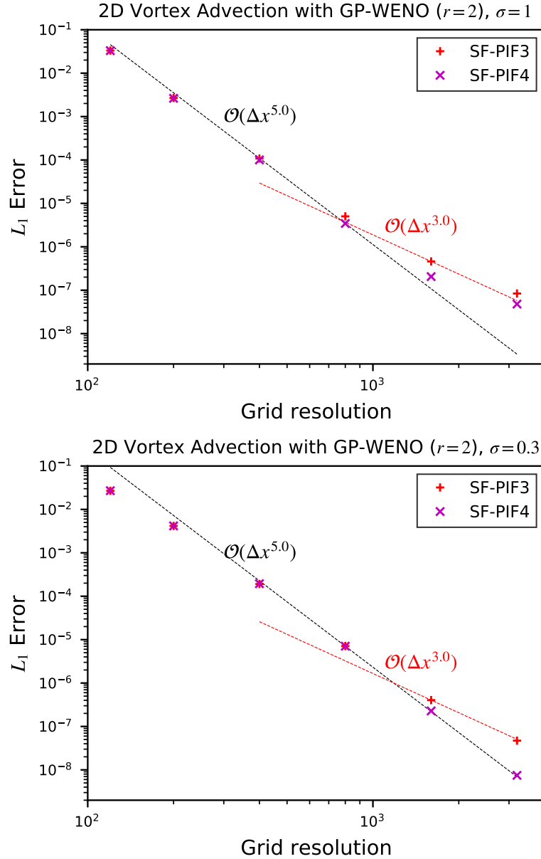
Figure 5.15: The convergence rate of GP-WENO method with r = 2 obtained by solving 2D isentropic vortex advection problem on varying grid resolutions. Two temporal methods, SF-PIF3 and SF-PIF4 are used for integrating the solution, and the behavior of third-order and fourth-order temporal schemes is identical to the results from Section 5.1.2. The GP length hyperparameters, \ell = 1 is used for both tests, and the shock-capturing hyperparameter top: \sigma = 1 , and bottom: \sigma = 0.3 are used. The tests with \sigma = 1 on the top panel have smaller absolute L_1 error, but failed to maintaining the convergence rate on high-resolution grids. On the other hand, tests with \sigma = 0.3 demonstrate consistent convergence rate on all grid configurations.
