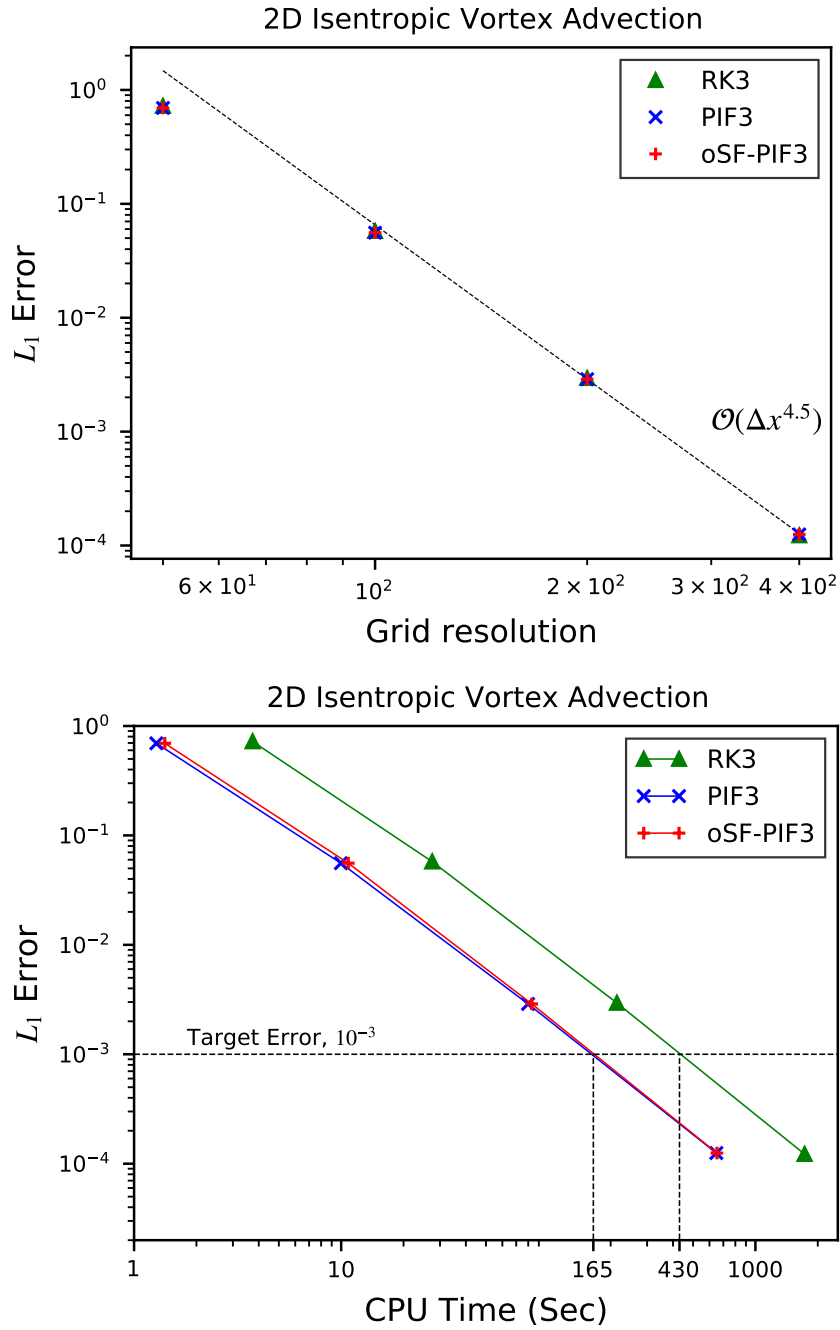
Figure 5.2: The L_1 errors of the isentropic vortex advection test problem on different grid resolutions, N_x = N_y = 50, 100, 200, and 400 . The three different third-order temporal schemes are used combined with WENO5 spatial method. The L_1 errors with respect to the grid resolutions ( top ); with respect to the computation time ( bottom ).
