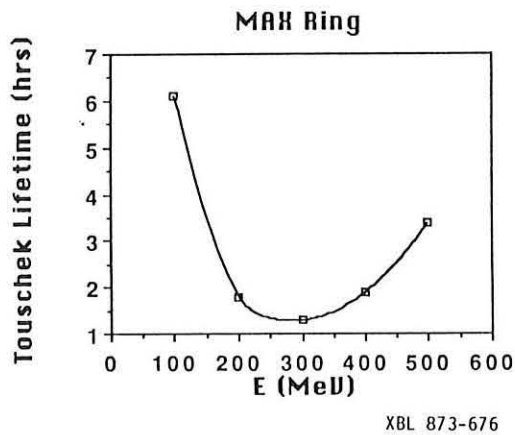
Fig. 7 Touschek lifetime for MAX ring at a beam current of 50 mA and 10% emittance coupling.
