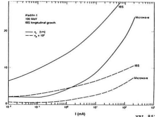
Fig. 4 Equilibrium bunch length and momentum spread as a function of beam intensity.
