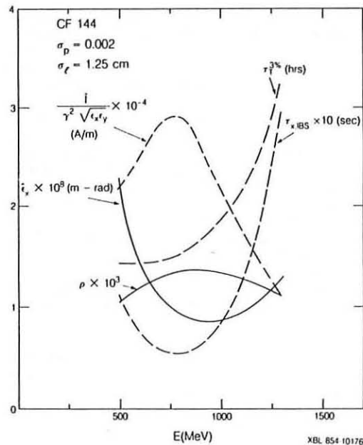
Fig. 3 Energy dependence of the following parameters: Touschek lifetime for 3% RF bucket height, \tau_T^{3\%} ; intrabeam scattering lifetime \tau_x ; equilibrium emittance \epsilon_x ; bunch volume density I/\gamma \sqrt{\epsilon_x \epsilon_y} ; FEL parameter \rho .
