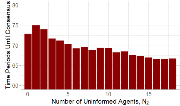
Figure 6: Controlling for initial bias strength, increasing the number of uninformed individuals added to a group of 12 polarized informed agents decreased the time needed for the group to reach consensus (among trials where consensus was reached in less than 200 time periods).
