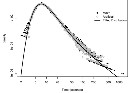
Figure 2: Histograms (in log-log scale) of the RLs in the Maze dataset (black solid dots) and of the simulated artificial dataset (grey open circles). The solid black line plots the fit to the data of the distribution from which the simulated points were sampled.
