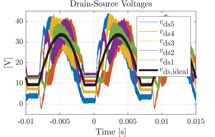
Fig. 6: Measured switch drain-source voltage stress for the operating conditions described in Section III. Ideally the peak switch drain-source voltage is V_{in}/(N-1) which is achieved when all flying capacitor voltages are at the balanced distribution. The peak drain to source voltage in this experiment was 44.5 V which is 31% higher than the ideal voltage.
