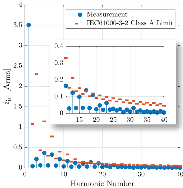
Fig. 7: Measured input current harmonics reported by the Keysight Power Analyzer PA2201A. At an output power of 432 W, all harmonics pass except for the 17th harmonic (1.02 kHz) which is 4% over the limit. Note that the IEC61000-3-2 limits are strictly applicable only for equipment operated at an input voltage above 230 V ac however the comparison is reported here to convey the magnitude of the harmonics relative to industry standards.
