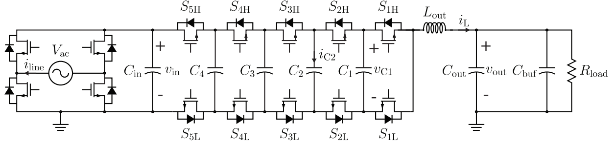
Fig. 1: Circuit diagram of an ac-dc PFC rectifier utilizing a six-level FCML converter with an input synchronous rectifier. C_{in} serves to buffer switching frequency ripple while C_{buf} performs twice-line frequency power buffering.
