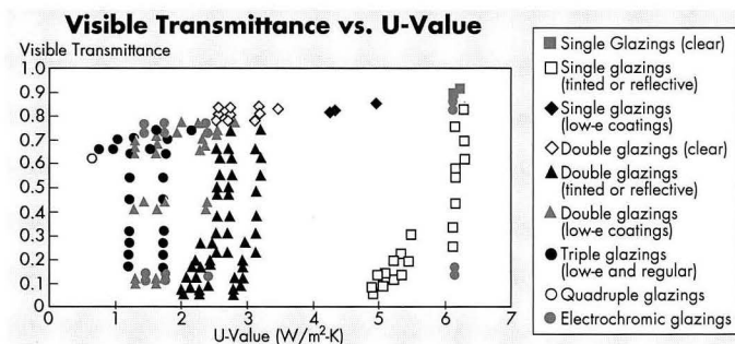
Figures 2a and 2b. Over a range of thermal efficiencies, (U-Value), windows vary considerably in their spectral selectivity (above) and visible transmittance (below).
