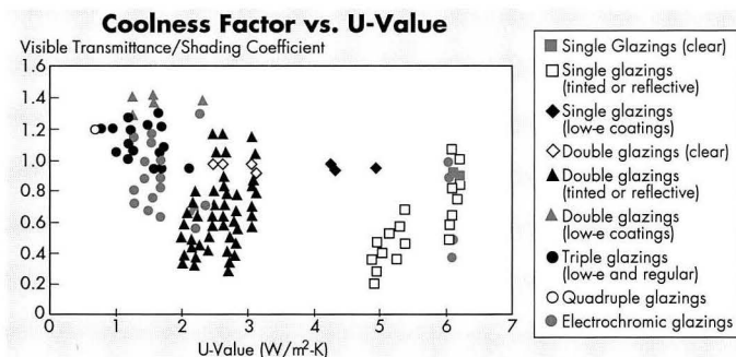
Figures 2a and 2b. Over a range of thermal efficiencies, (U-Value), windows vary considerably in their spectral selectivity (above) and visible transmittance (below).
