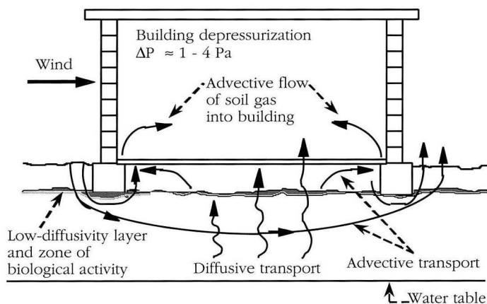
Schematic of soil-gas and contaminant transport into a slab-on-grade building at a former service station site. Three effects are illustrated that can contribute to reducing the amount of contaminant available for entry into the building: biodegradation by soil microorganisms; a layer of soil that limits diffusive movement of the contaminant; and wind-driven ventilation of the soil below the building. Not illustrated are the effects of ventilation on contaminant concentrations inside the building.
