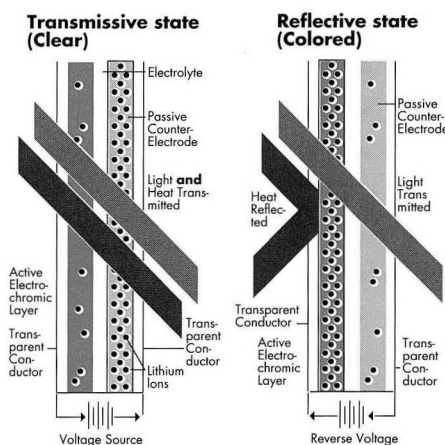
Figure 3. Cross section of prototype five-layer electrochromic coating in clear and colored states (layers not to scale).
