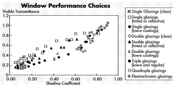
Figure 1. Variations in visible transmittance and shading coefficients for various glazing products. With the exception of electrochromics, the figure represents products available on the U.S. market in 1992. (From the Window Library in the DOE-2 building energy simulation program.) Note: The next revision to this database will report solar properties as Solar Heat Gain Coefficient, which is now gradually replacing Shading Coefficient in product literature as the key solar parameter.
