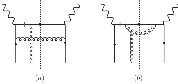
FIG. 1: The example diagrams for the soft pole (a) and hard pole (b) contributions to \Lambda transverse polarization in semi-inclusive DIS process. The short bars indicate the pole contribution from the propagators.
