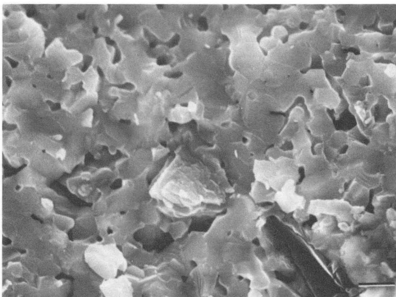
Doped matrix, 5 vol% SiC, heated to 1100 °C.
