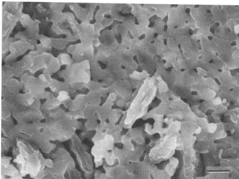
Doped matrix, 5 vol% SiC, sintered to 1100 °C.
