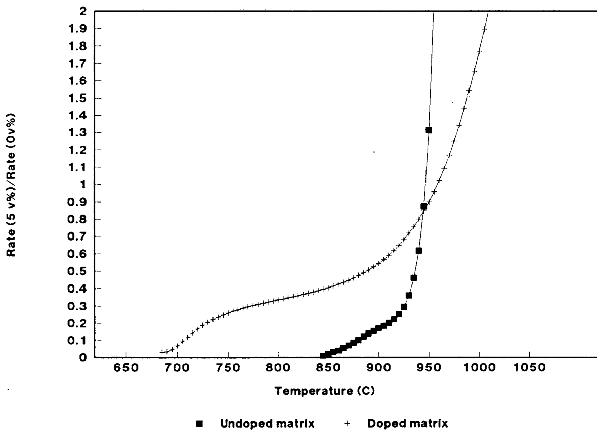
Figure 13: Normalized Densification Rate vs. Temperature
