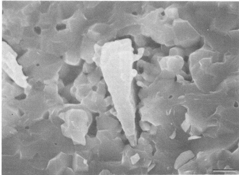
Undoped matrix, 1 vol% SiC, sintered to 1100 °C.
