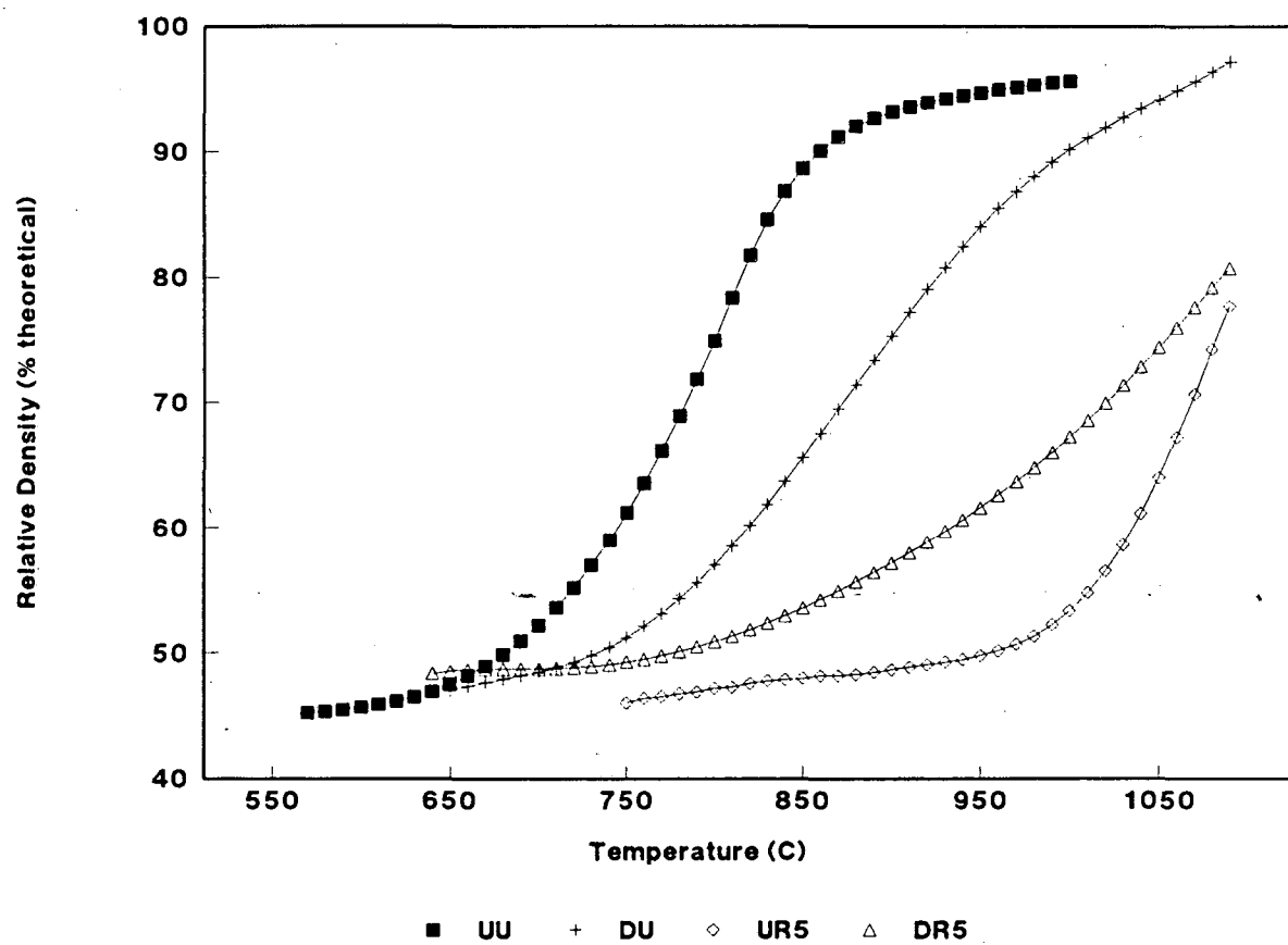
Figure 10: Density vs. Temperature
