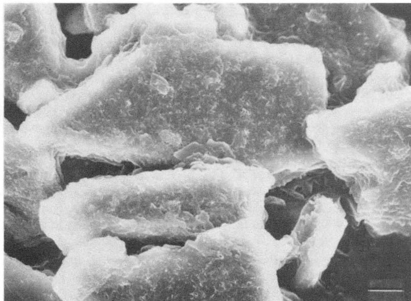
Figure 4(a): ZnO-SiC, from nitrate solution, after 15 minutes. Bar = 3.3 \mu\text{m} .
