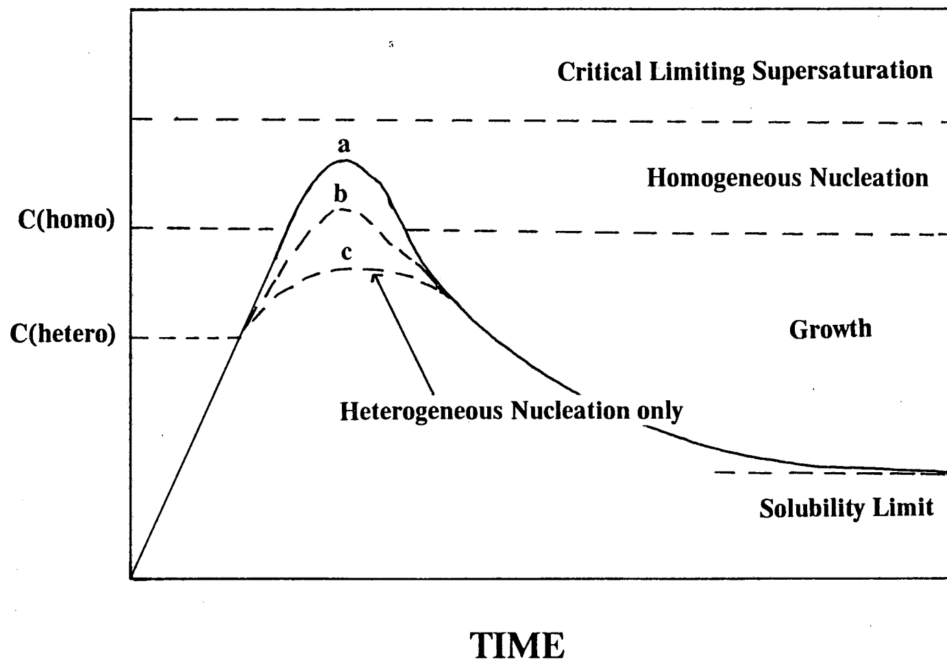
Figure 2: La Mer diagram [29].
