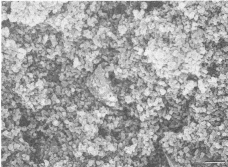
Doped matrix, 5 vol% SiC, heated to 700 °C.
