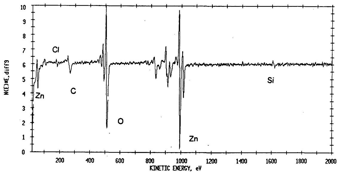
Figure 15: Auger Electron Spectrum of undoped ZnO-% vol% SiC composite
