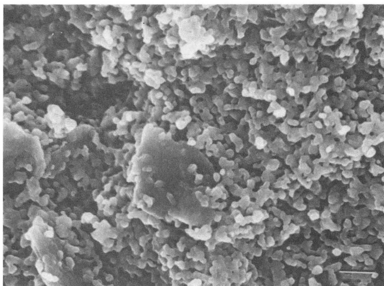
Doped matrix, 10 vol% SiC, sintered to 1100 °C.
