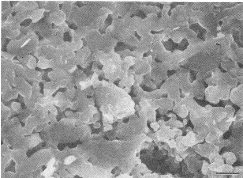
Doped matrix, 1 vol% SiC, sintered to 1100 °C.
