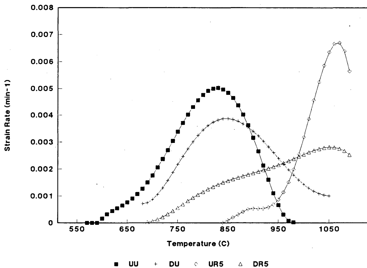
Figure 12: Densification Rate vs. Temperature
