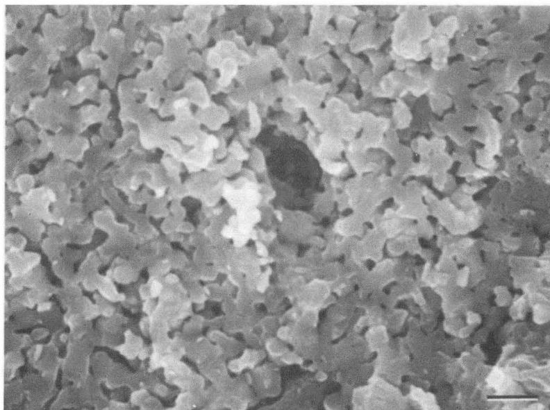
Undoped matrix, 5 vol% SiC, heated to 1100 °C.
