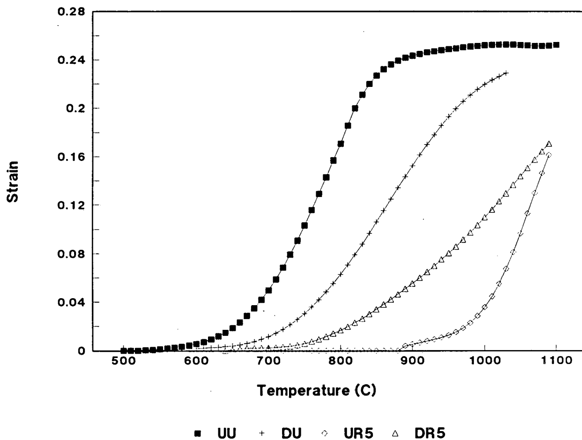
Figure 11: Densification Strain vs. Temperature
