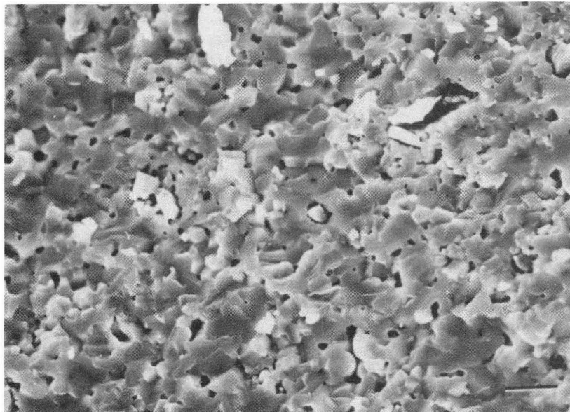
Figure 9(g): Undoped matrix, 1 vol% SiC, showing the formation of voids. Bar = 3.3 \mu\text{m} .
