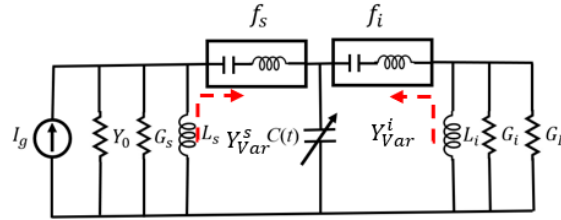
Figure 1.2: Simplified circuit model for parametric circuit.
